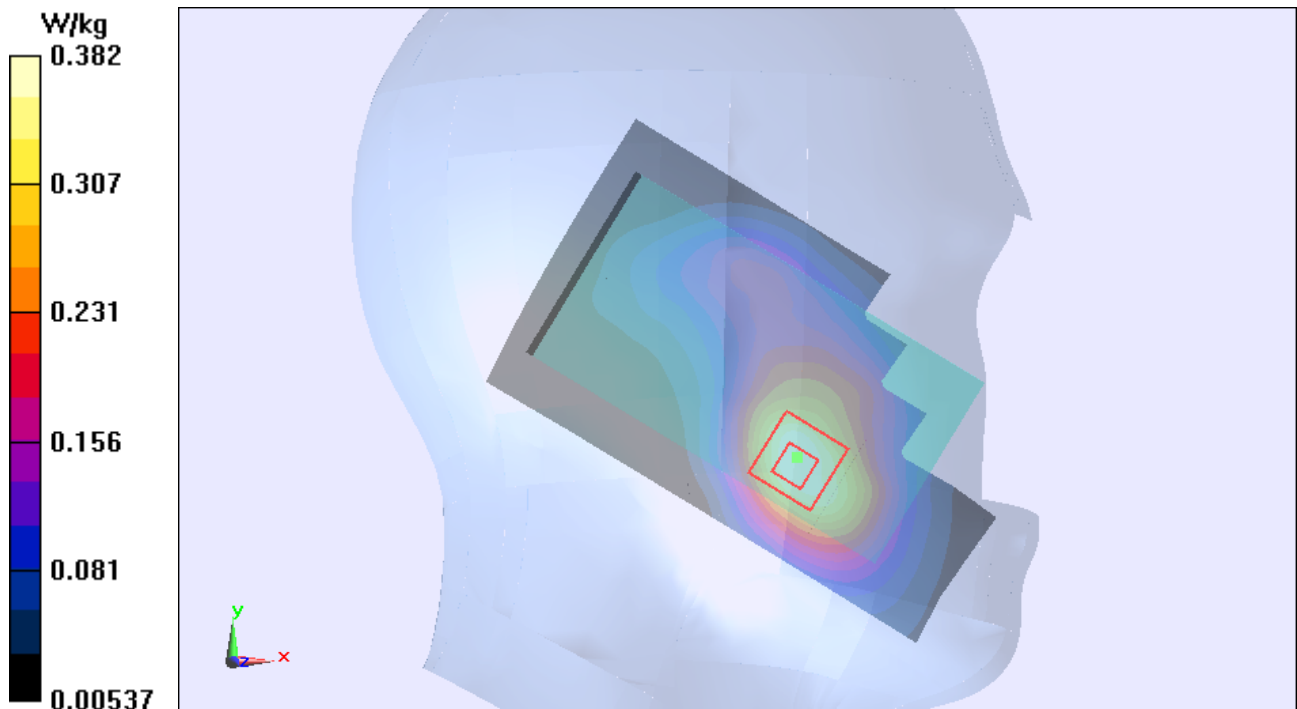
Figure 40 Left Hand Touch Cheek GSM 1900 Channel 661
