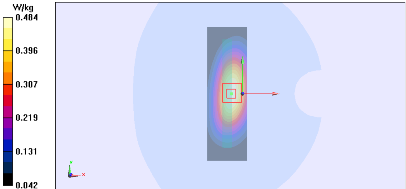
Figure 95 Body, Left Edge, UMTS Band V Channel 4183
