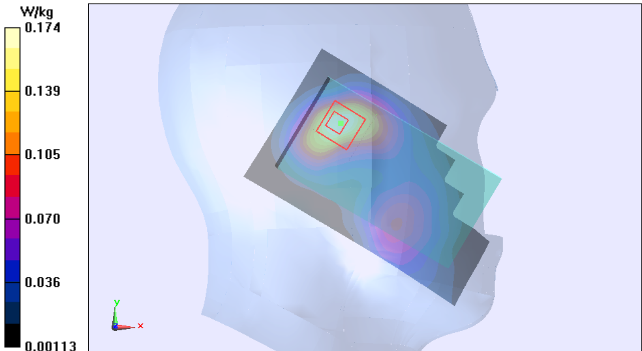
Figure 35 Left Hand Tilt 15° GSM 1900 Channel 661
