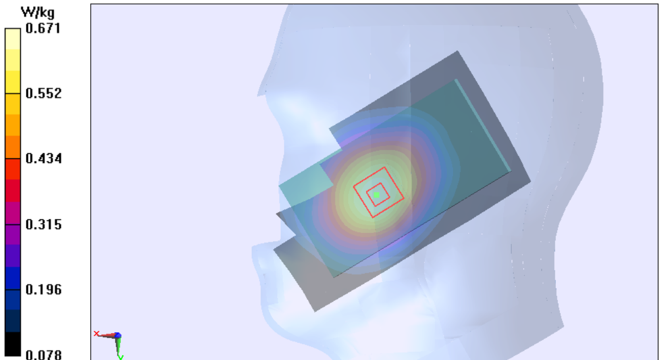
Figure 84 Right Hand Touch Cheek UMTS Band V Channel 4132
