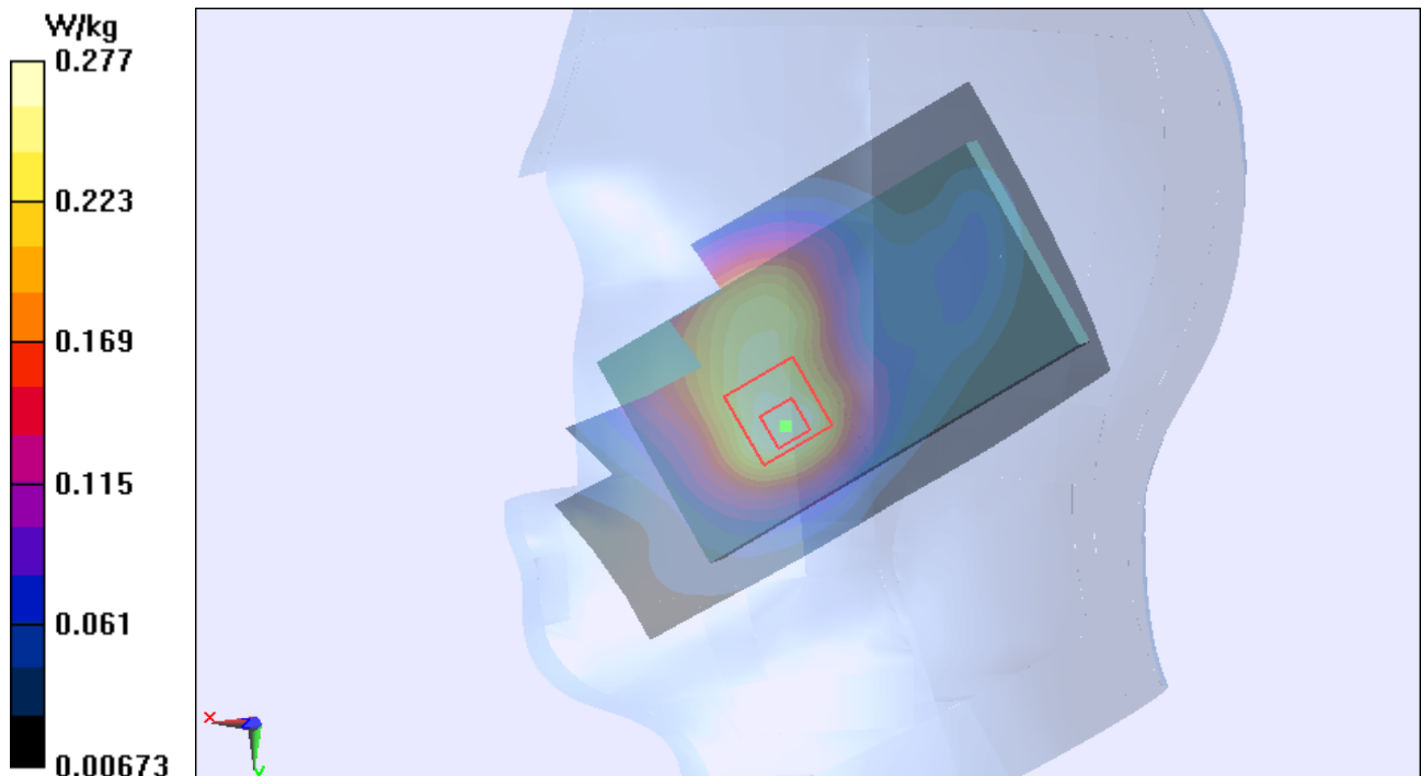
Figure 36 Right Hand Touch Cheek GSM 1900 Channel 661
