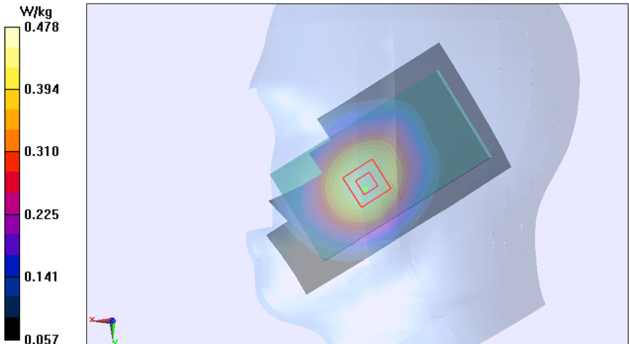
Figure 18 Right Touch Cheek GSM 850 Channel 190
