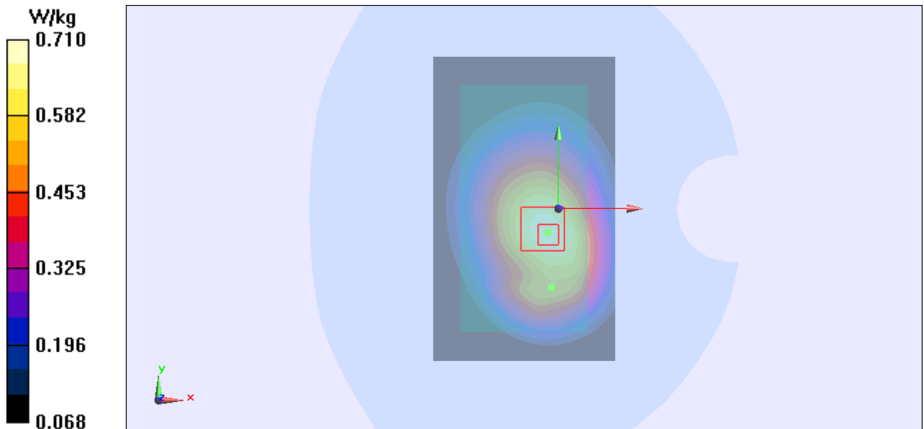
Figure 100 Body, Back Side, UMTS Band V Channel 4183
