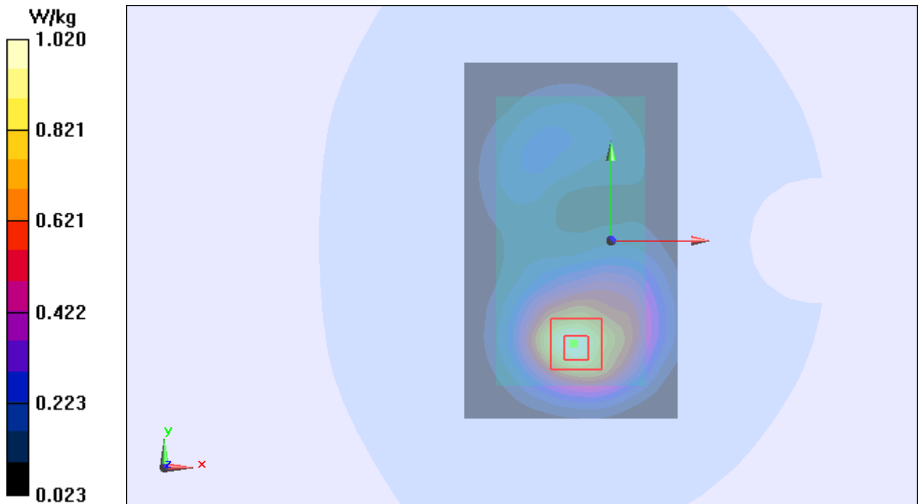
Figure 71 Body, Back Side, UMTS Band II Channel 9262
