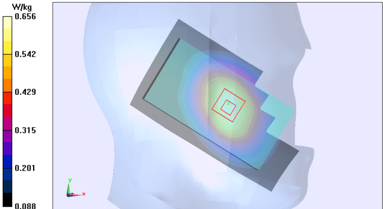
Figure 87 Left Touch Cheek UMTS Band V Channel 4183
