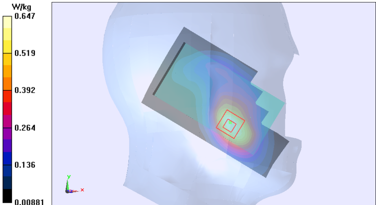
Figure 62 Left Hand Touch Cheek UMTS Band II Channel 9400
