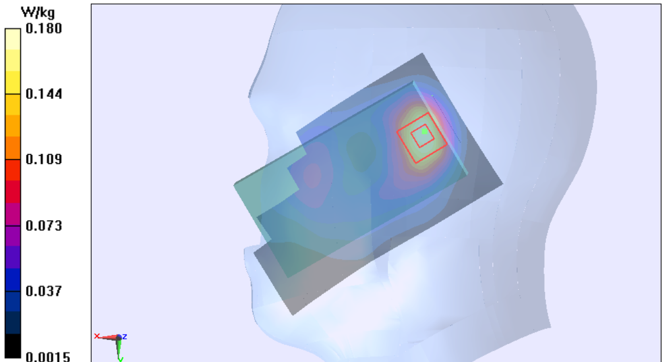
Figure 37 Right Hand Tilt 15° GSM 1900 Channel 661
