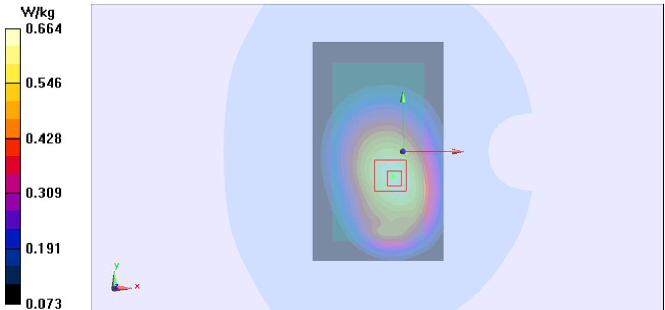
Figure 93 Body, Back Side, UMTS Band V Channel 4132
