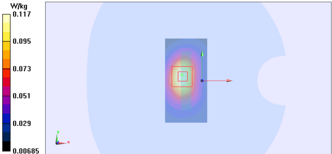
Figure 97 Body, Bottom Edge, UMTS Band V Channel 4183
