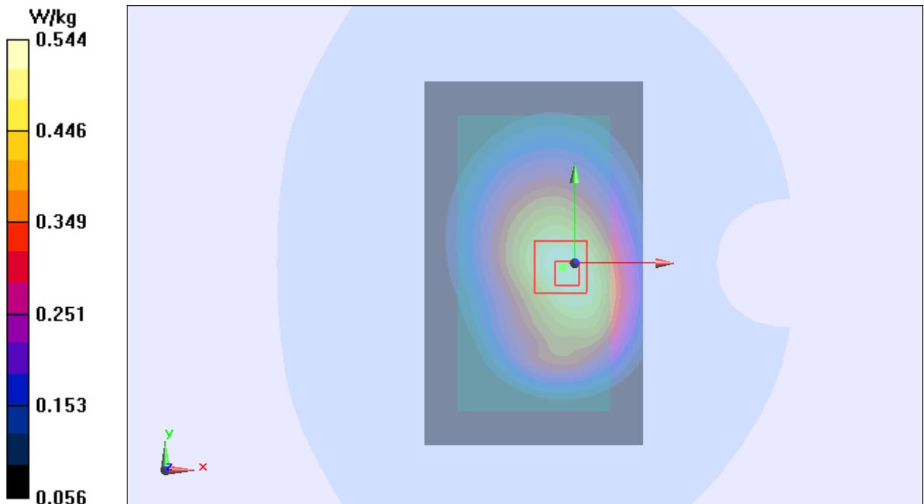
Figure 29 Body, Back Side, GSM 850 GPRS (2Txslots) Channel 190
