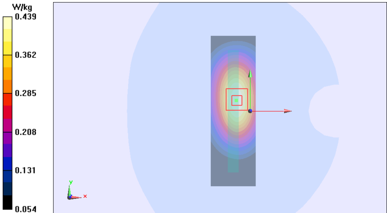
Figure 26 Body, Right Edge, GSM 850 GPRS (2Txslots)Channel 190
