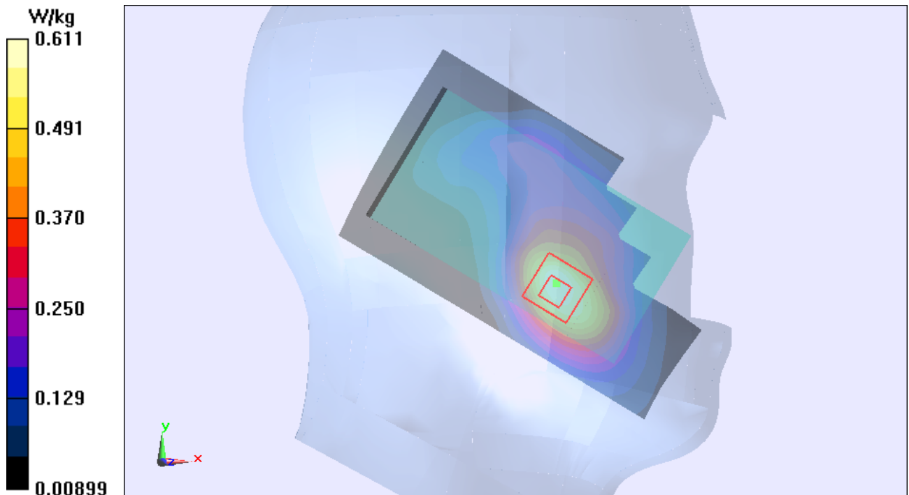
Figure 63 Left Hand Touch Cheek UMTS Band II Channel 9400
