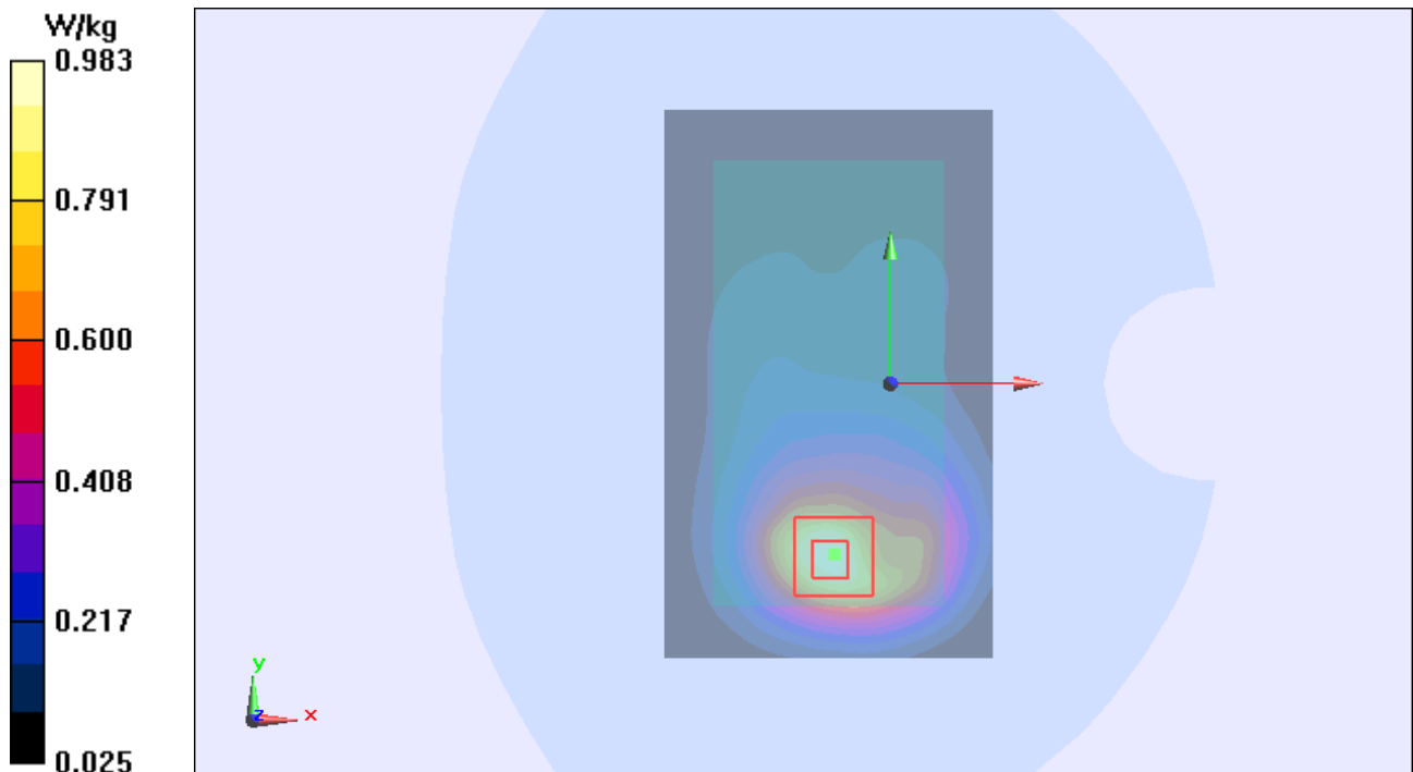
Figure 76 Body, Back Side, UMTS Band II Channel 9262
