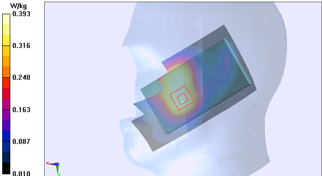
Figure 57 Right Hand Touch Cheek UMTS Band II Channel 9400
