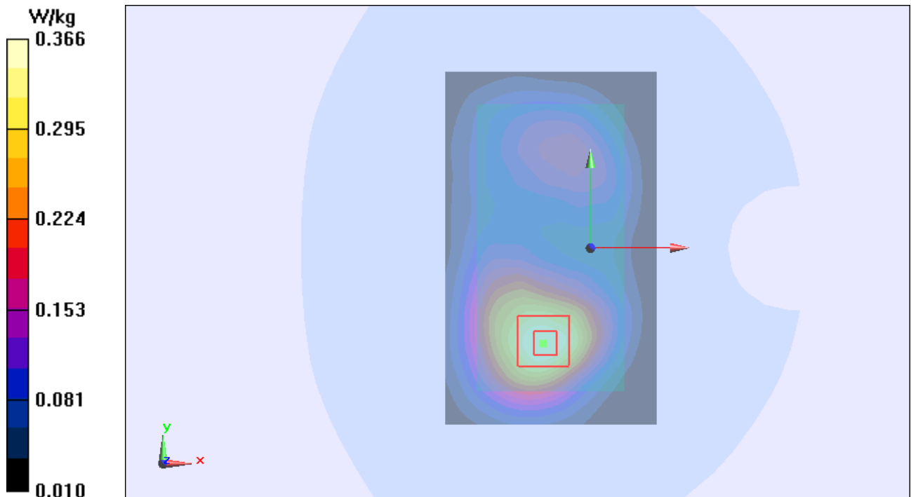
Figure 45 Body, Front Side, GSM 1900 GPRS (2Txslots) Channel 661
