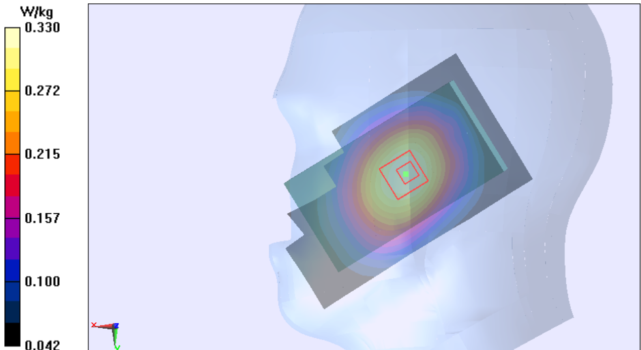
Figure 16 Right Hand Tilt 15° GSM 850 Channel 190
