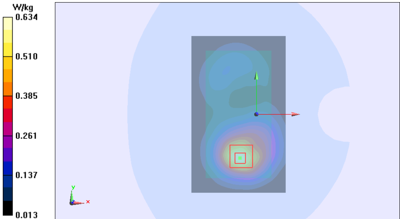
Figure 50 Body, Back Side, GSM 1900 GPRS (2Txslots) Channel 661
