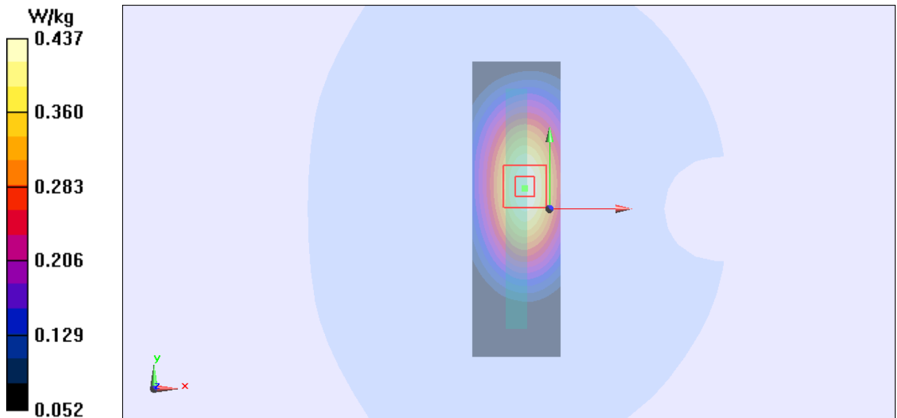
Figure 96 Body, Right Edge, UMTS Band V Channel 4183
