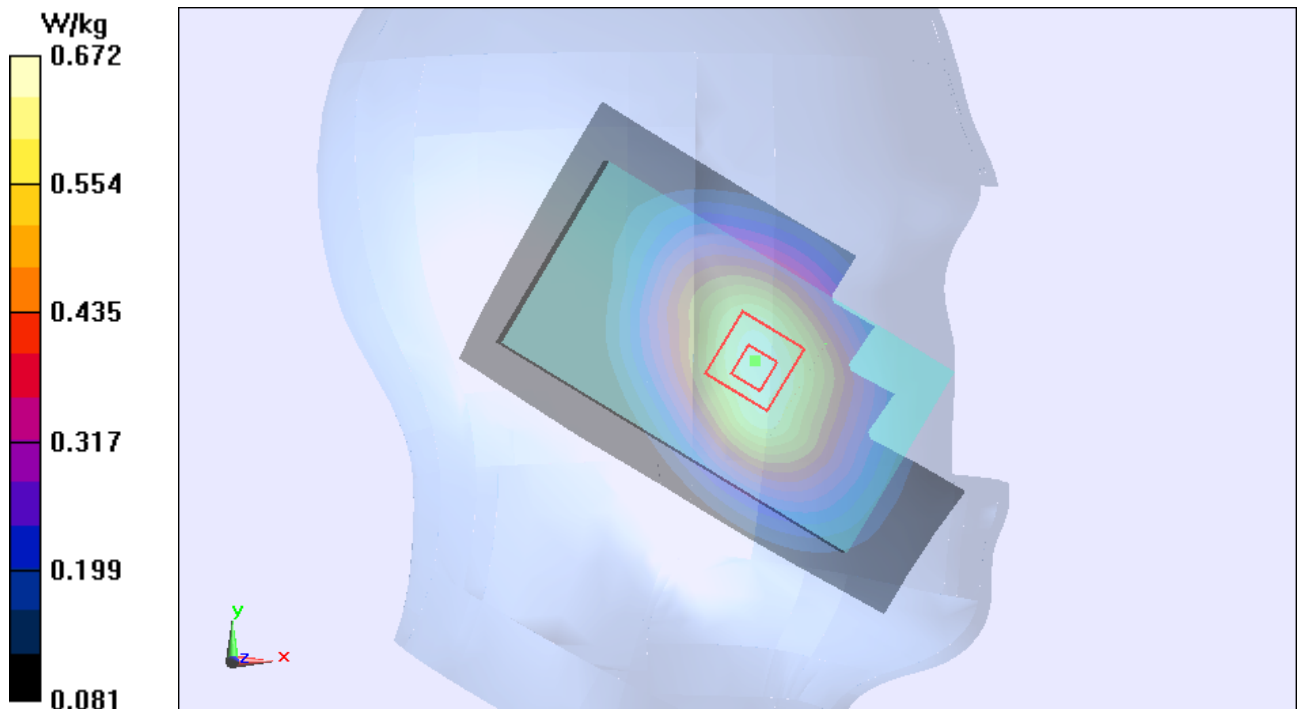
Figure 90 Left Touch Cheek UMTS Band V Channel 4183
