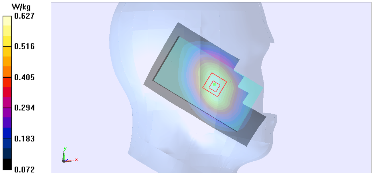
Figure 78 Left Hand Touch Cheek UMTS Band V Channel 4233
