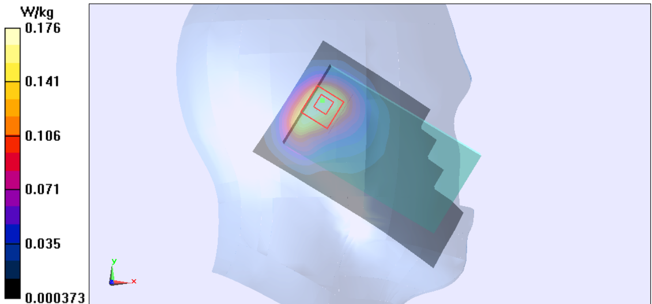
Figure 104 Left Hand Tilt 15° 802.11b Channel 1
