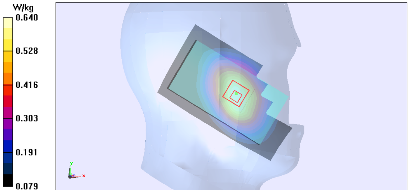
Figure 80 Left Hand Touch Cheek UMTS Band V Channel 4132
