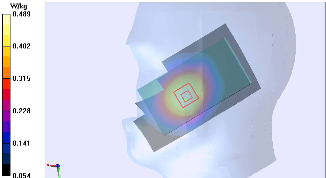
Figure 22 Right Touch Cheek GSM 850 Channel 190
