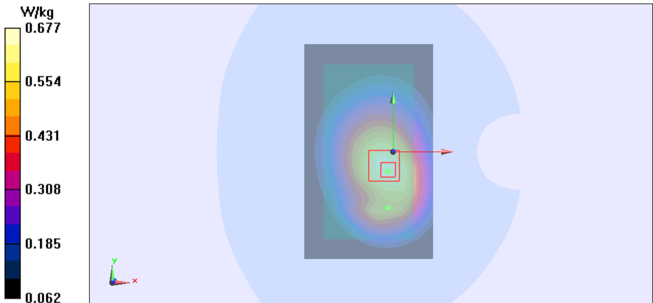
Figure 102 Body, Back Side, UMTS Band V Channel 4183
