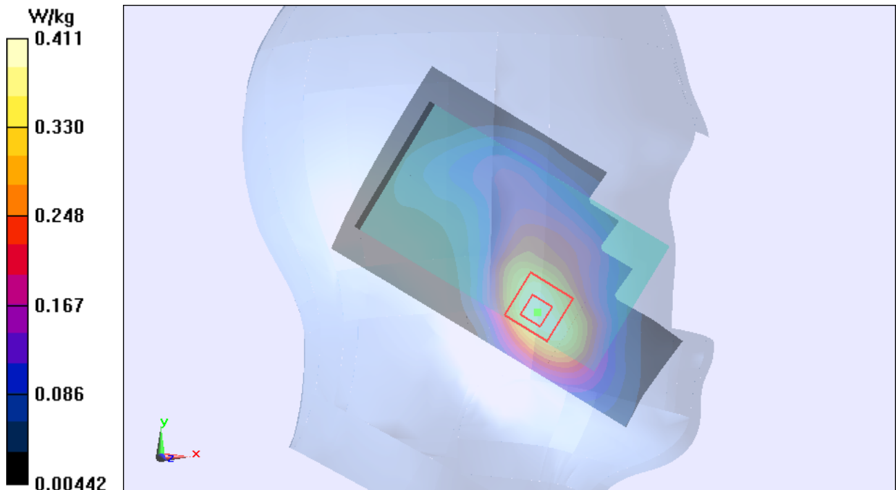
Figure 43 Left Hand Touch Cheek GSM 1900 Channel 661
