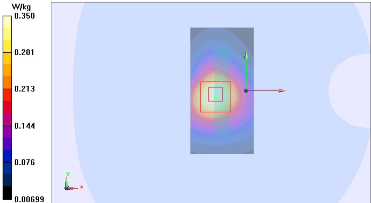
Figure 48 Body, Bottom Edge, GSM 1900 GPRS (2Txslots) Channel 661
