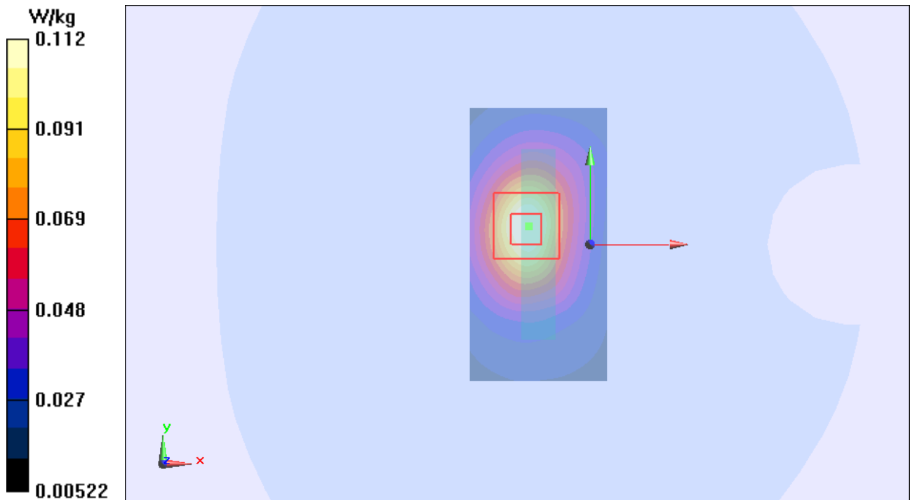
Figure 27 Body, Bottom Edge, GSM 850 GPRS (2Txslots)annel 190
