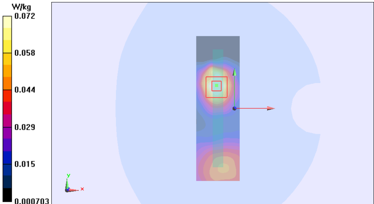
Figure 47 Body, Right Edge, GSM 1900 GPRS (2Txslots) Channel 661
