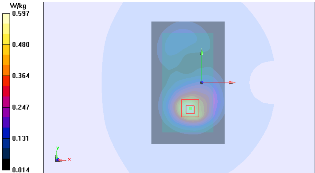
Figure 53 Body, Back Side, GSM 1900 GPRS (2Txslots) Channel 661
