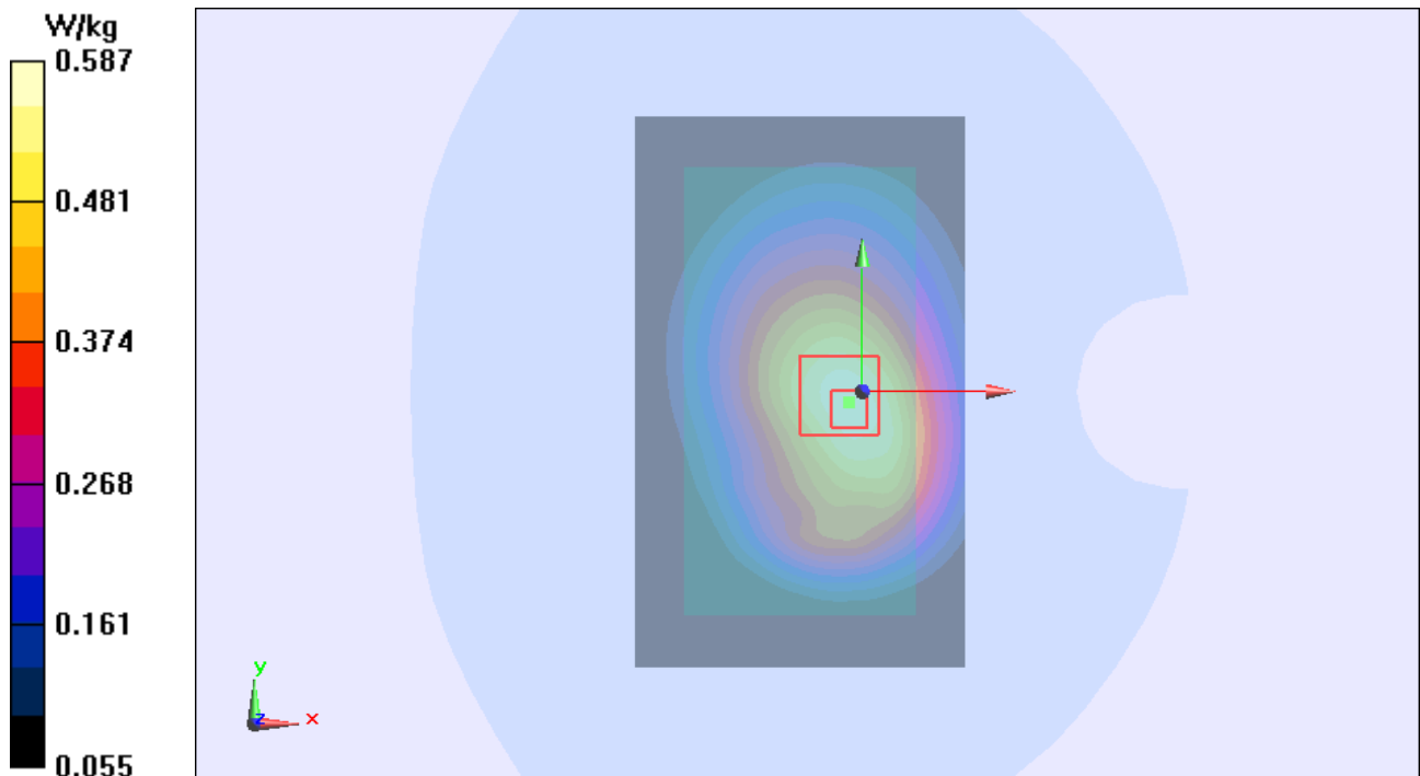
Figure 31 Body, Back Side, GSM 850 GPRS (2Txslots) Channel 190
