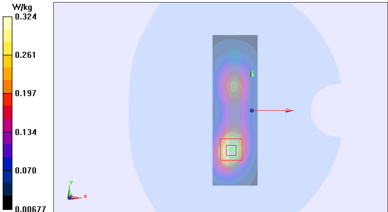
Figure 68 Body, Left Edge, UMTS Band II Channel 9400
