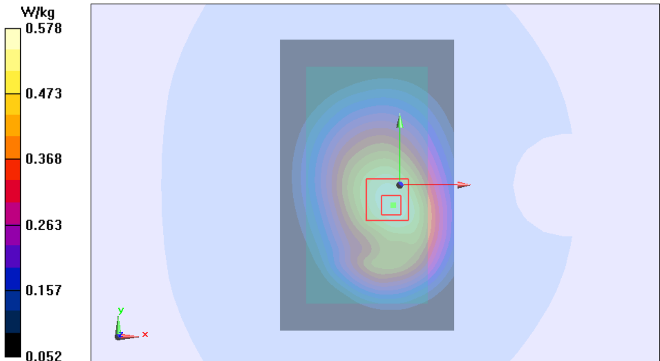
Figure 30 Body, Back Side, GSM 850 GPRS (2Txslots) Channel 190
