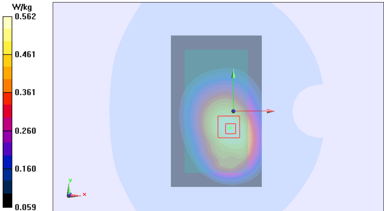
Figure 33 Body, Back Side, GSM 850 GPRS (2Txslots) Channel 190
