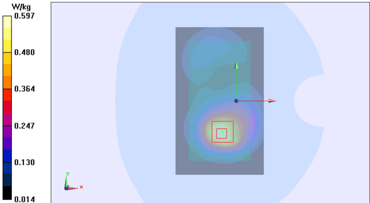
Figure 49 Body, Back Side, GSM 1900 GPRS (2Txslots) Channel 661
