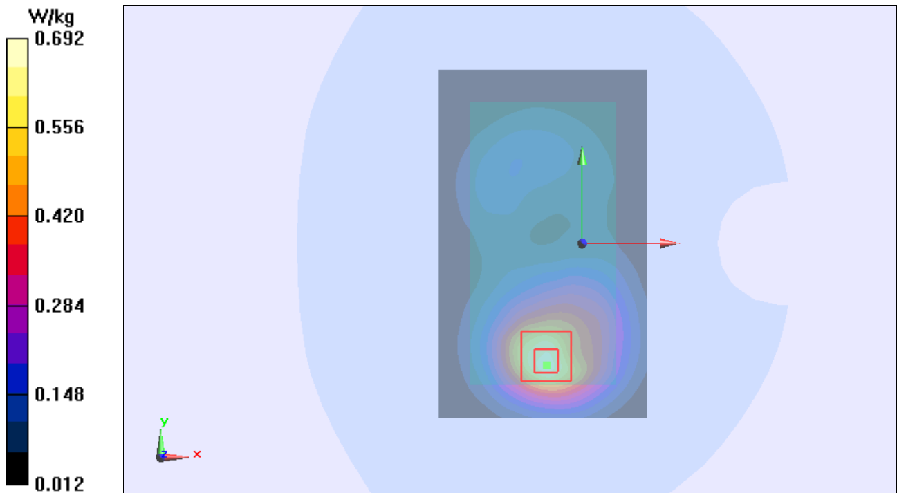
Figure 54 Body, Back Side, GSM 1900 GPRS (2Txslots) Channel 661
