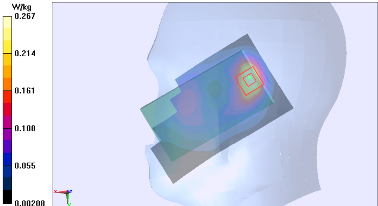
Figure 58 Right Hand Tilt 15° UMTS Band II Channel 9400
