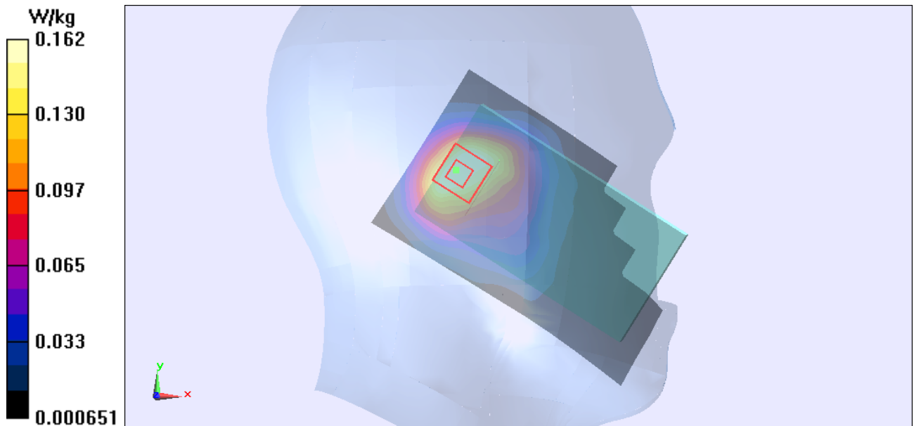
Figure 103 Left Hand Touch Cheek 802.11b Channel 1
