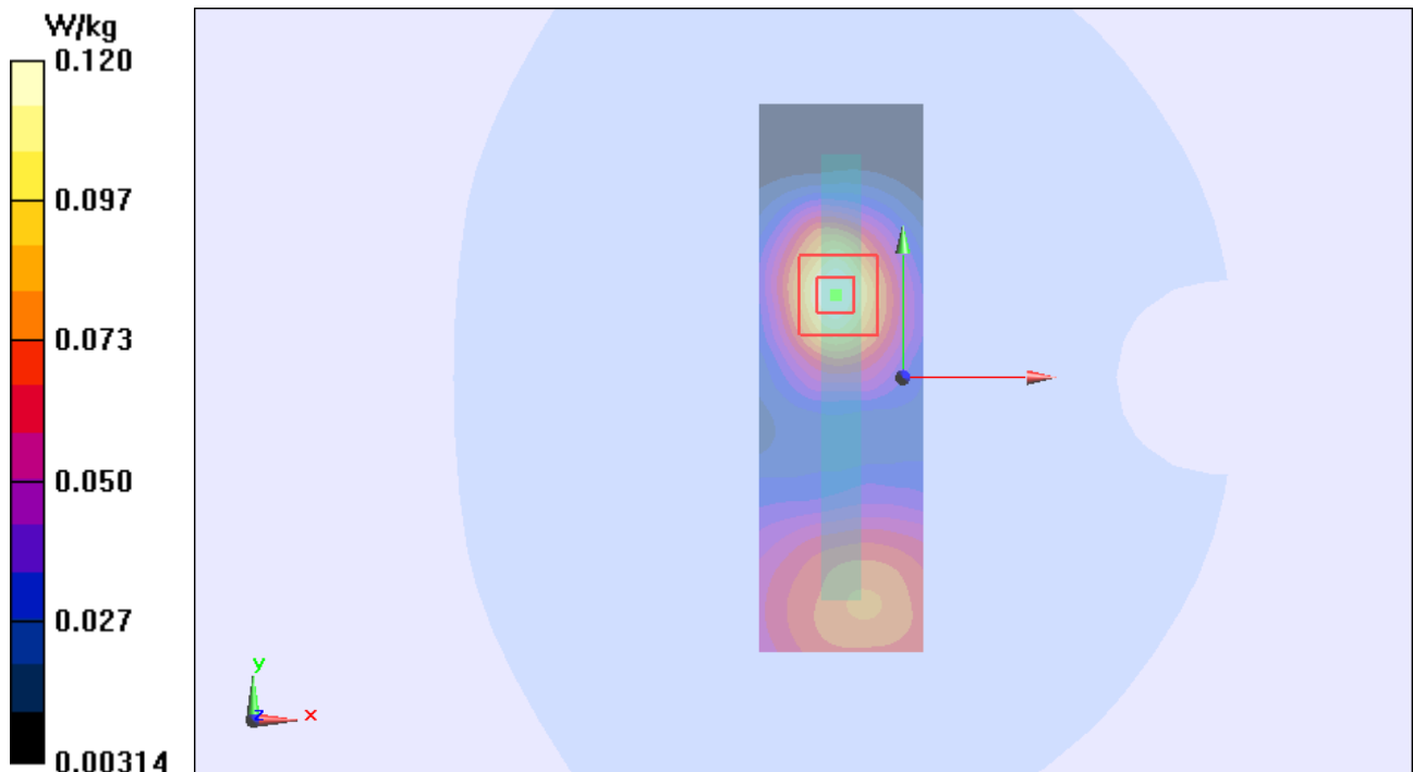
Figure 69 Body, Right Edge, UMTS Band II Channel 9400
