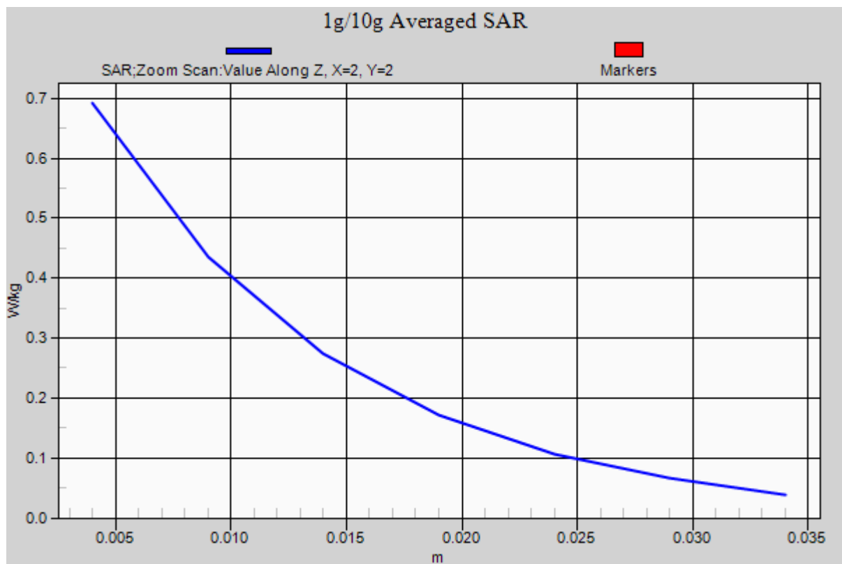
Figure 44 Body, Back Side, GSM 1900 GPRS (2Txslots) Channel 661
