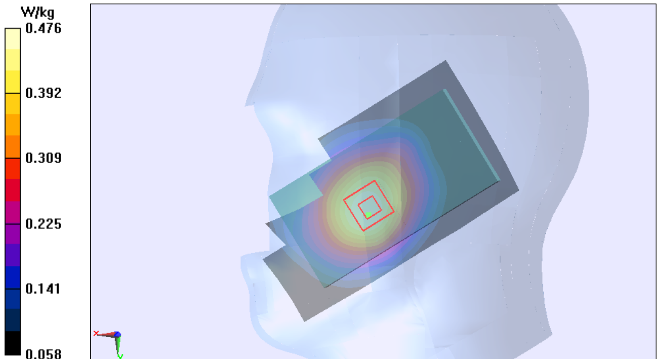
Figure 20 Right Touch Cheek GSM 850 Channel 190
