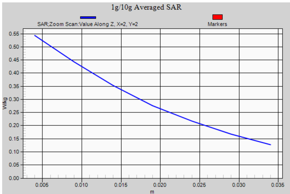
Figure 17 Right Touch Cheek GSM 850 Channel 190
