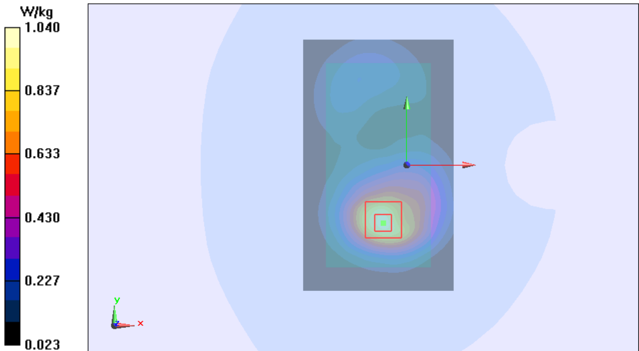
Figure 74 Body, Back Side, UMTS Band II Channel 9262
