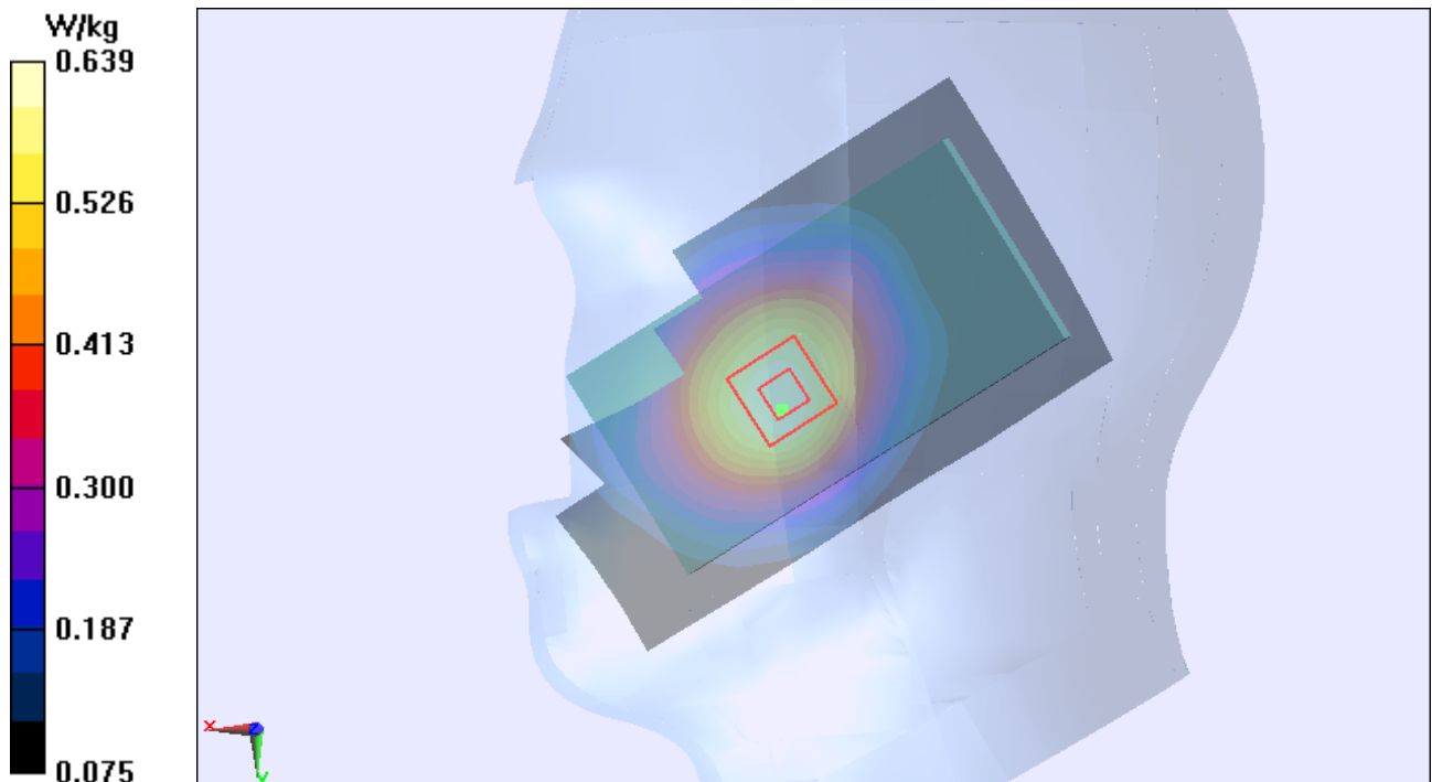
Figure 83 Right Hand Touch Cheek UMTS Band V Channel 4183
