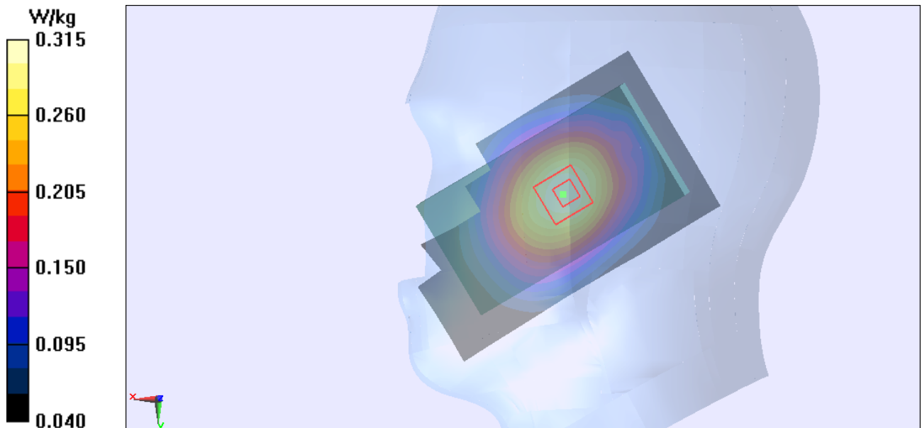
Figure 85 Right Hand Tilt 15° UMTS Band V Channel 4183
