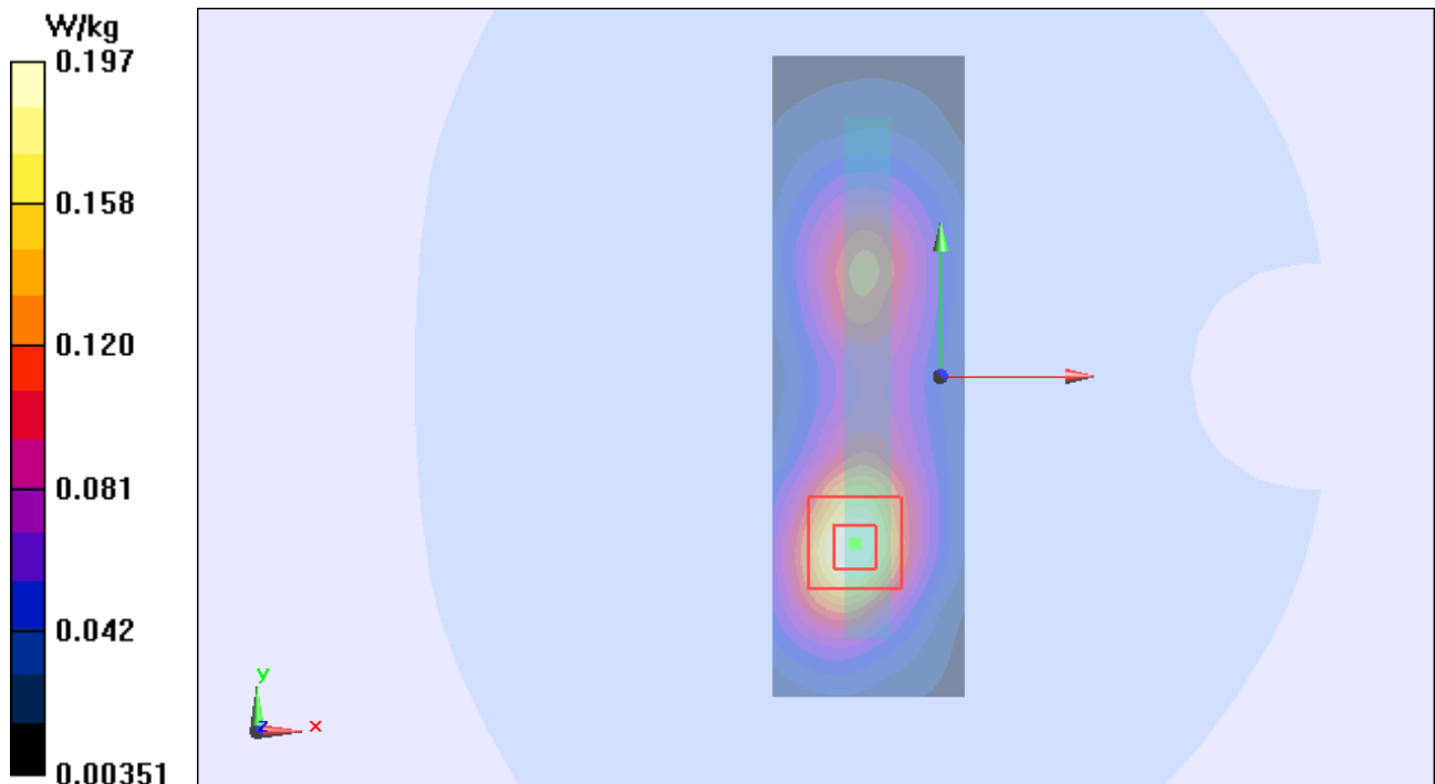
Figure 46 Body, Left Edge, GSM 1900 GPRS (2Txslots) Channel 661
