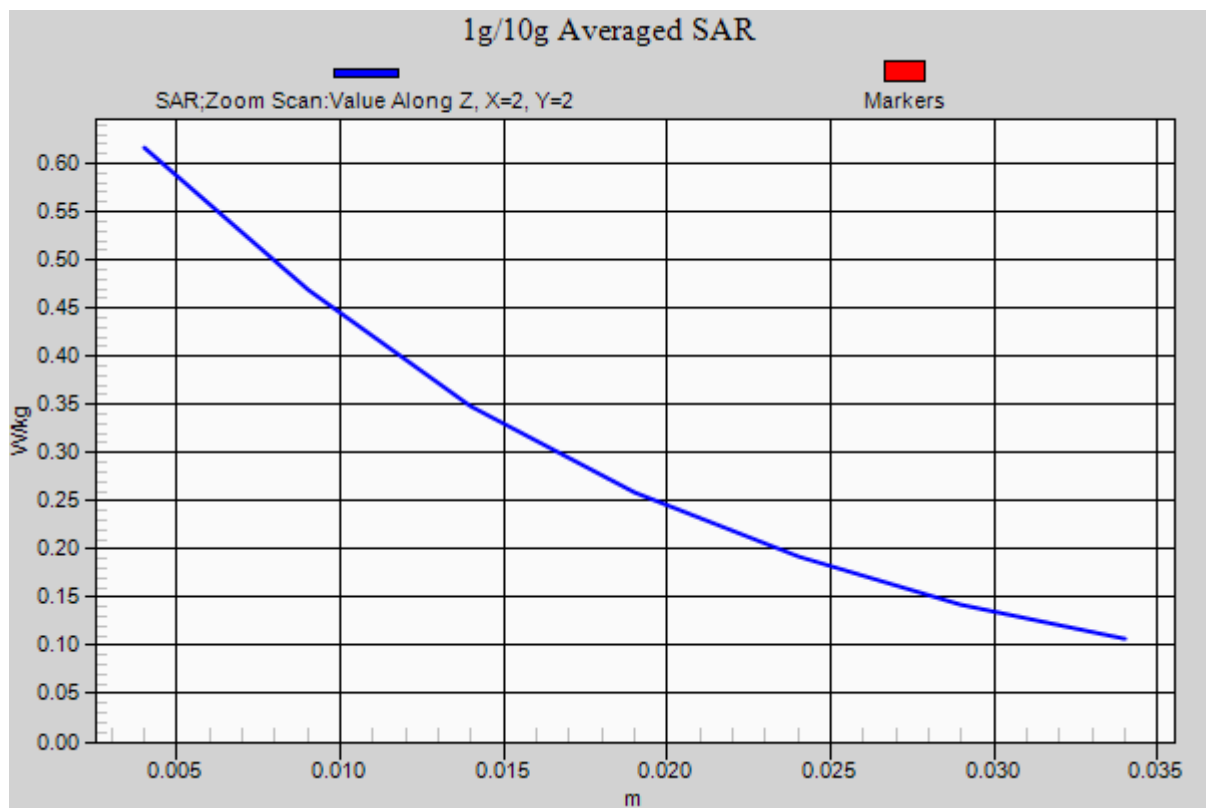
Figure 28 Body, Back Side, GSM 850 GPRS (2Txslots) Channel 190
