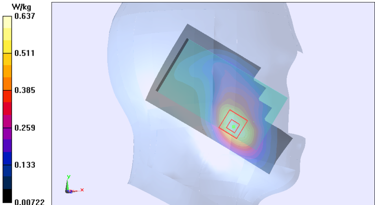
Figure 55 Left Hand Touch Cheek UMTS Band II Channel 9400
