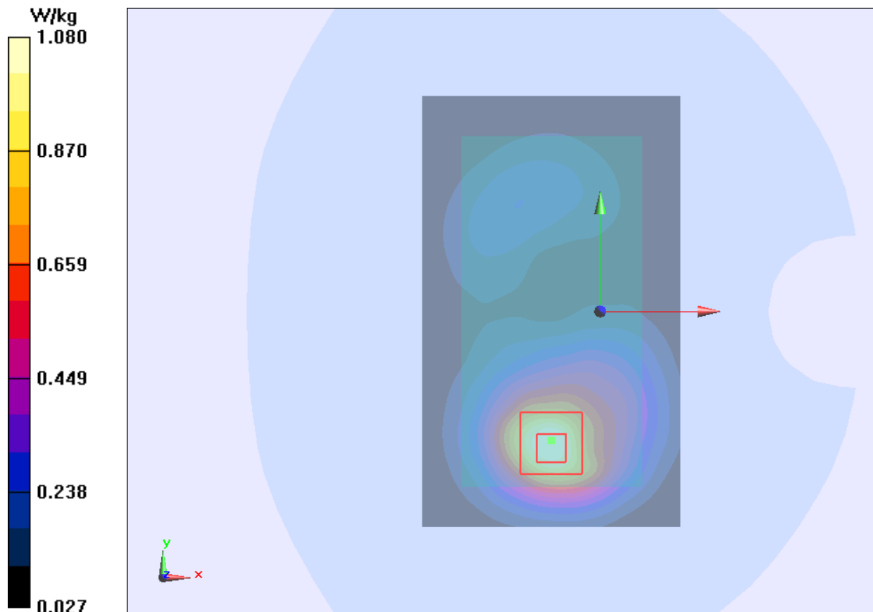
Figure 65 Body, Back Side, UMTS Band II Channel 9400
