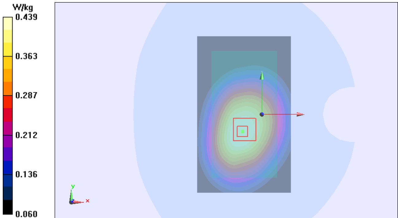
Figure 24 Body, Front Side, GSM 850 GPRS (2Txslots)Channel 190
