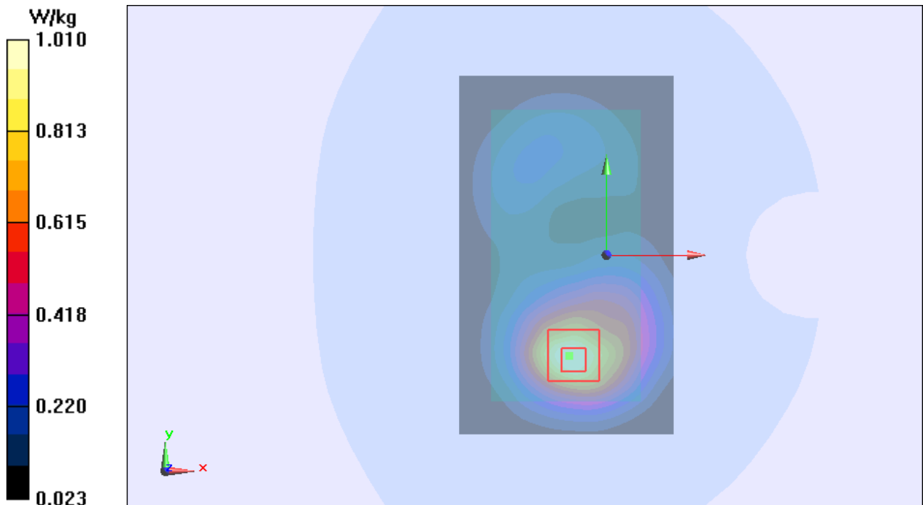
Figure 72 Body, Back Side, UMTS Band II Channel 9262
