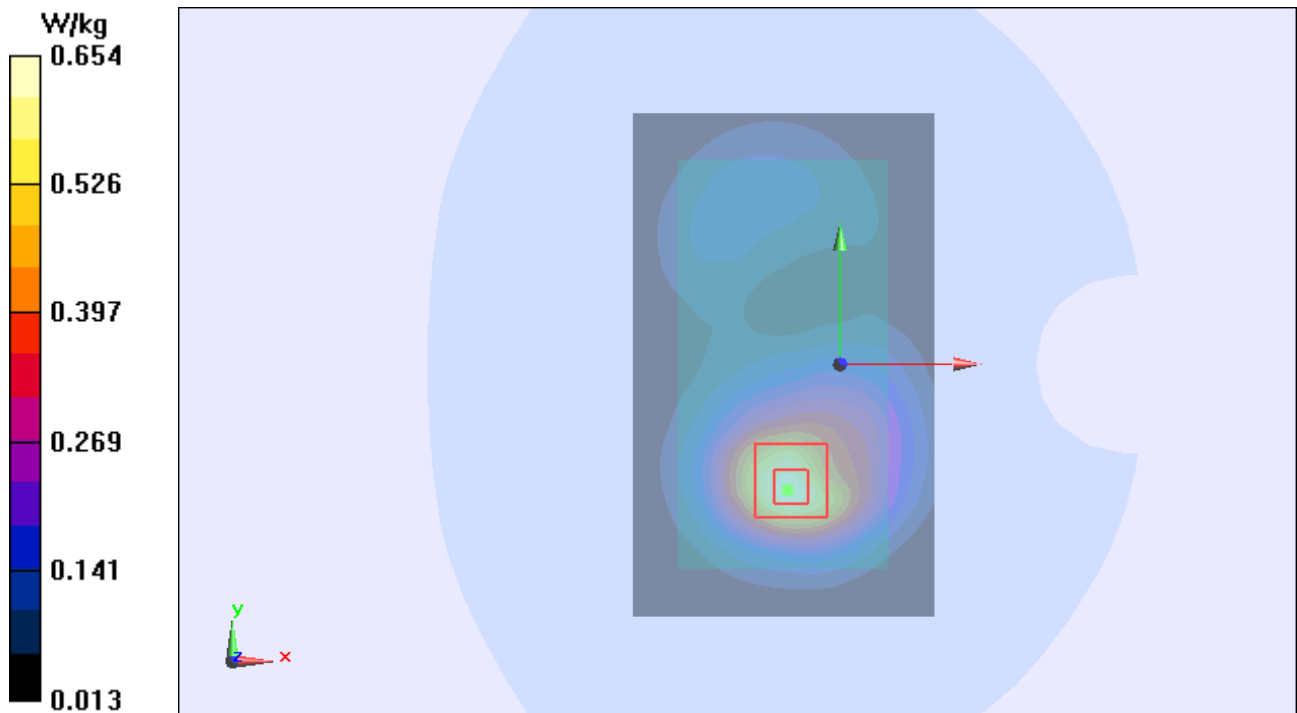
Figure 52 Body, Back Side, GSM 1900 GPRS (2Txslots) Channel 661
