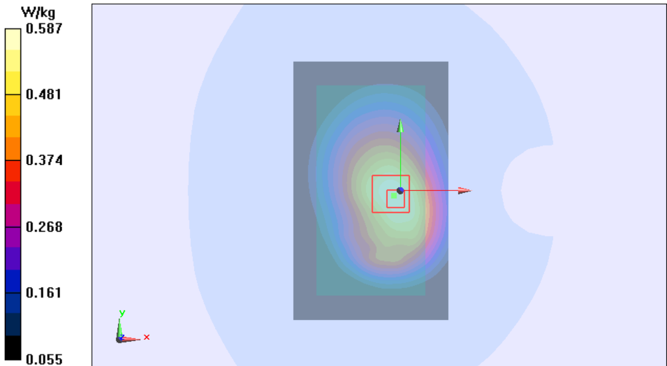
Figure 32 Body, Back Side, GSM 850 GPRS (2Txslots) Channel 190
