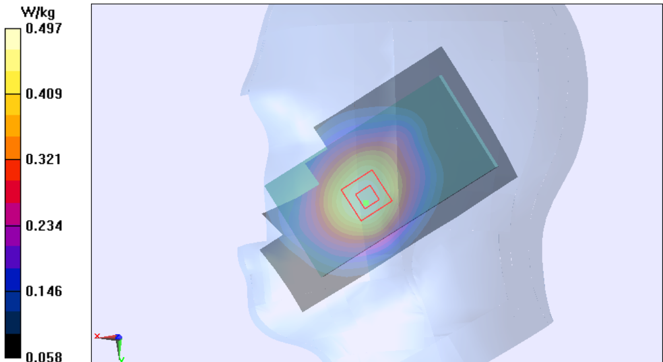
Figure 15 Right Hand Touch Cheek GSM 850 Channel 190
