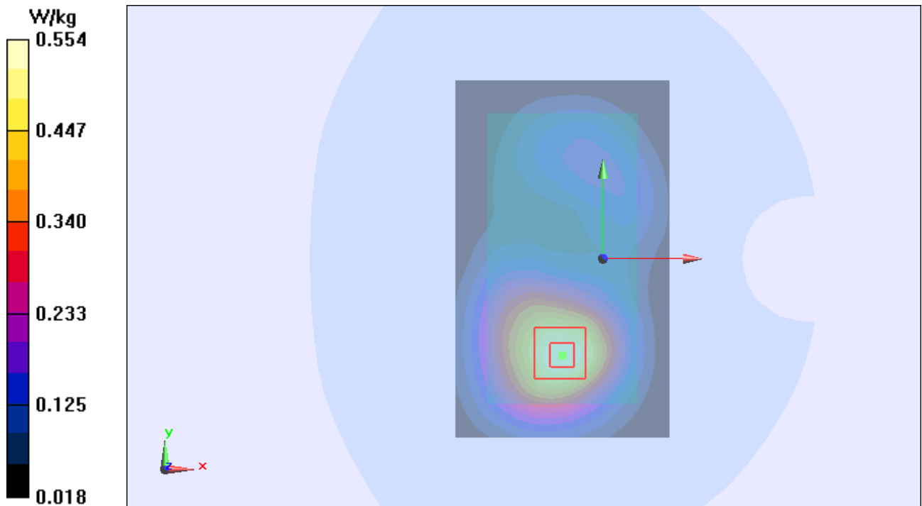
Figure 67 Body, Front Side, UMTS Band II Channel 9400
