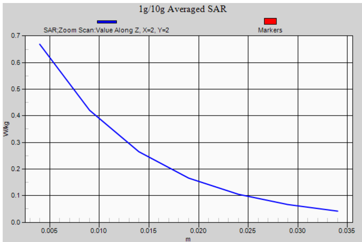
Figure 60 Left Hand Touch Cheek UMTS Band II Channel 9400
