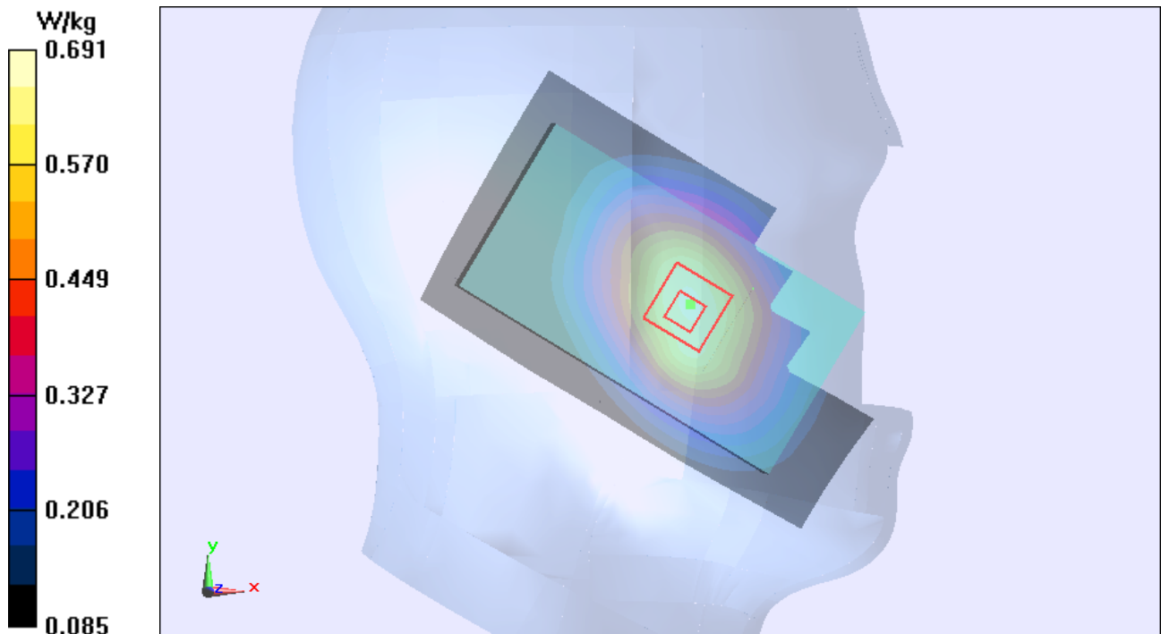
Figure 86 Left Touch Cheek UMTS Band V Channel 4183
