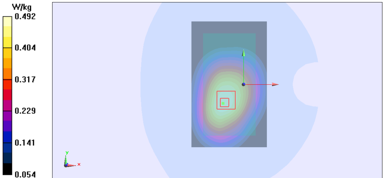
Figure 94 Body, Front Side, UMTS Band V Channel 4183
