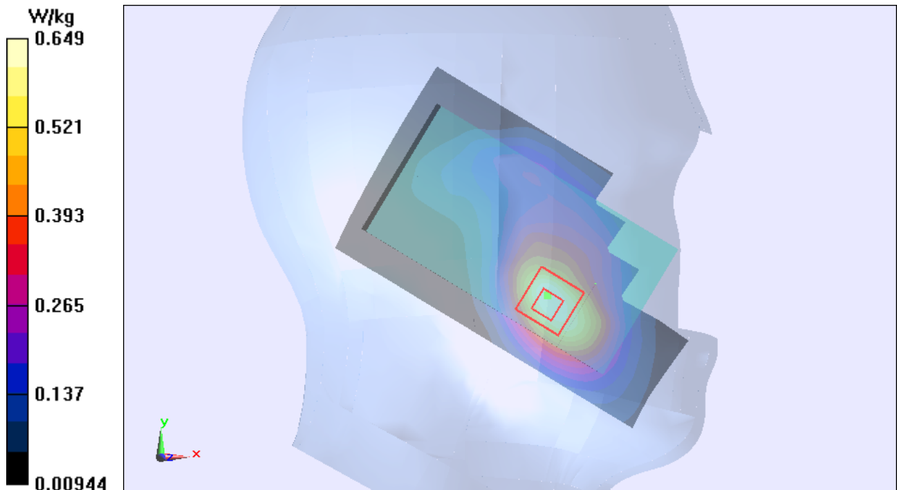
Figure 59 Left Hand Touch Cheek UMTS Band II Channel 9400
