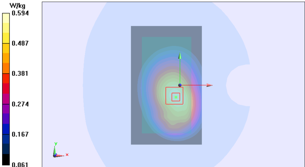
Figure 23 Body, Back Side, GSM 850 GPRS (2Txslots) Channel 190
