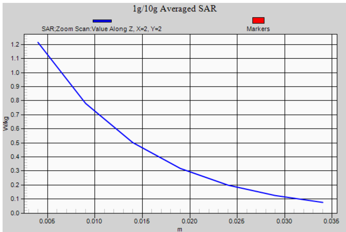
Figure 77 Body, Back Side, UMTS Band II Channel 9262
