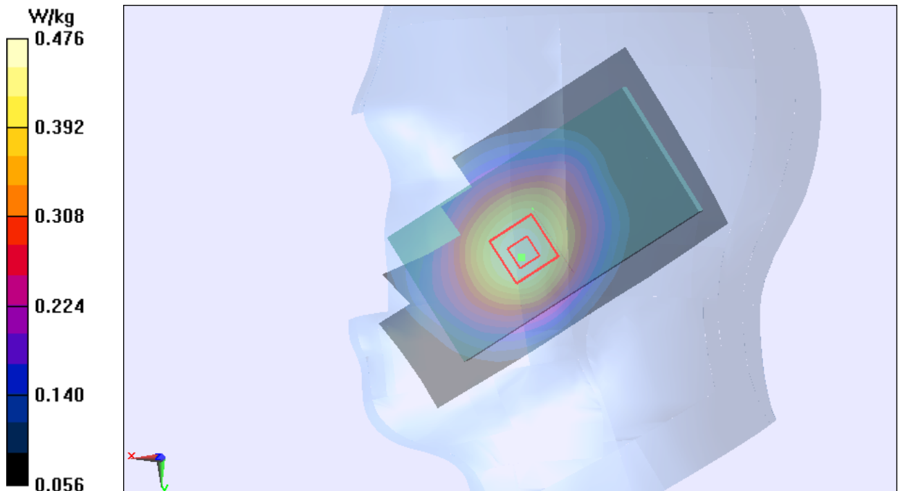
Figure 21 Right Touch Cheek GSM 850 Channel 190
