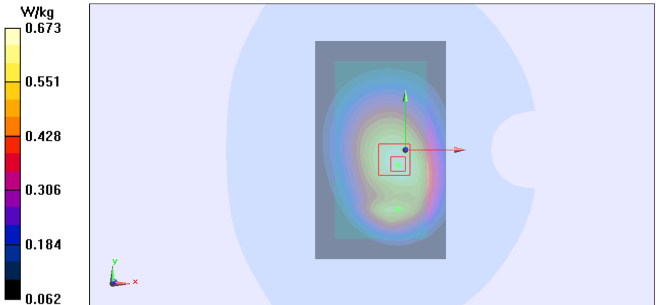
Figure 92 Body, Back Side, UMTS Band V Channel 4183
