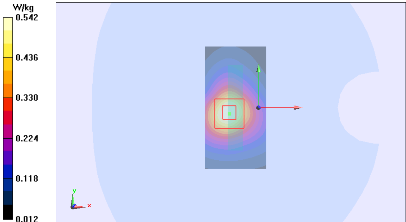
Figure 70 Body, Bottom Edge, UMTS Band II Channel 9400
