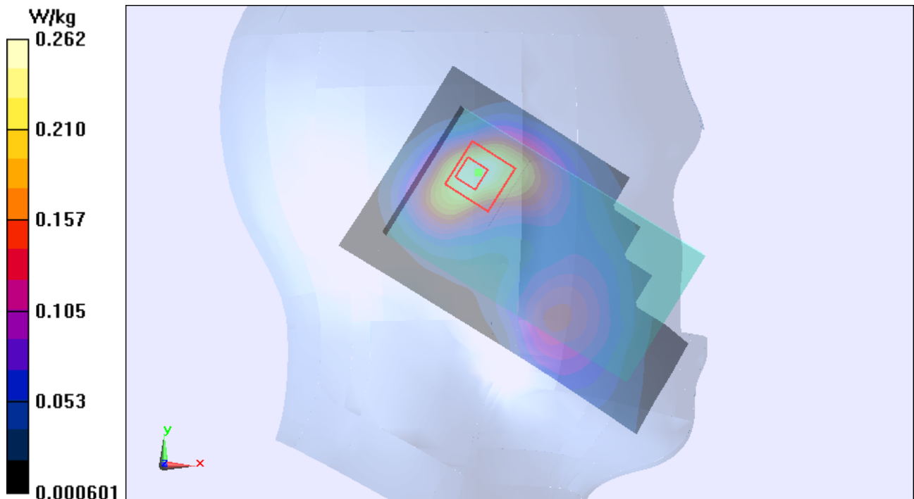
Figure 56 Left Hand Tilt 15° UMTS Band II Channel 9400
