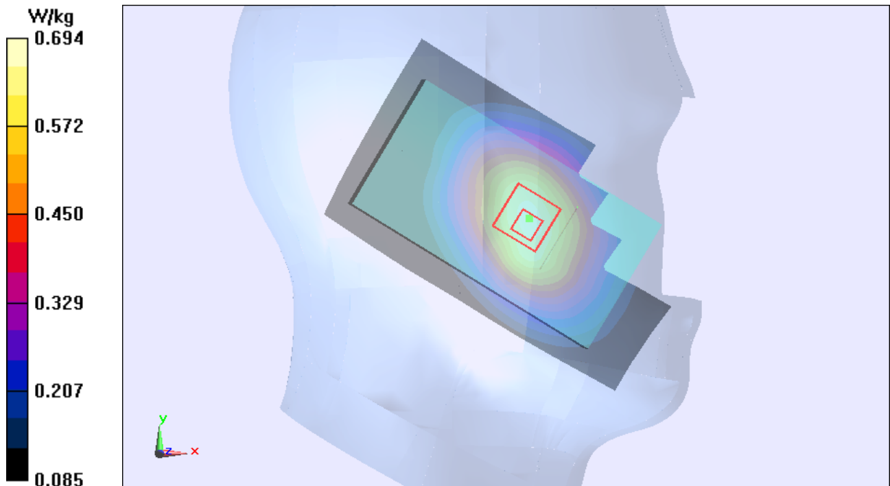
Figure 88 Left Touch Cheek UMTS Band V Channel 4183
