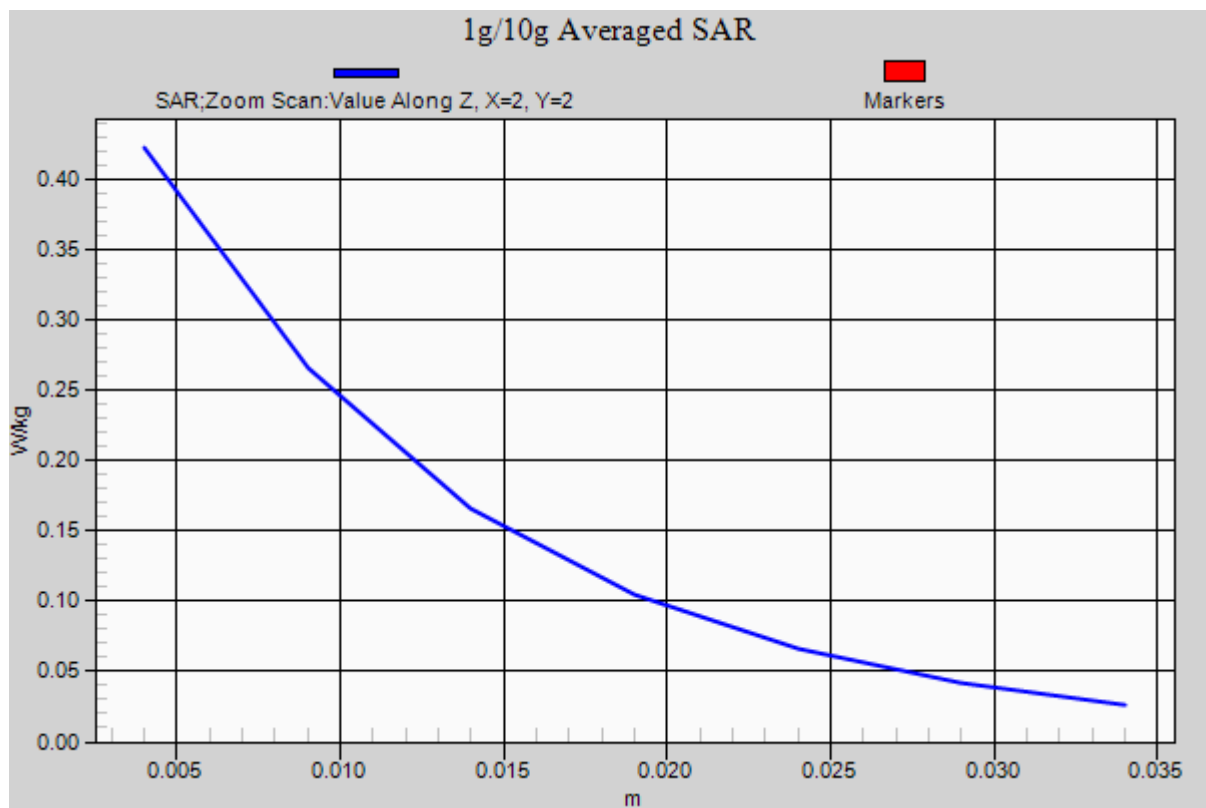
Figure 42 Left Hand Touch Cheek GSM 1900 Channel 661
