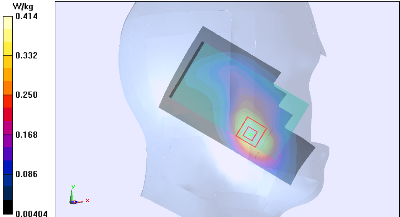
Figure 34 Left Hand Touch Cheek GSM 1900 Channel 661
