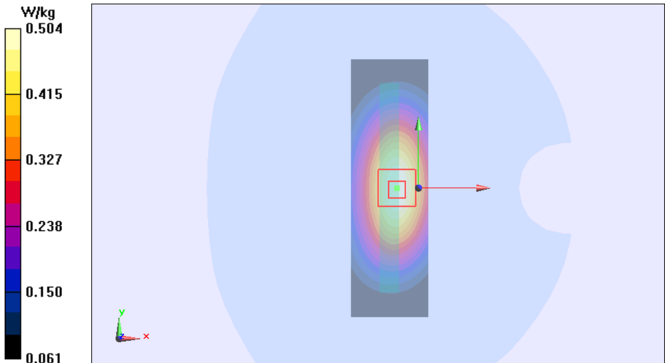
Figure 25 Body, Left Edge, GSM 850 GPRS (2Txslots)Channel 190
