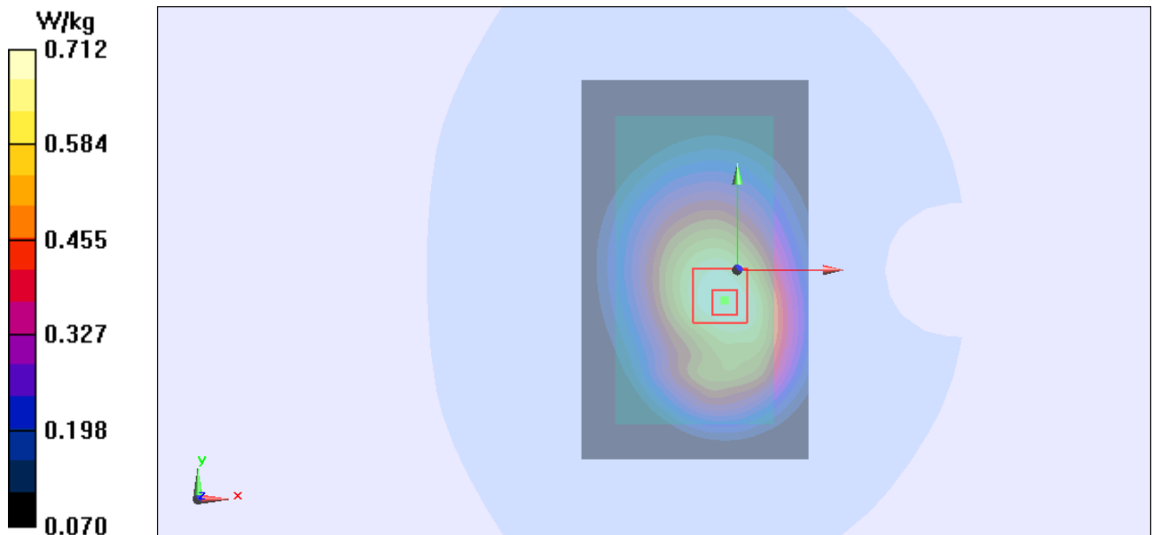
Figure 99 Body, Back Side, UMTS Band V Channel 4183
