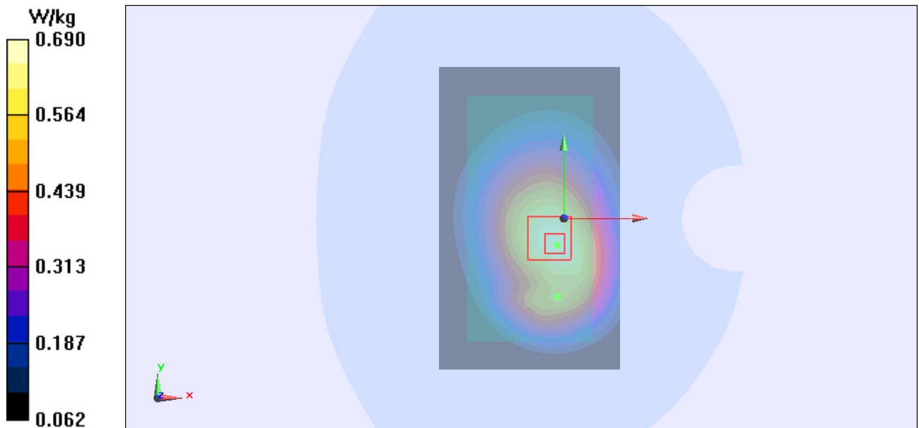
Figure 101 Body, Back Side, UMTS Band V Channel 4183
