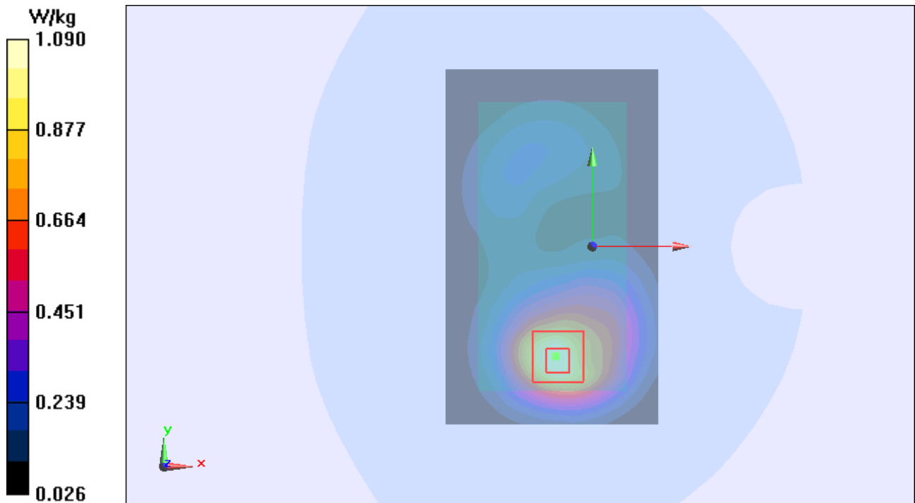
Figure 75 Body, Back Side, UMTS Band II Channel 9262
