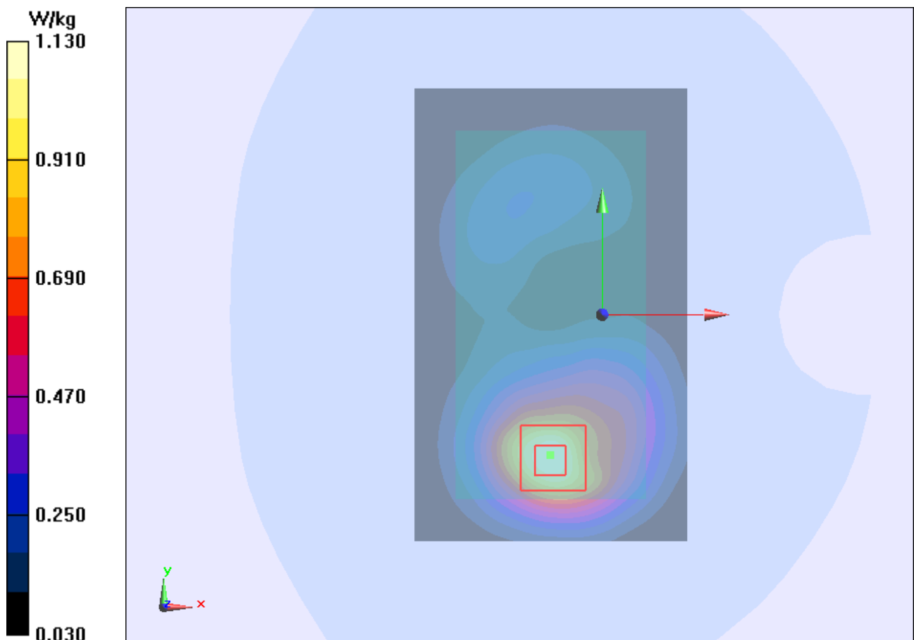
Figure 66 Body, Back Side, UMTS Band II Channel 9262
