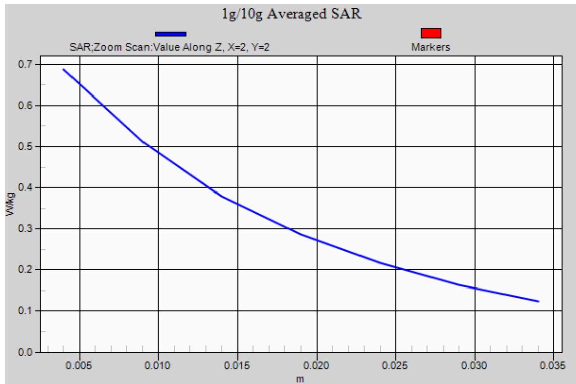
Figure 79 Left Hand Touch Cheek UMTS Band V Channel 4183
