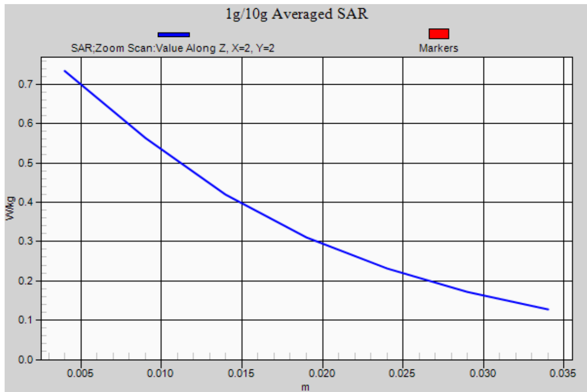
Figure 98 Body, Back Side, UMTS Band V Channel 4183
