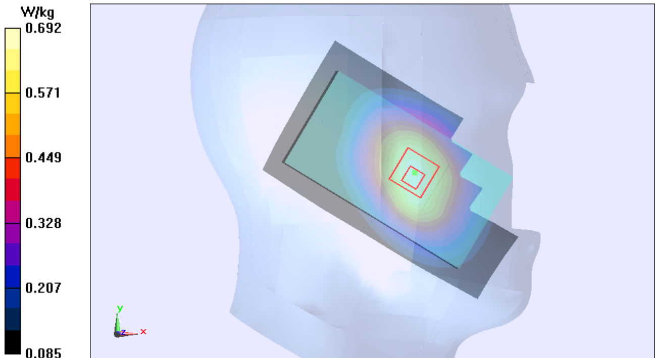
Figure 89 Left Touch Cheek UMTS Band V Channel 4183
