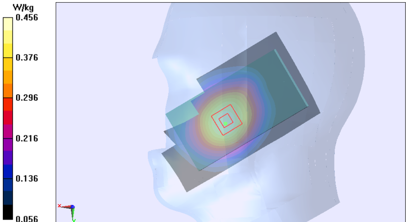
Figure 19 Right Touch Cheek GSM 850 Channel 190
