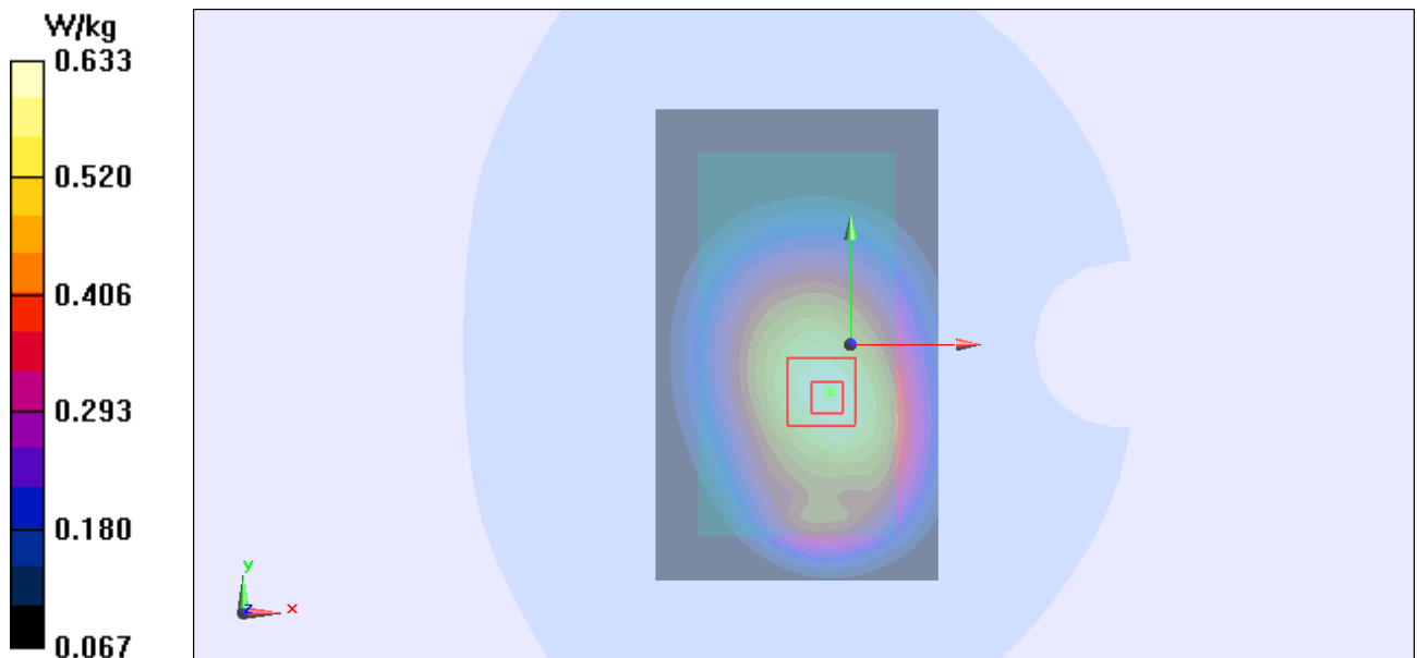
Figure 91 Body, Back Side, UMTS Band V Channel 4233
