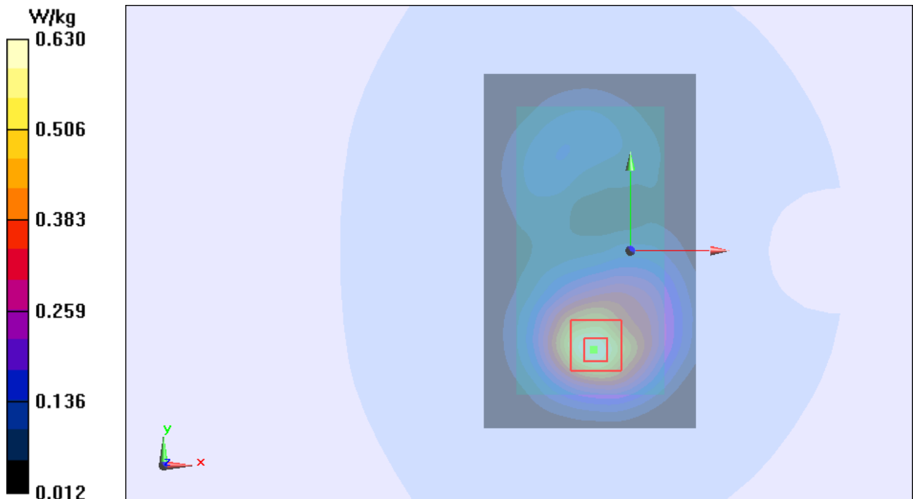
Figure 51 Body, Back Side, GSM 1900 GPRS (2Txslots) Channel 661
