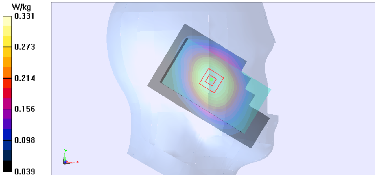
Figure 81 Left Hand Tilt 15° UMTS Band V Channel 4183
