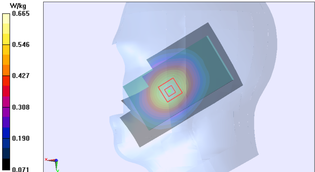
Figure 82 Right Hand Touch Cheek UMTS Band V Channel 4233
