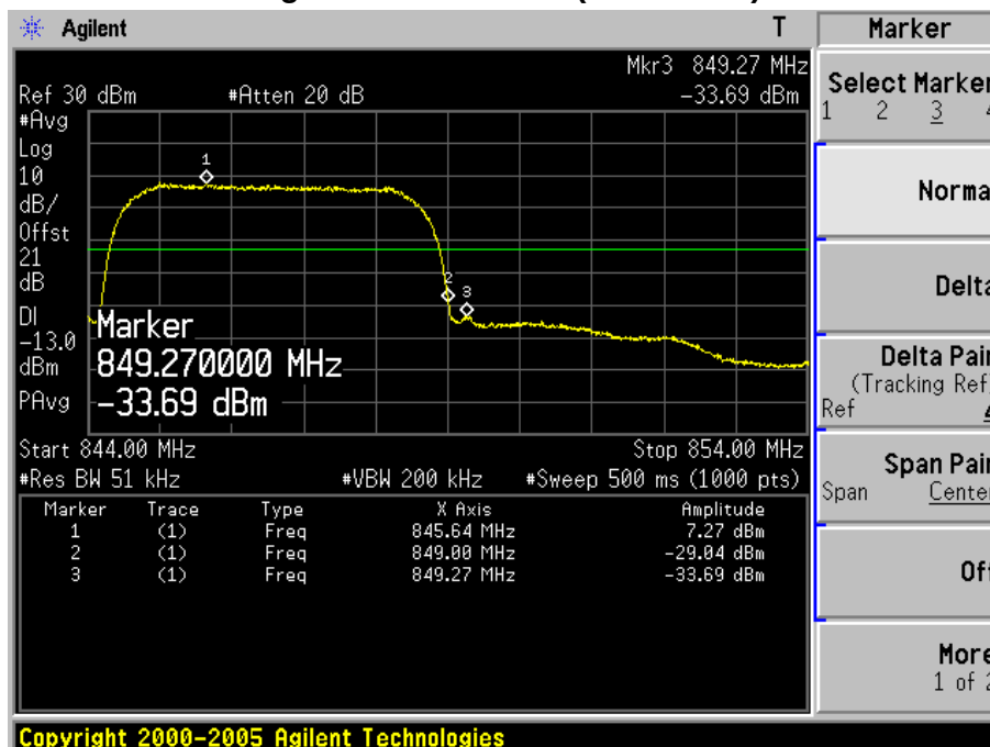
Figure Channel 4233 (846.60MHz)
