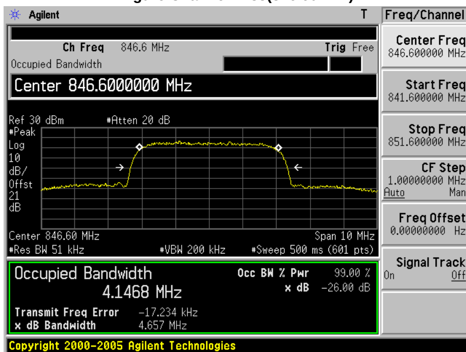
Figure Channel 4233(846.60MHz)
