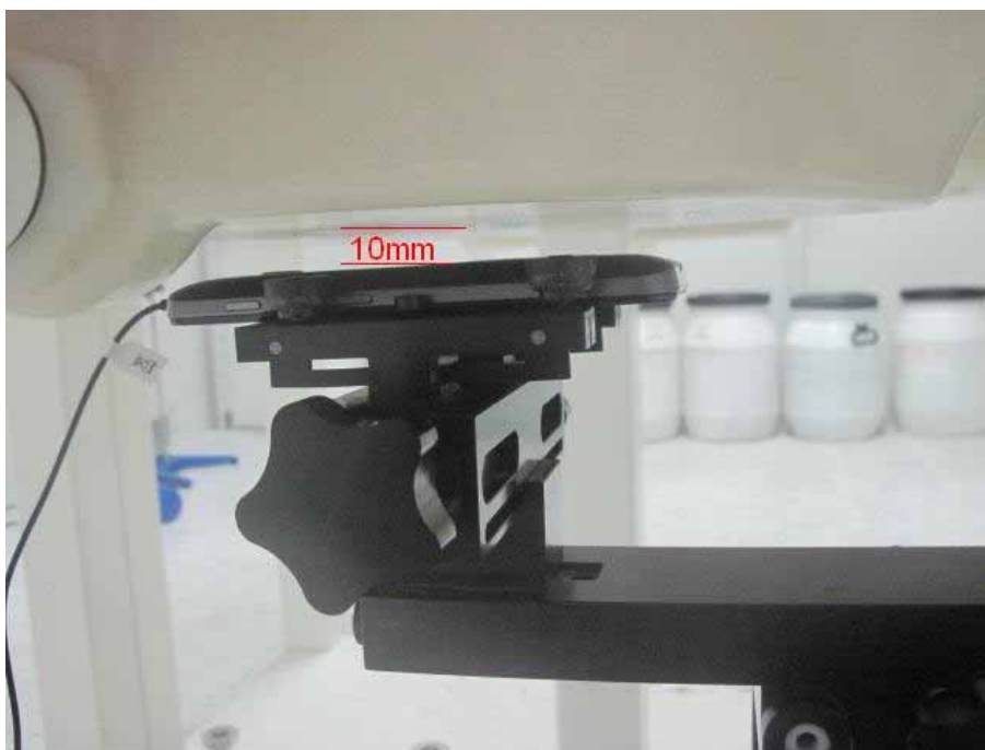
Body SAR Back with headset #2 10mm
