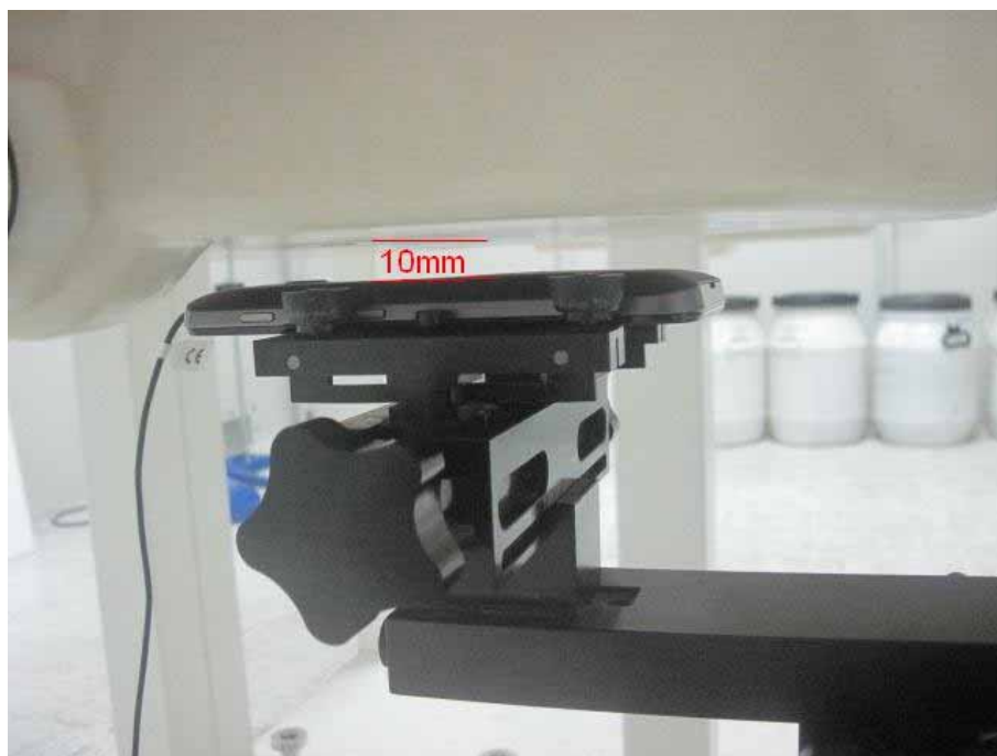
Body SAR Back with headset #1 10mm
