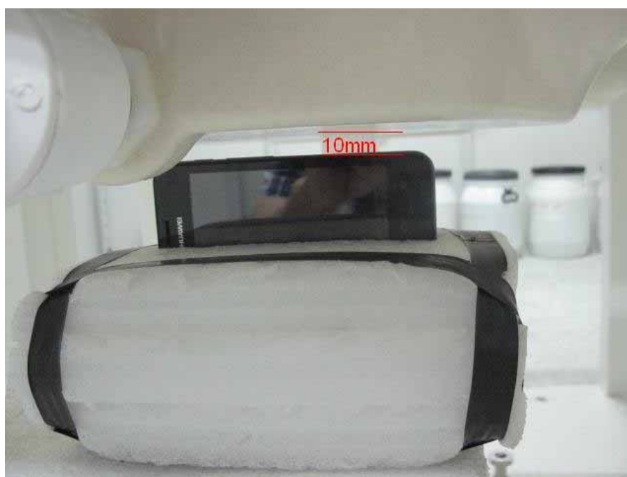
Body SAR Right Side 10mm for Wi-Fi
