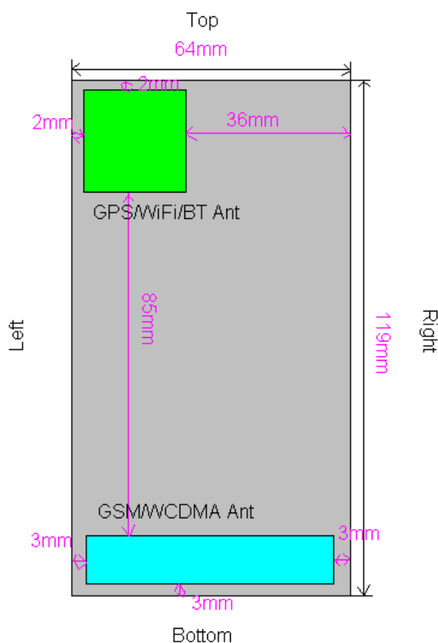
Mobile Hotspot Sides for SAR Testing
