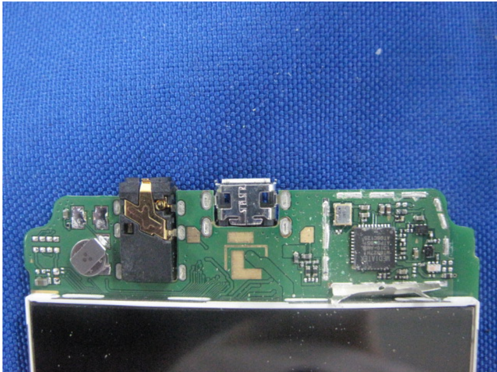
(13) EUT Photo(Single SIM Slot)
