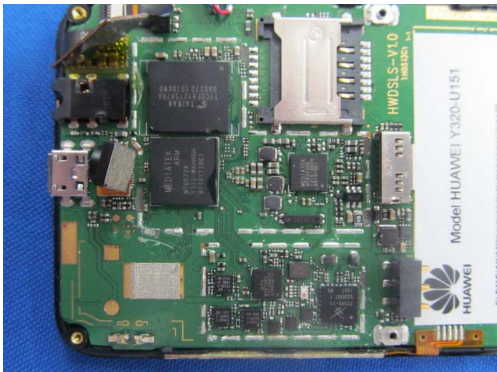
(6) EUT Photo(Single SIM Slot)
