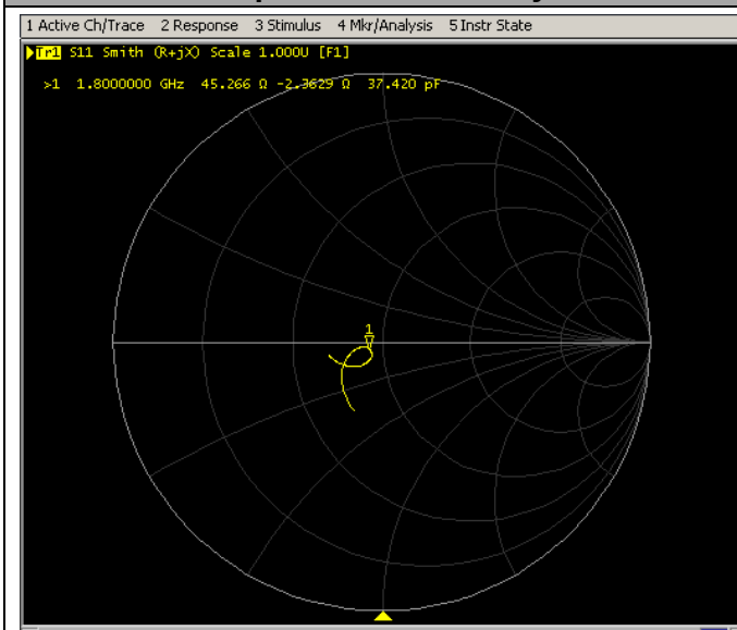
Impedance Test-Body
