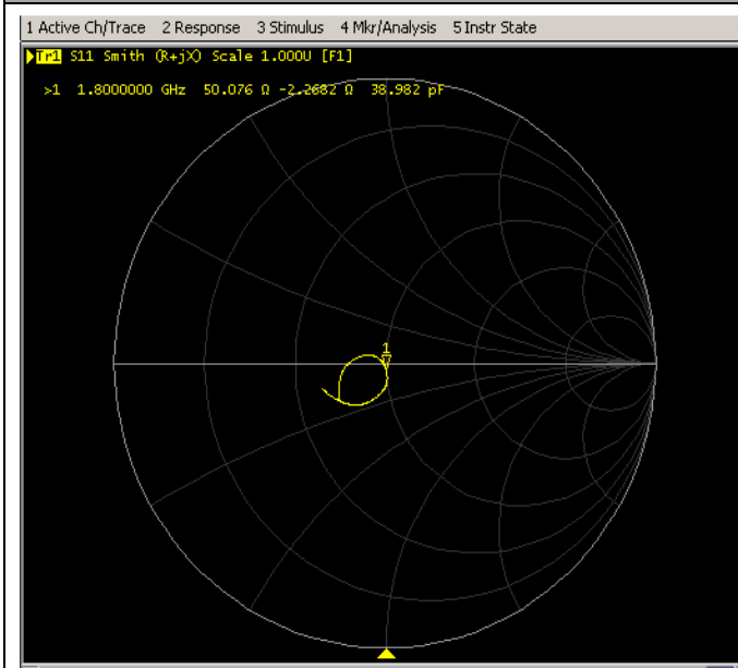
Impedance Test-Body
