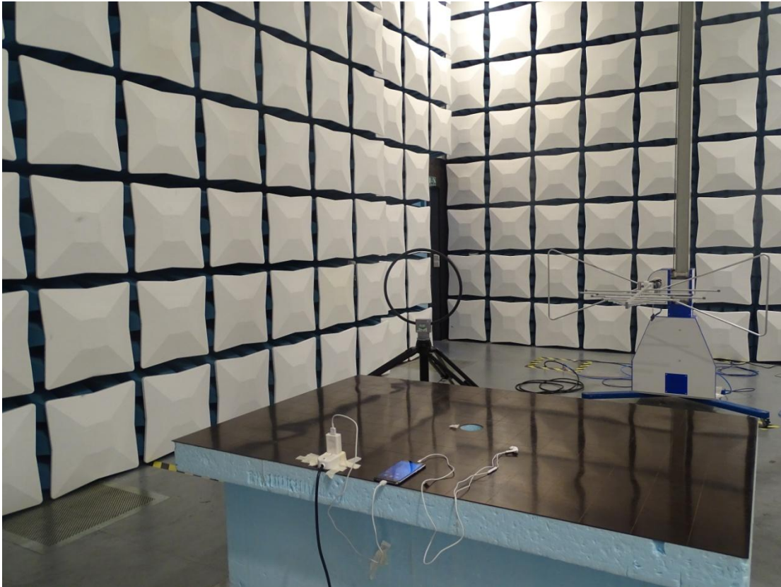
Radiated Spurious Emission (9KHz--30MHZ & 30MHZ-1GHz)
