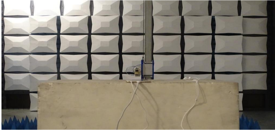
Radiated Spurious Emission (above 18GHz)
