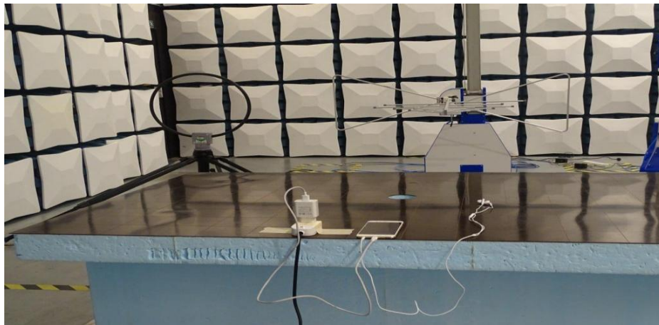
Radiated Spurious Emission (9K-30MHz)
