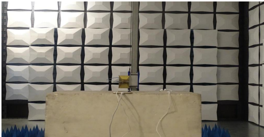
Radiated Spurious Emission (1GHz to 18GHz)
