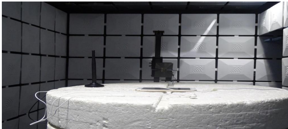
Radiated Spurious Emission (3GHz to18GHz)
