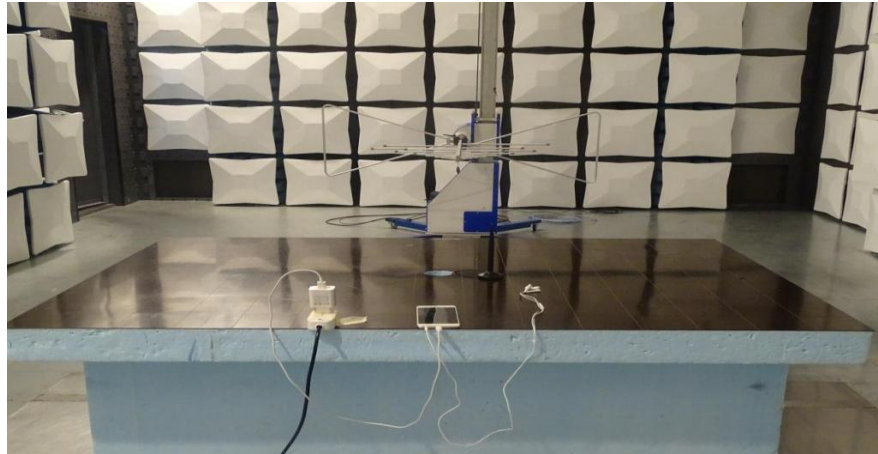
Radiated Spurious Emission (below 1GHz)
