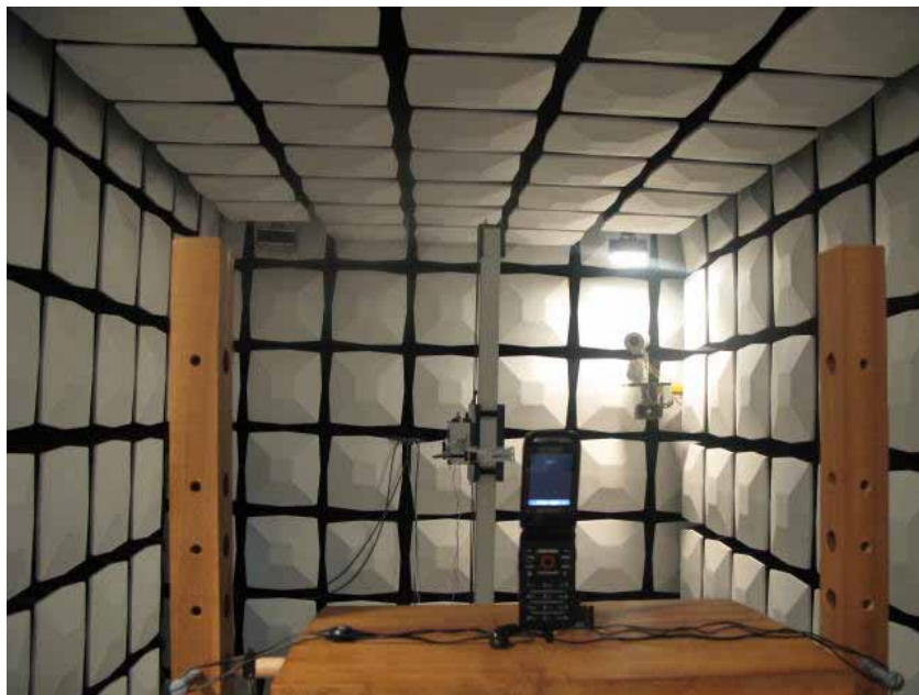
Radiated Spurious Emission 18G~26.5GHz
