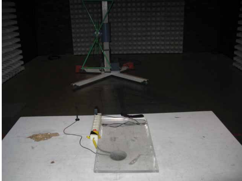
Radiated Disturbance
