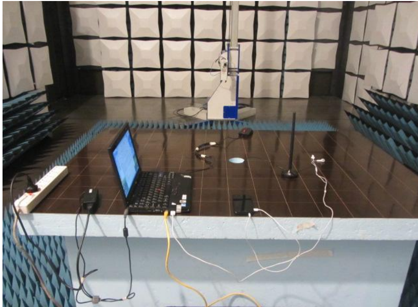
Radiated Spurious Emission (above 18GHz)
