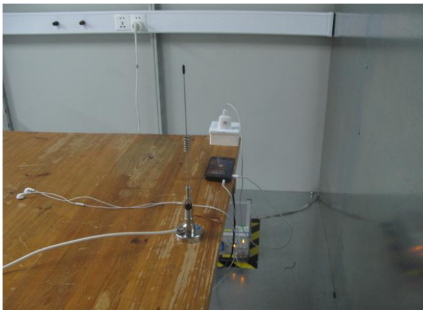
Conducted Emissions for AC Ports
