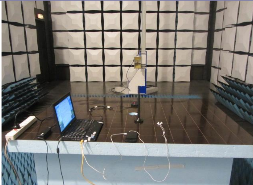
Radiated Spurious Emission (1GHz to18GHz)
