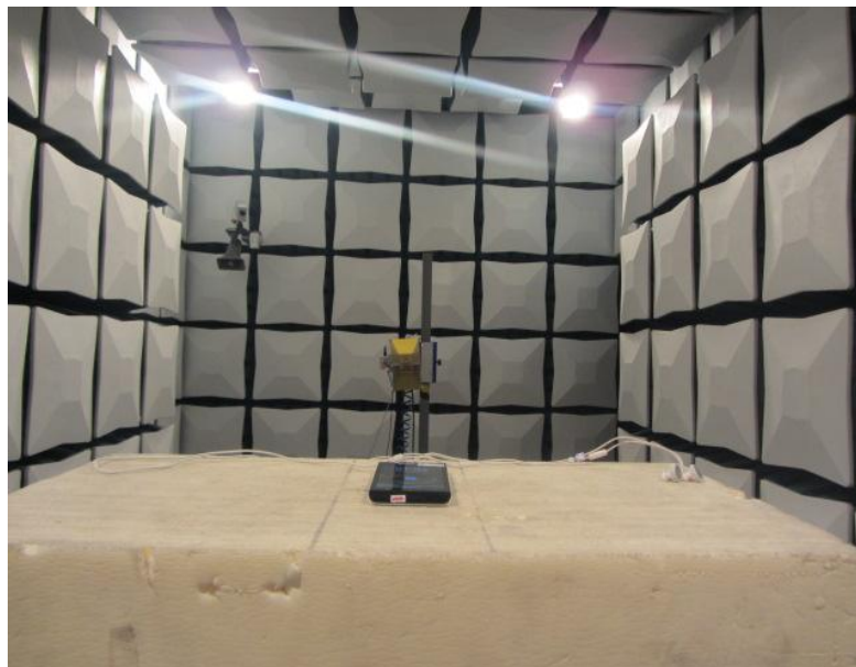
Radiated Spurious Emission (3GHz to18GHz)
