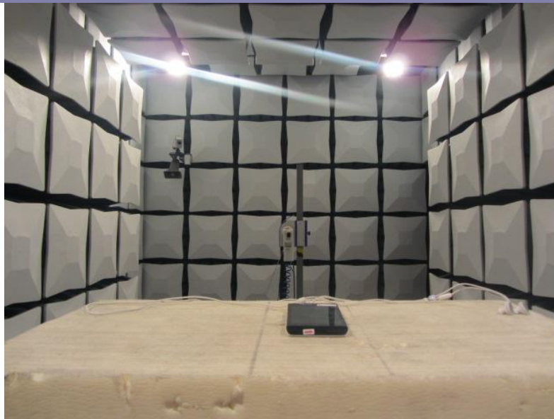
Radiated Spurious Emission (18GHz to26.5GHz)
