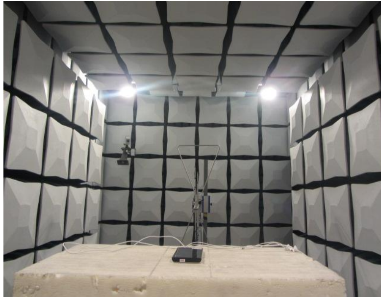
Radiated Spurious Emission (below 3GHz)
