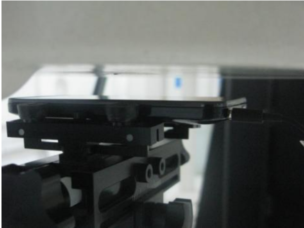
Photo 14:Towards Phantom with Headset (10mm)
