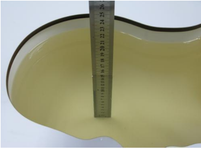
Photo 18:HSL1900MHz depth (15.2cm)
