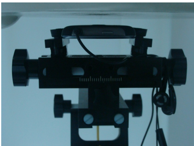
Back of the DUT with Phantom 1 cm Gap (with Earphone 2)
