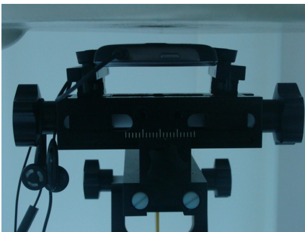
Back of the DUT with Phantom 1 cm Gap (with Earphone 1)
