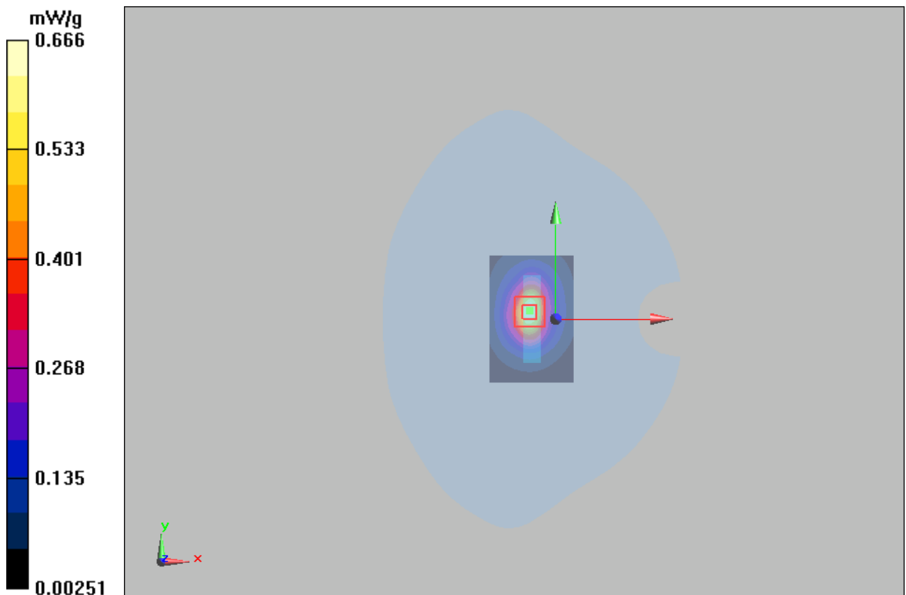
Figure 42 Body, Bottom Edge, GSM 1900 GPRS (2Txslots) Channel 661
