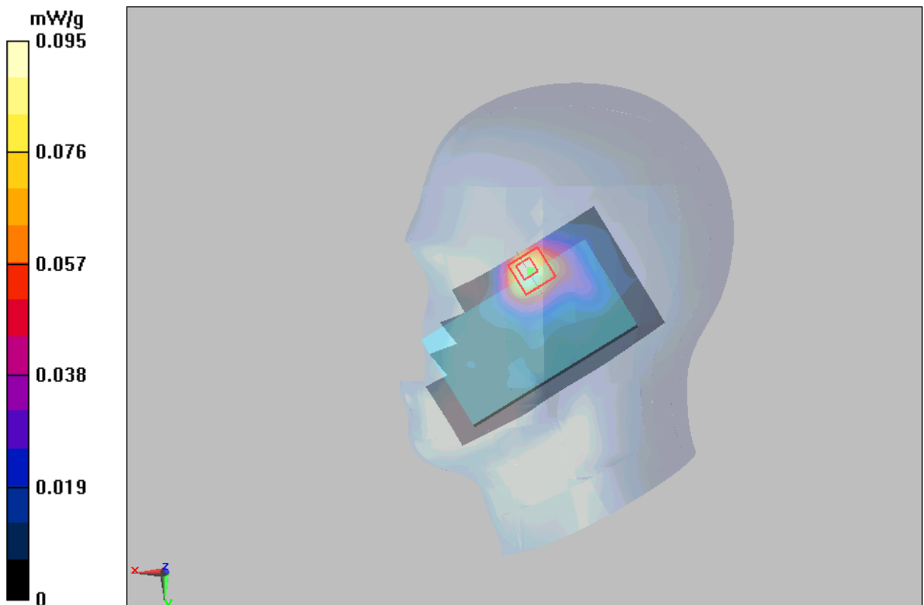
Figure 49 Right Hand Touch Cheek 802.11b Channel 1
