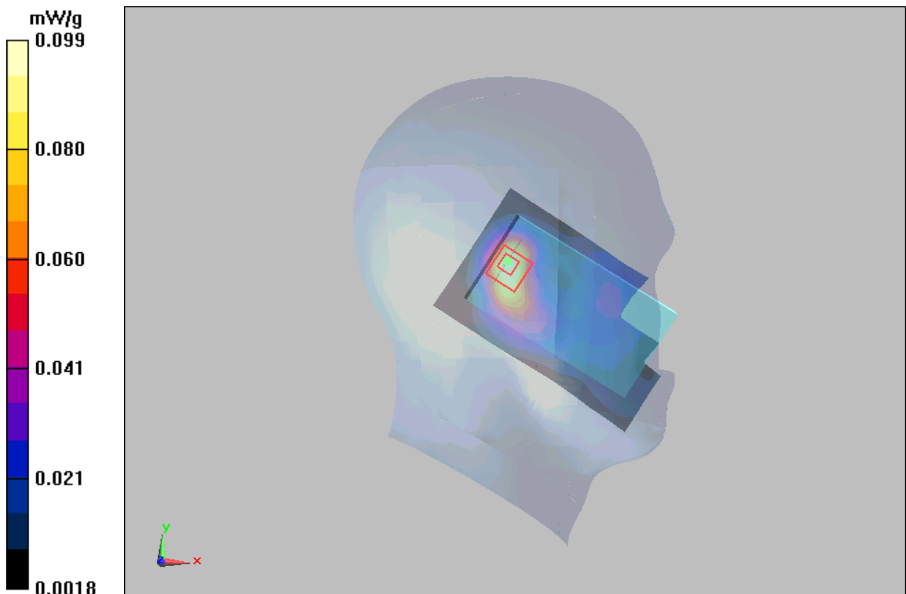
Figure 32 Left Hand Tilt 15° GSM 1900 Channel 661
