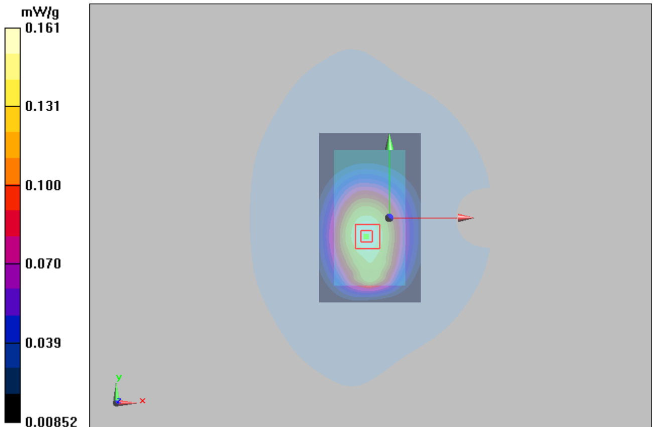
Figure 19 Body, Back Side, GSM 850 Channel 190
