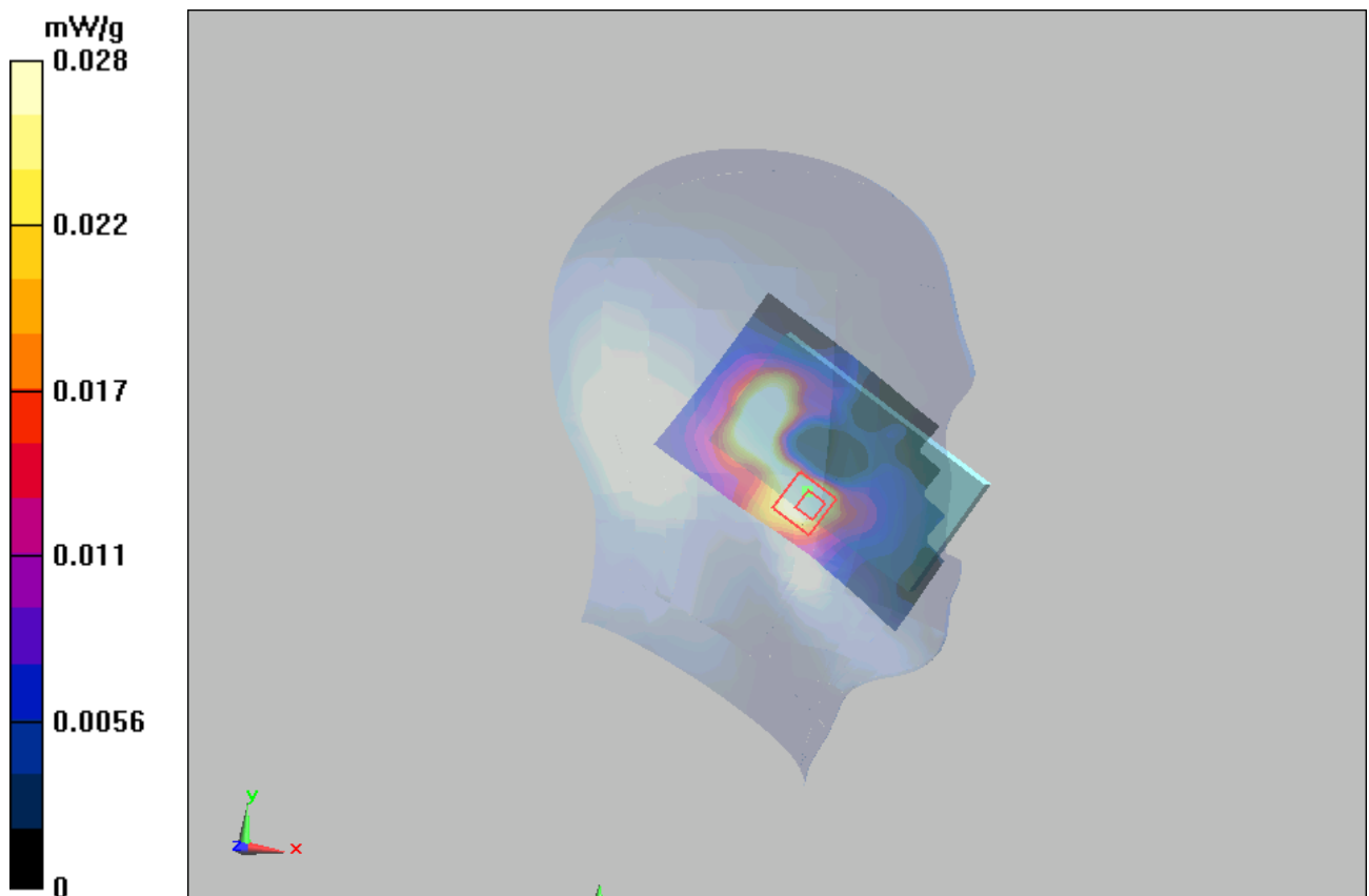
Figure 45 Left Hand Touch Cheek 802.11b Channel 6
