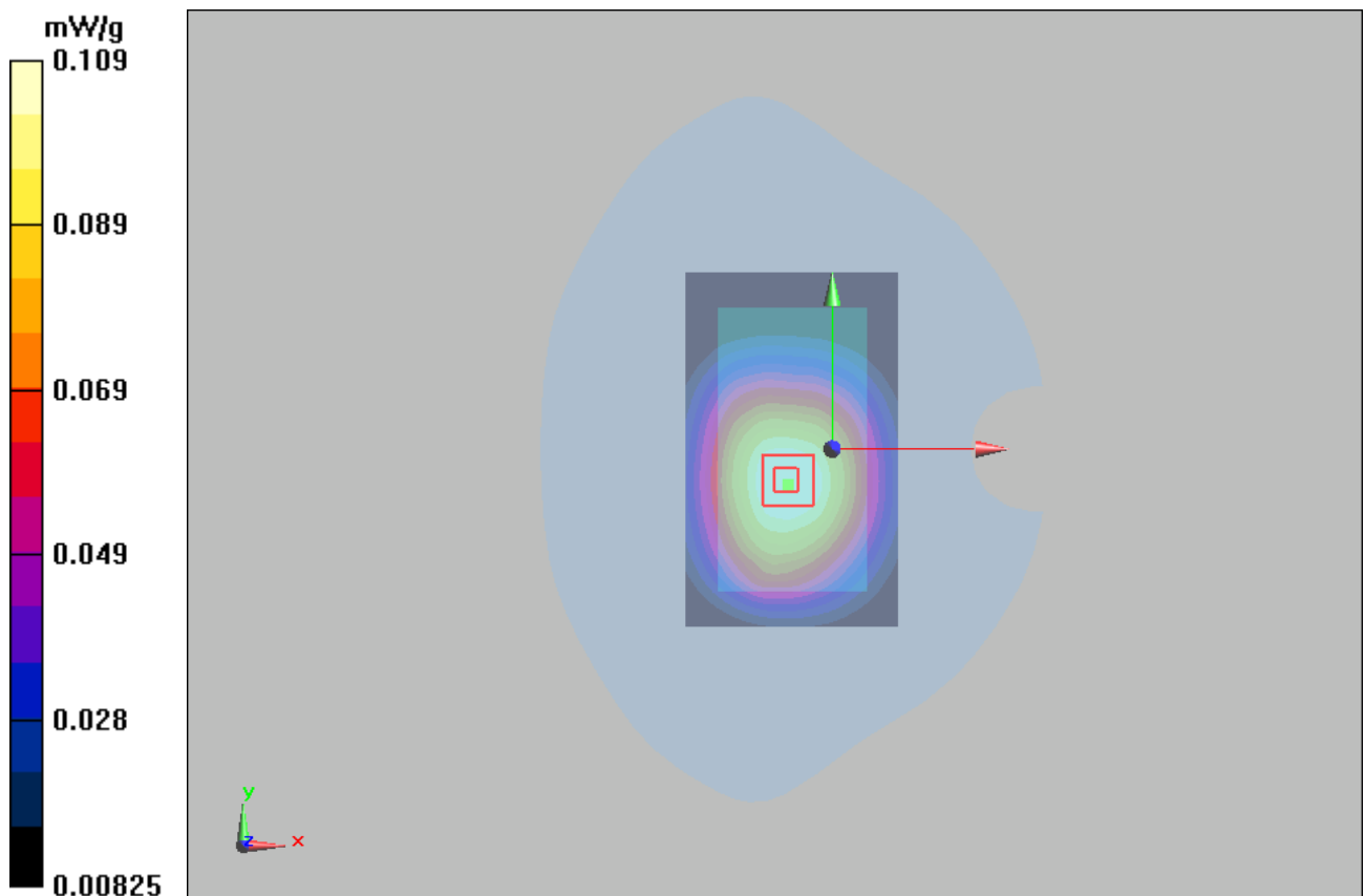
Figure 23 Body, Front Side, GSM 850 GPRS (2Txslots) Channel 190
