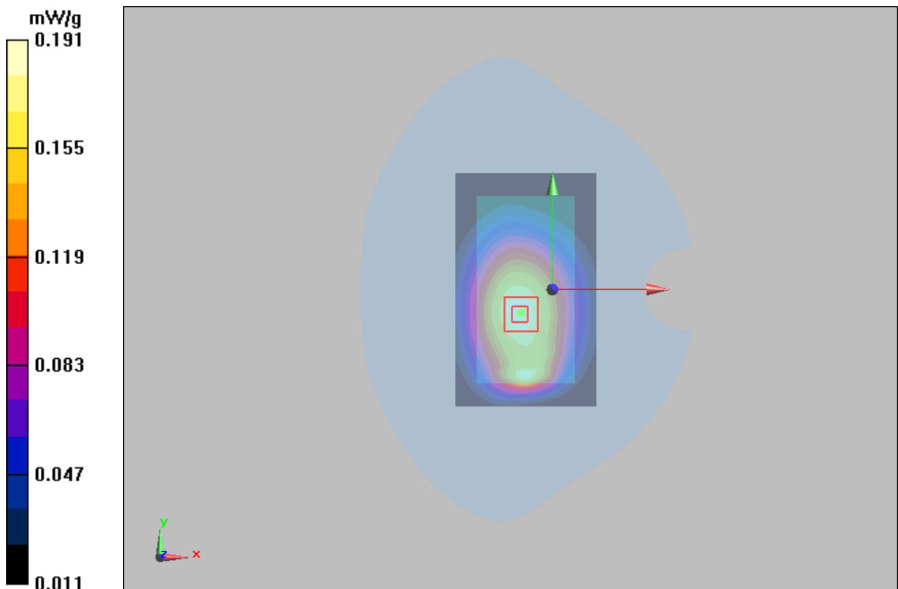
Figure 27 Body with Earphone, Back Side, GSM 850 Channel 251
