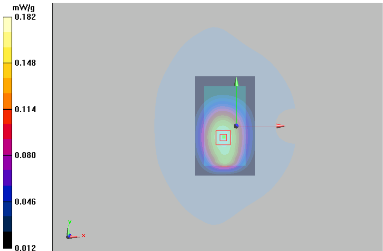
Figure 22 Body, Back Side, GSM 850 GPRS (2Txslots) Channel 128
