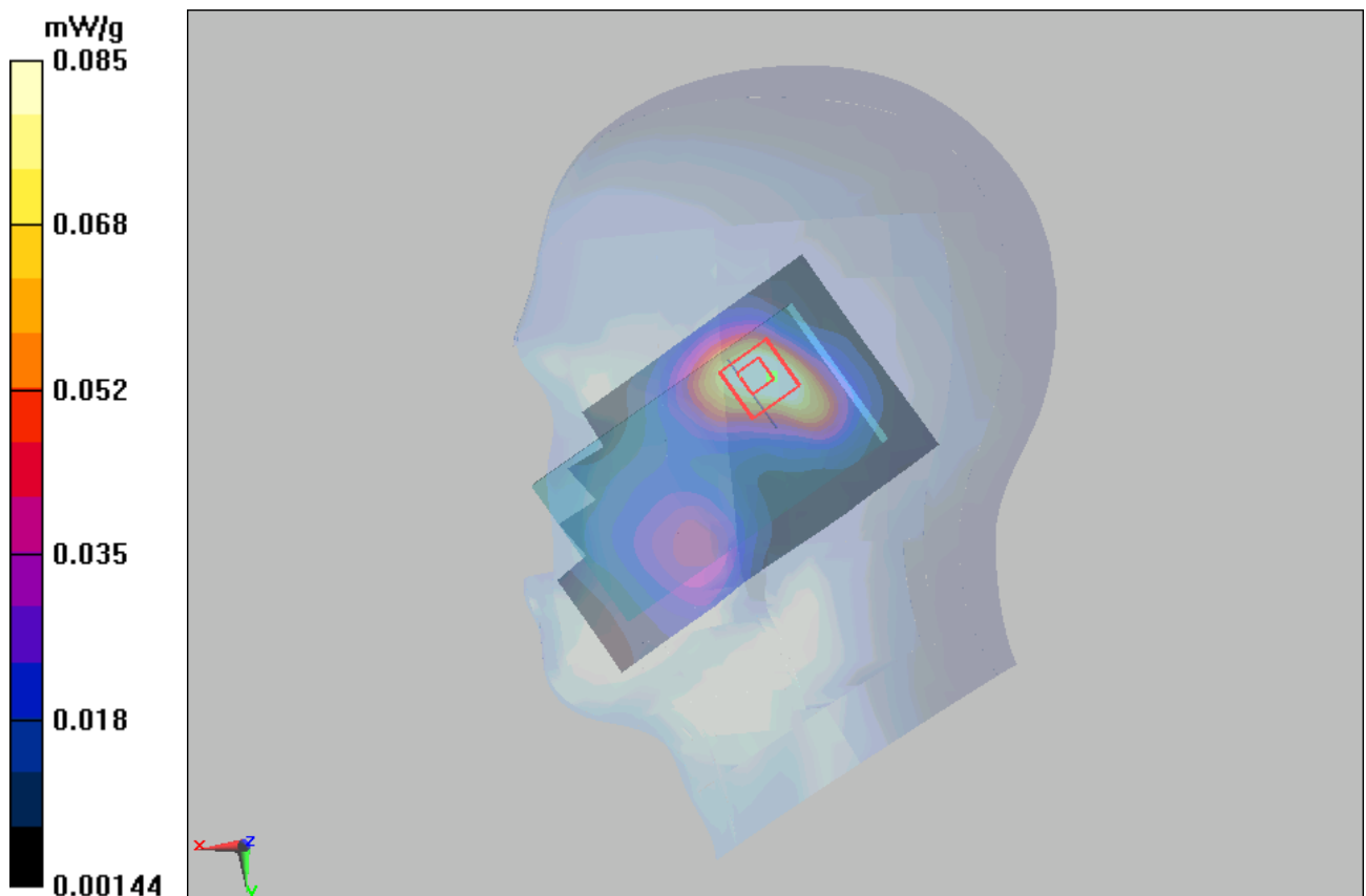
Figure 34 Right Hand Tilt 15° GSM 1900 Channel 661
