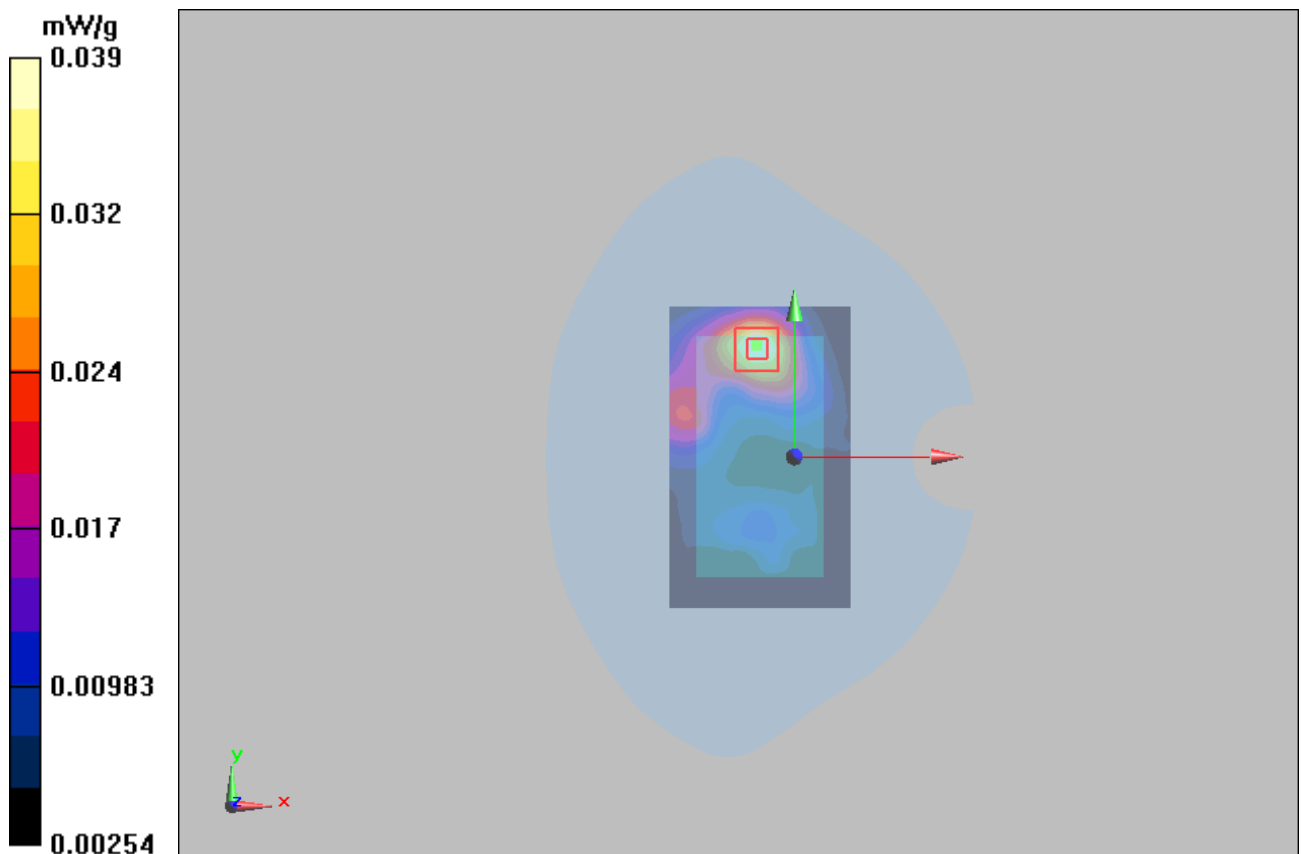
Figure 54 Body, Front Side, 802.11b Channel 6
