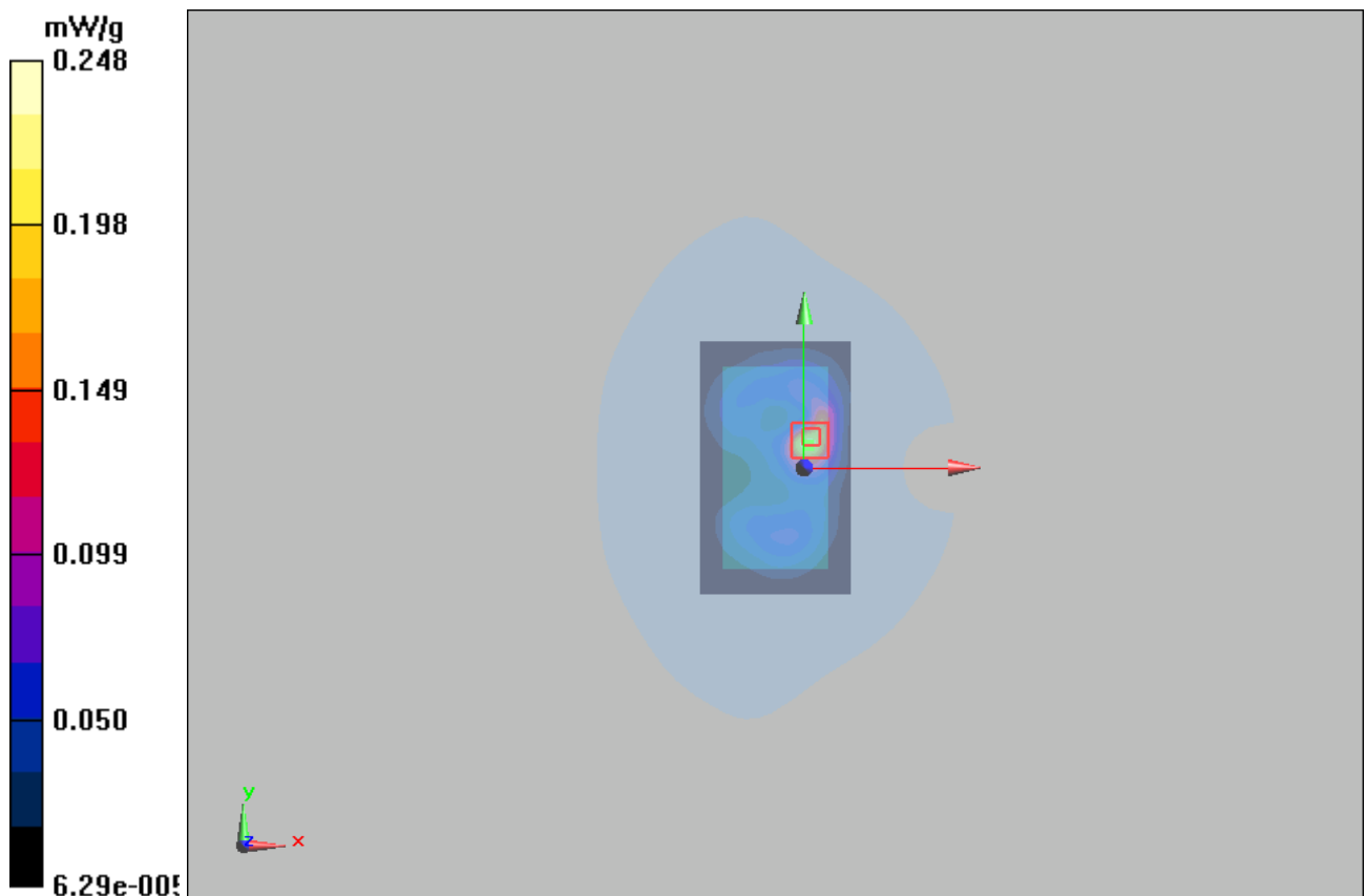
Figure 53 Body, Back Side, 802.11b Channel 1
