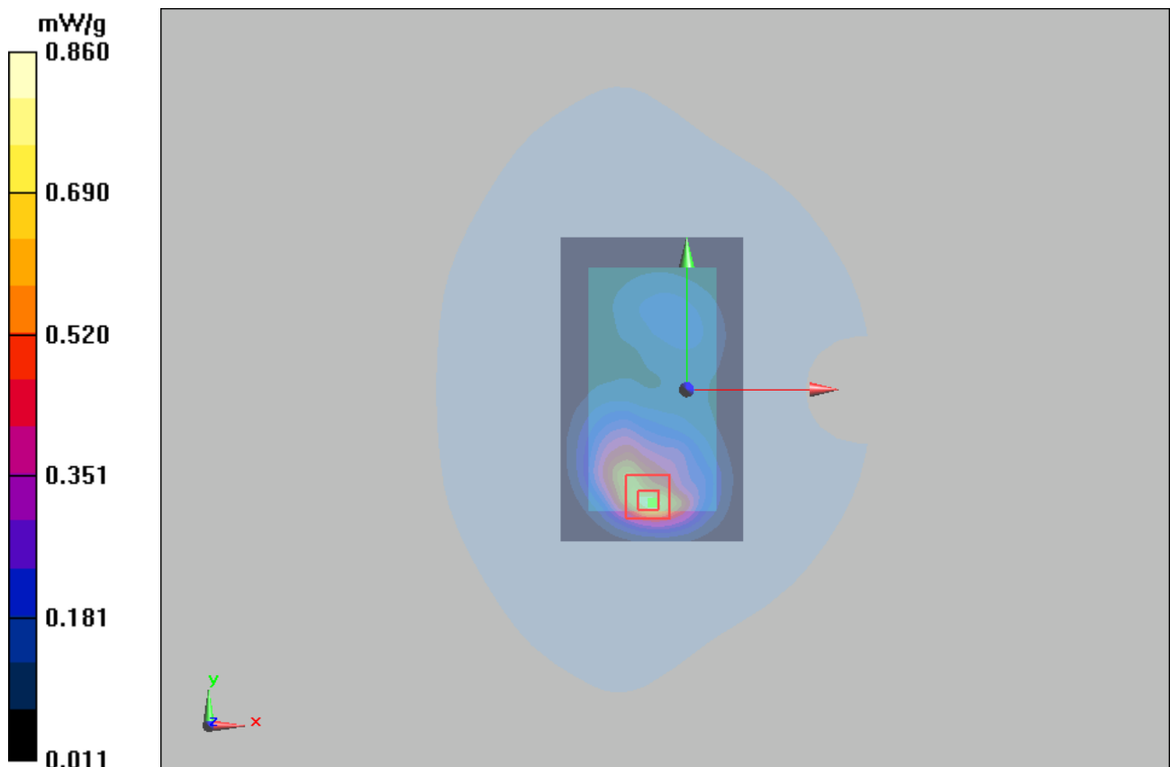
Figure 38 Body, Back Side, GSM 1900 GPRS (2Txslots) Channel 512
