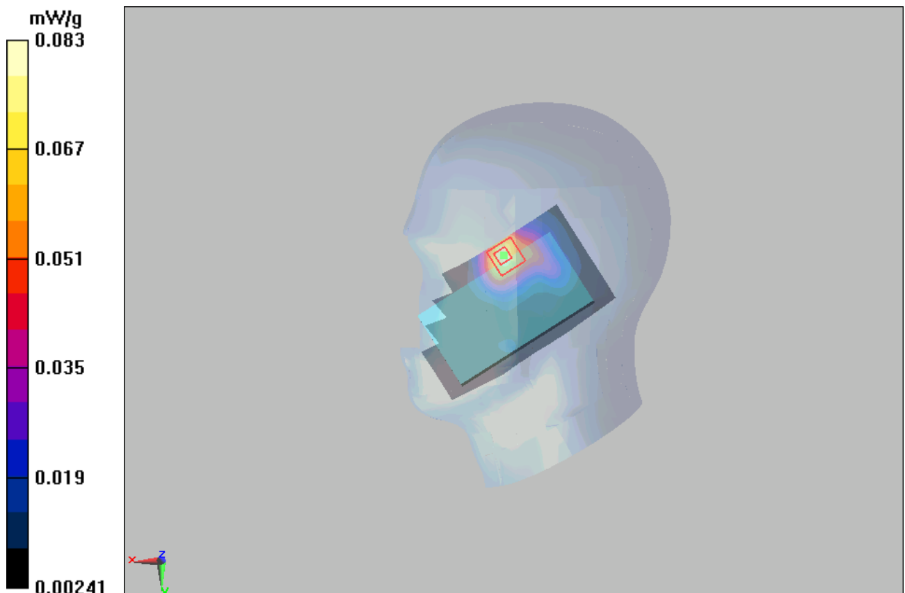
Figure 48 Right Hand Touch Cheek 802.11b Channel 6
