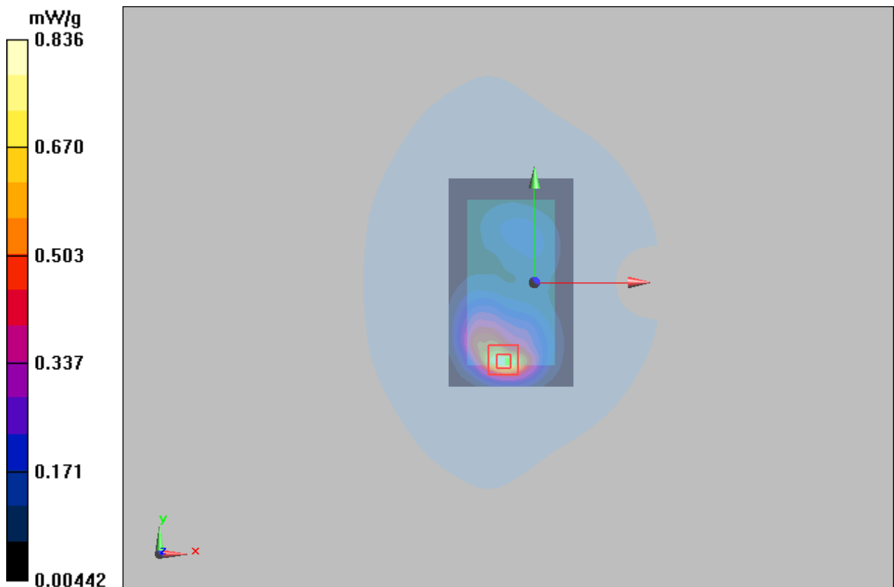
Figure 37 Body, Back Side, GSM 1900 GPRS (2Txslots) Channel 661
