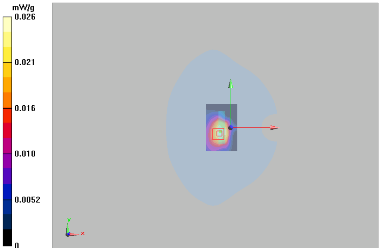
Figure 56 Body, Top Edge, 802.11b Channel 6
