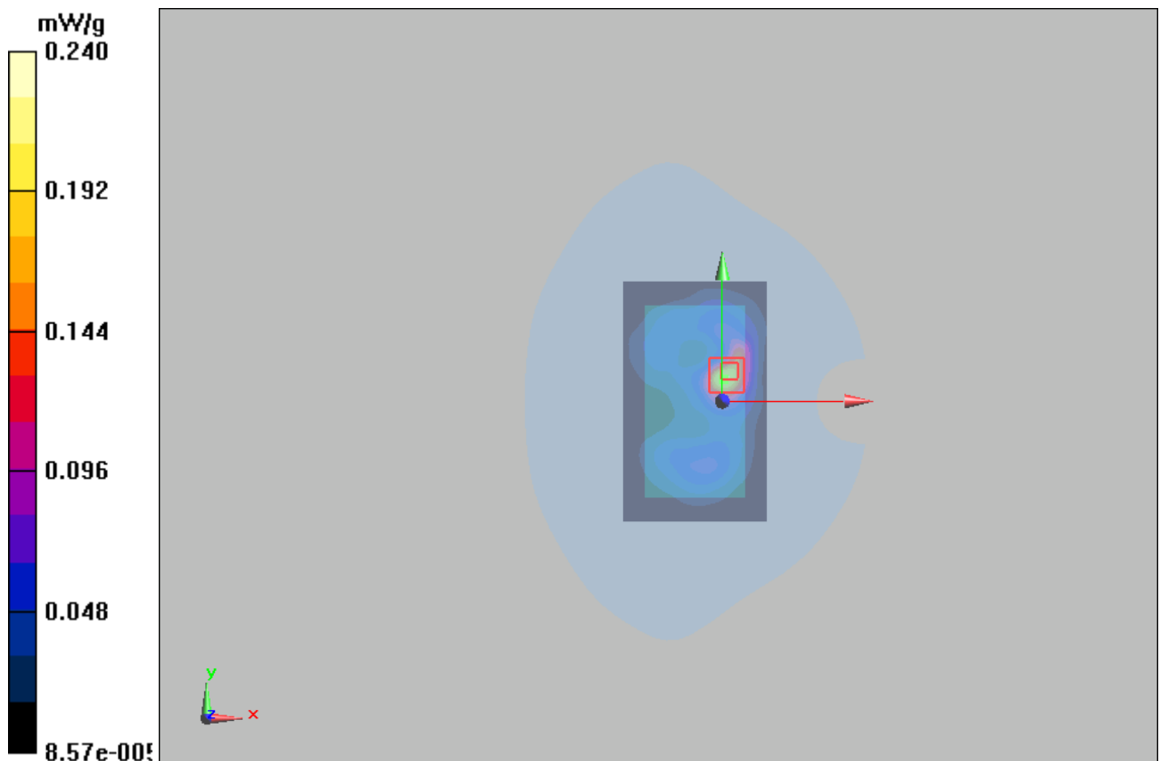
Figure 57 Body with earphone, Back Side, 802.11b Channel 6
