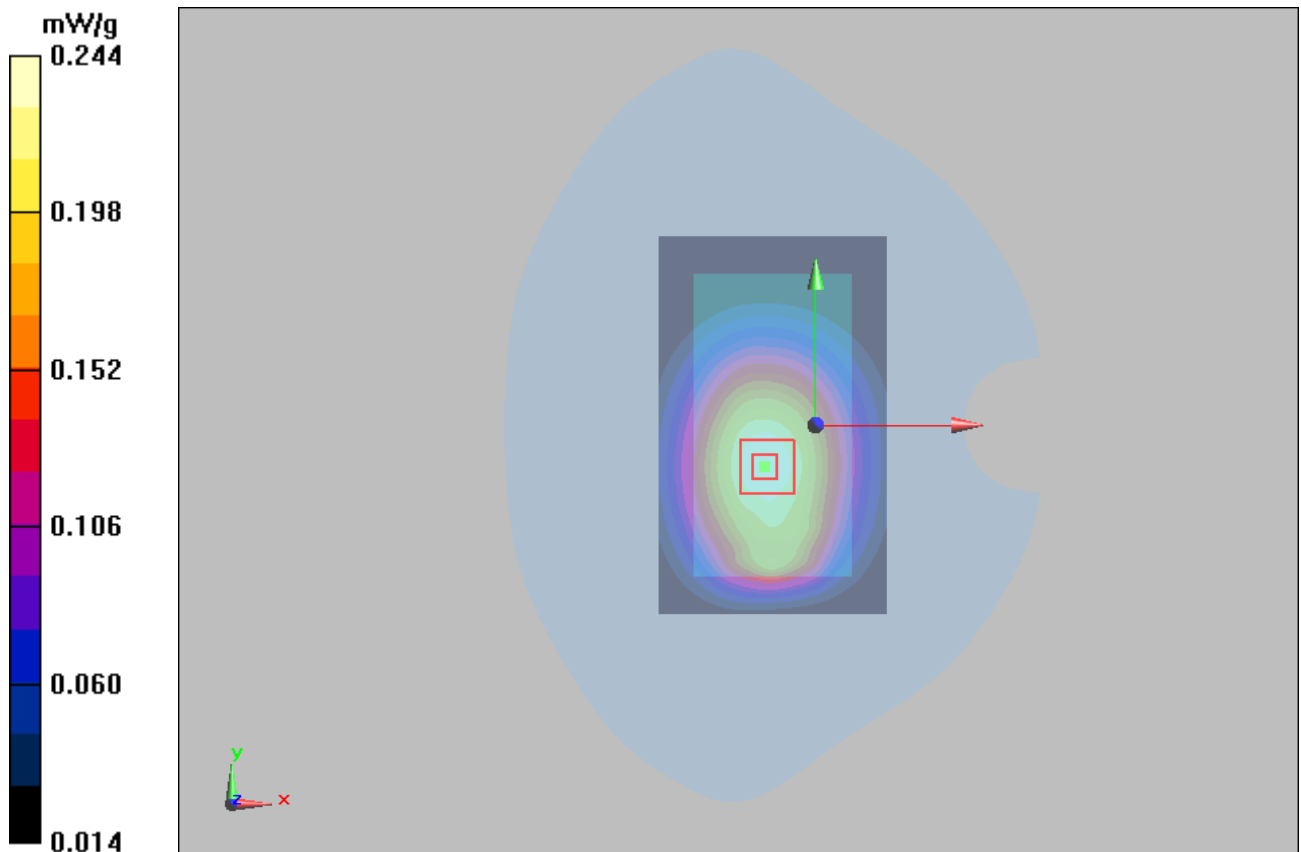
Figure 21 Body, Back Side, GSM 850 GPRS (2Txslots) Channel 190
