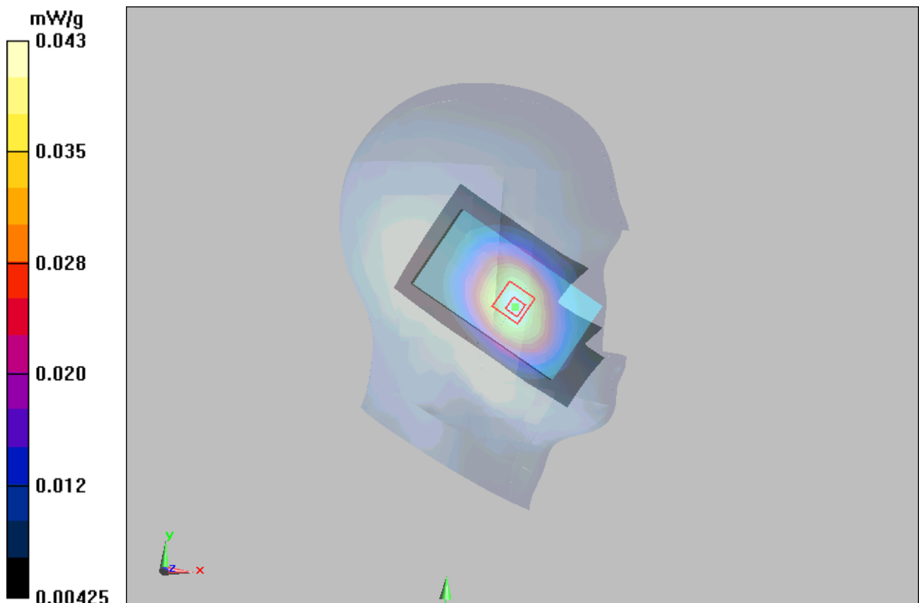
Figure 15 Left Hand Touch Cheek GSM 850 Channel 128
