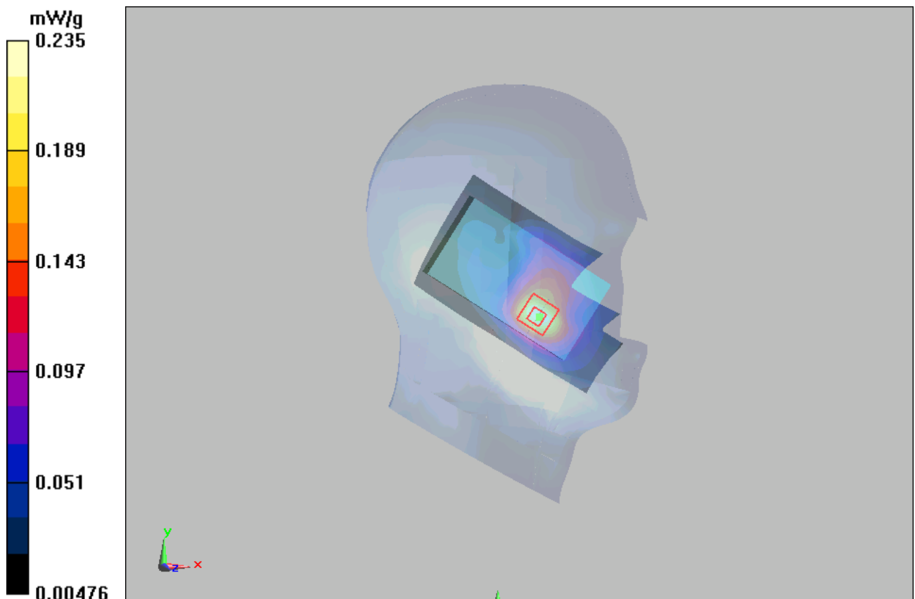
Figure 30 Left Hand Touch Cheek GSM 1900 Channel 661
