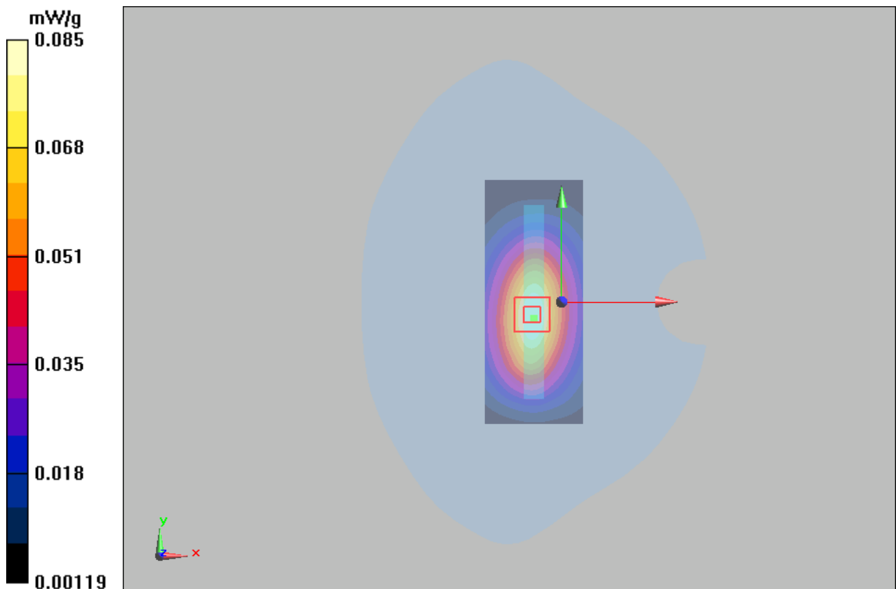
Figure 24 Body, Left Edge, GSM 850 GPRS (2Txslots) Channel 190
