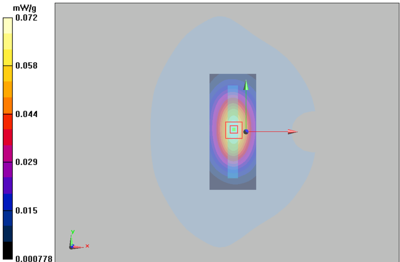
Figure 25 Body, Right Edge, GSM 850 GPRS (2Txslots) Channel 190
