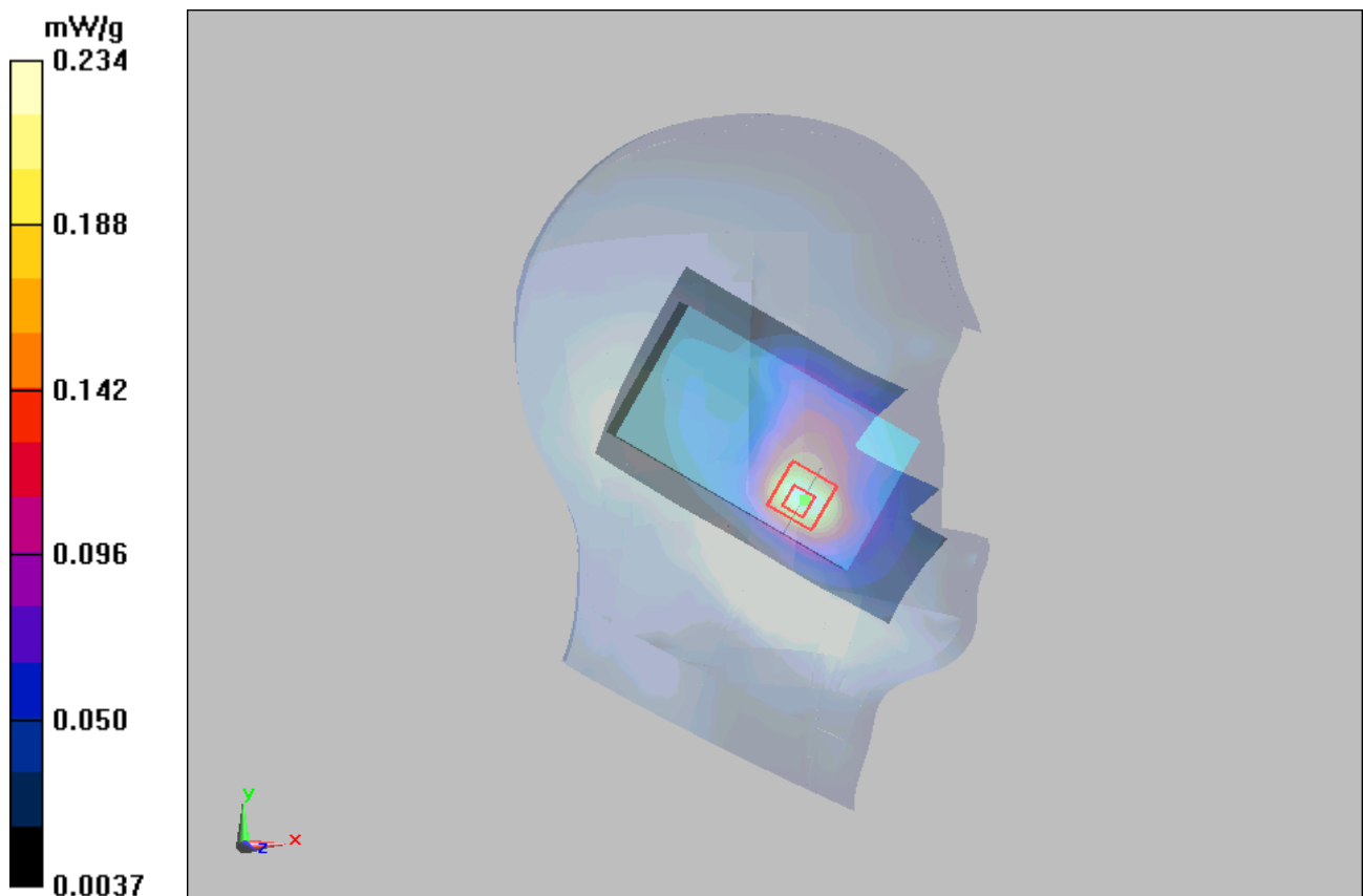
Figure 29 Left Hand Touch Cheek GSM 1900 Channel 810
