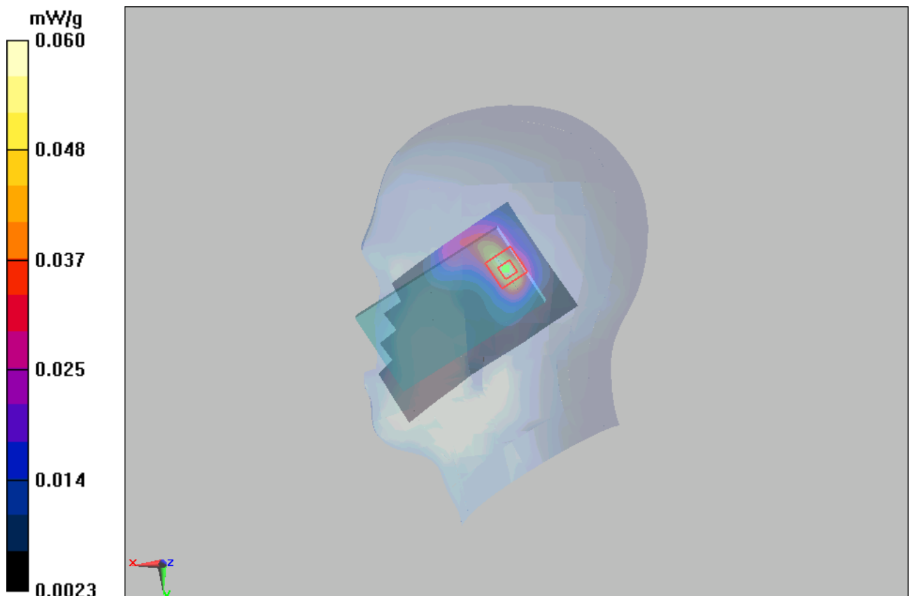
Figure 50 Right Hand Tilt 15° 802.11b Channel 6
