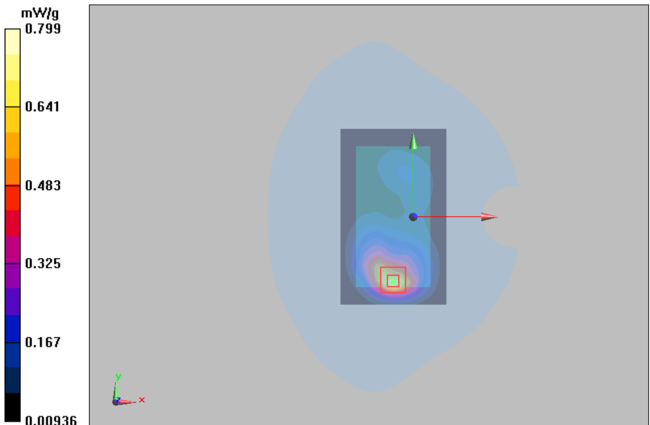
Figure 43 Body with Earphone, Back Side, GSM 1900 Channel 810
