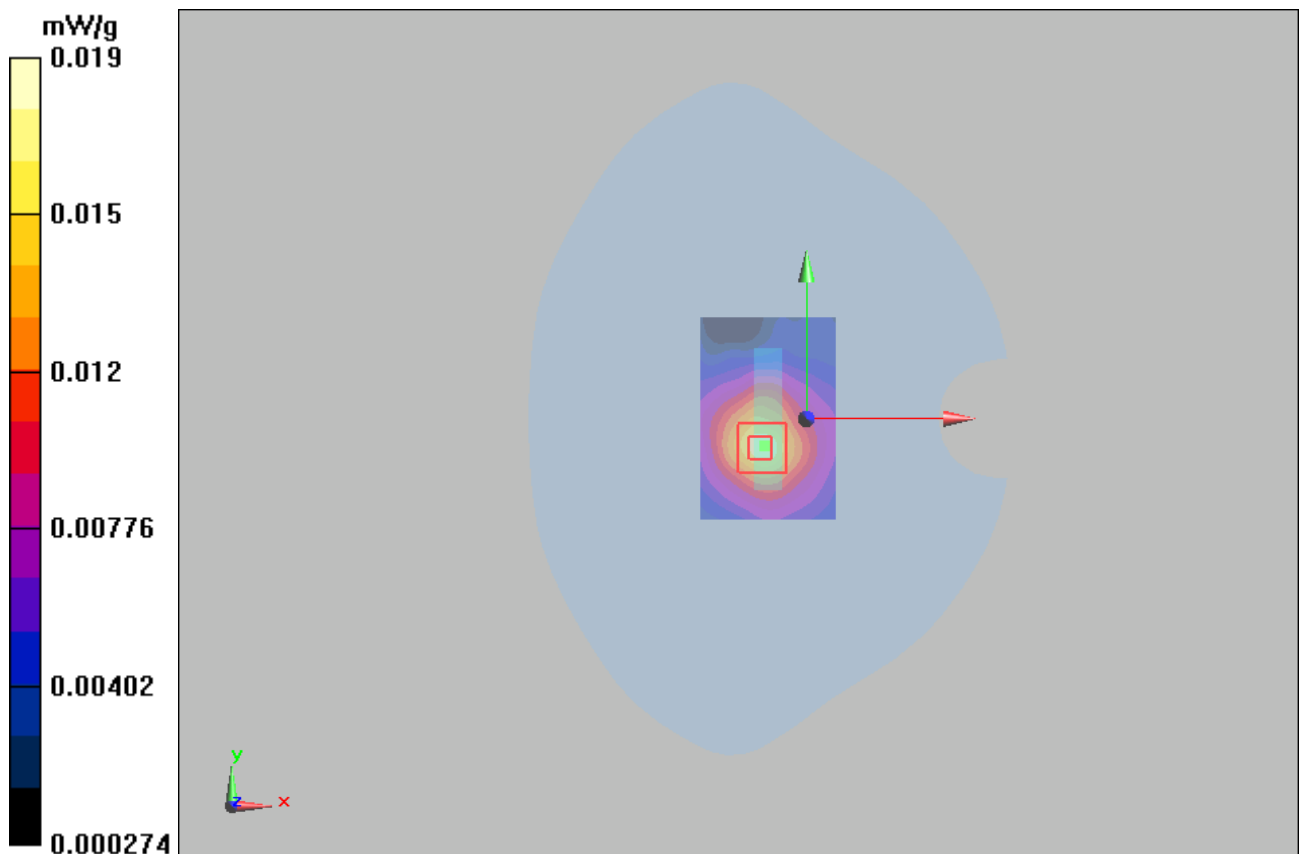
Figure 26 Body, Bottom Edge, GSM 850 GPRS (2Txslots) Channel 190
