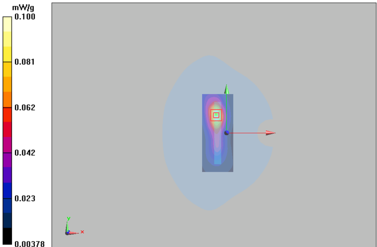
Figure 41 Body, Right Edge, GSM 1900 GPRS (2Txslots) Channel 661
