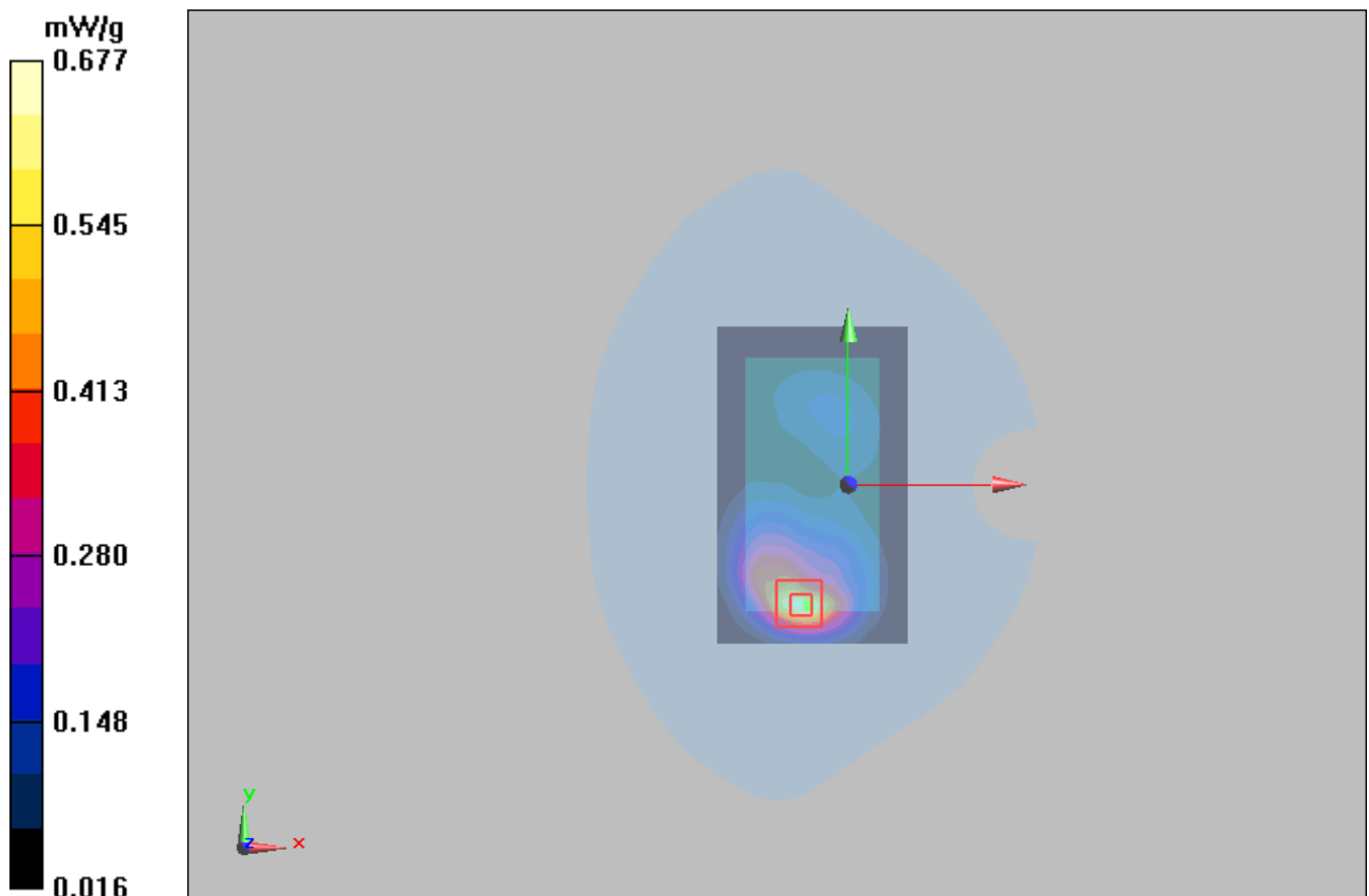
Figure 35 Body, Back Side, GSM 1900 Channel 661
