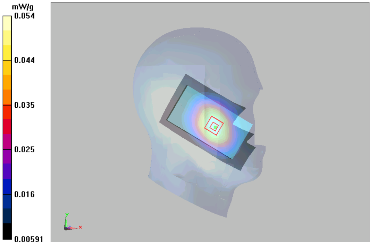
Figure 14 Left Hand Touch Cheek GSM 850 Channel 190
