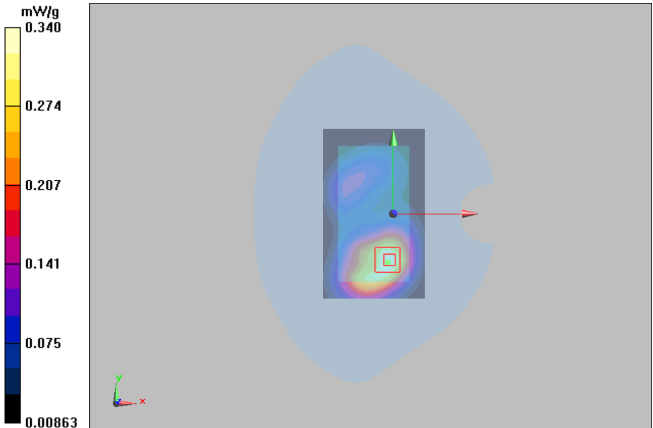
Figure 39 Body, Front Side, GSM 1900 GPRS (2Txslots) Channel 661
