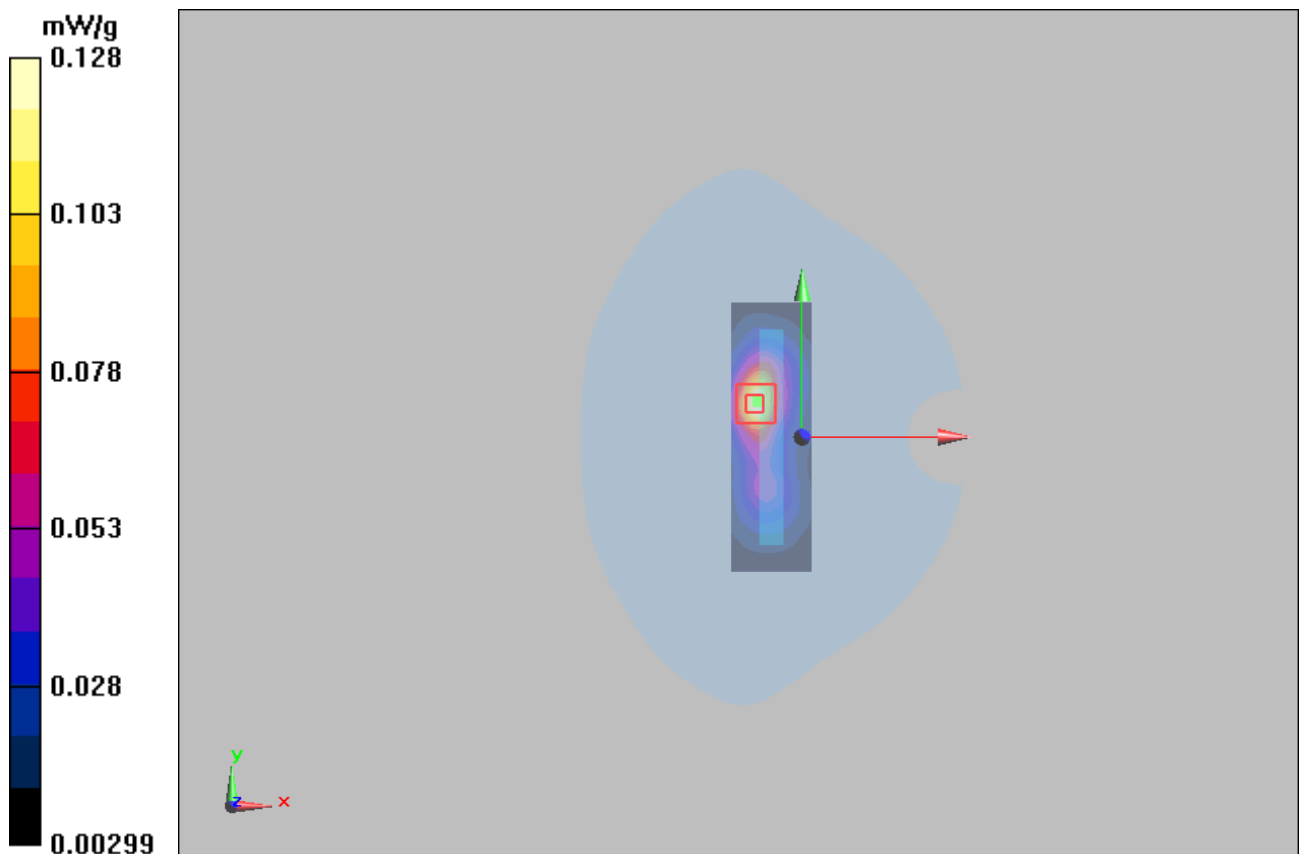
Figure 55 Body, Left Edge, 802.11b Channel 6
