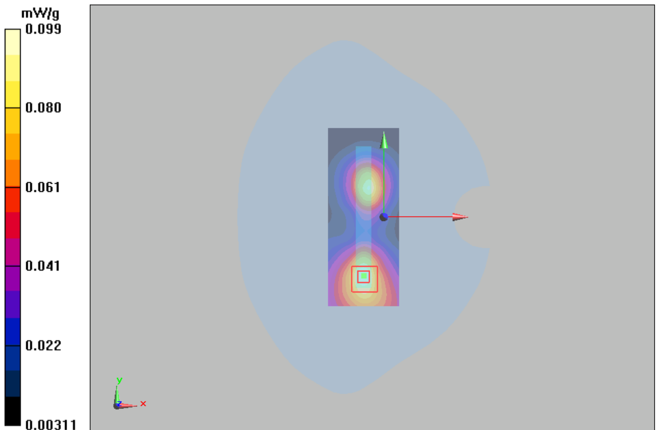
Figure 40 Body, Left Edge, GSM 1900 GPRS (2Txslots) Channel 661
