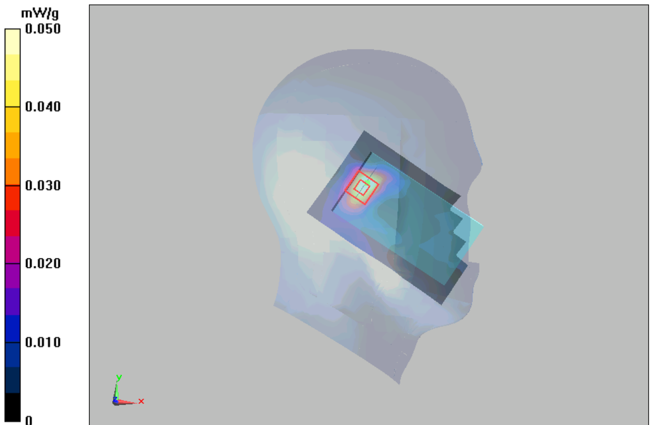
Figure 46 Left Hand Tilt 15° 802.11b Channel 6
