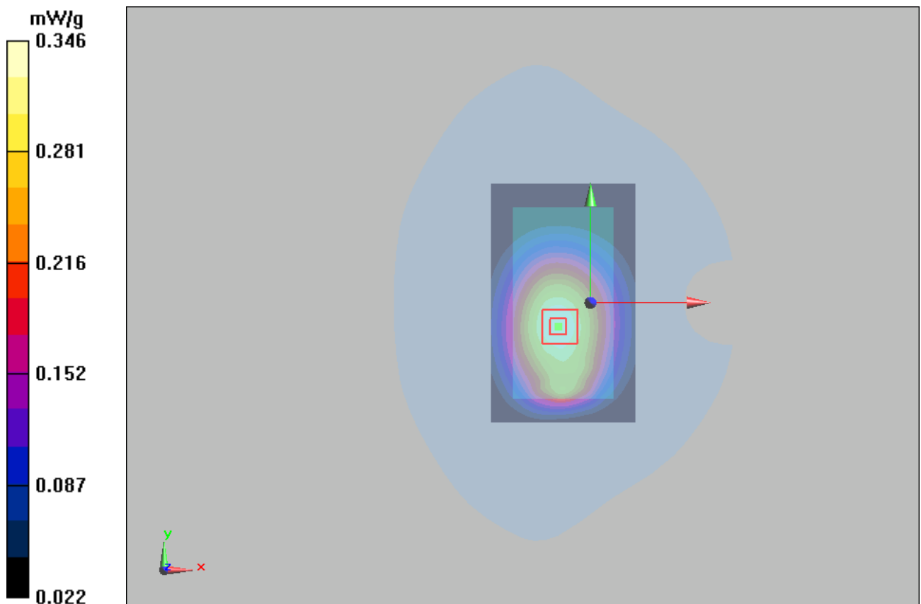
Figure 28 Body, Back Side, GSM 850 EGPRS (2Txslots) Channel 251
