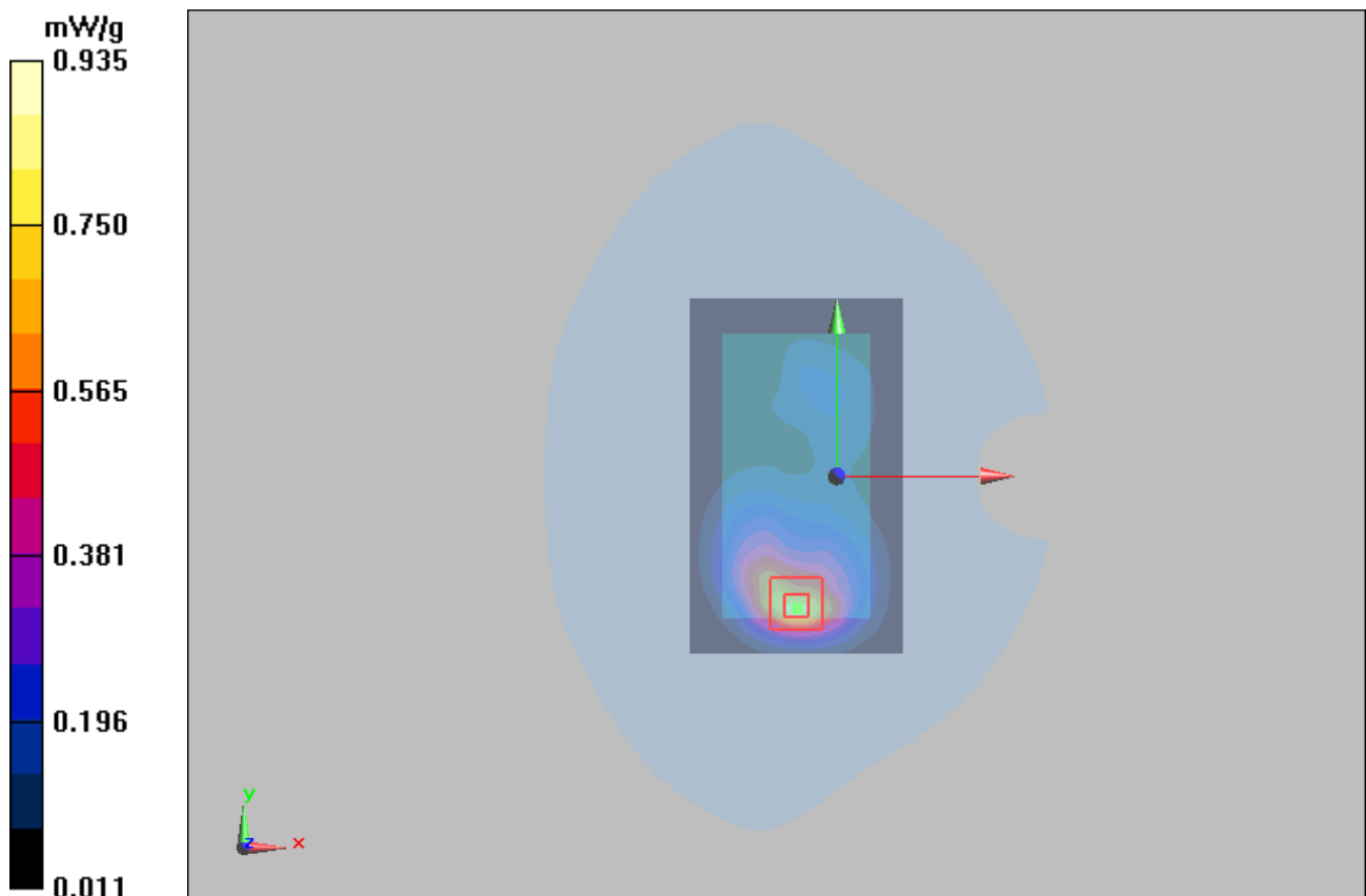
Figure 44 Body, Back Side, GSM 1900 EGPRS (2Txslots) Channel 810
