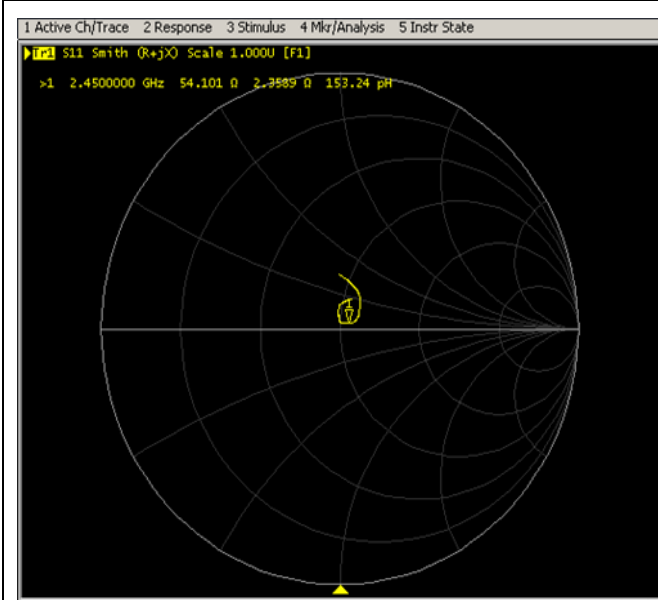
Impedance Test-Body
