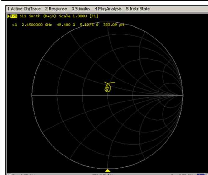
Impedance Test-Body
