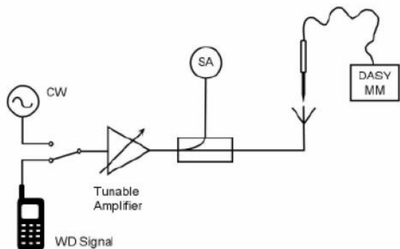
Fig. 6 Probe Modulation Factor Test Setup
