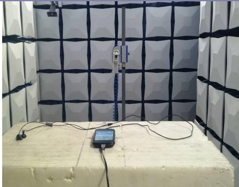
Radiated Spurious Emission (18GHz to26.5GHz)
