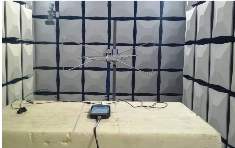
Radiated Spurious Emission (below 3GHz)
