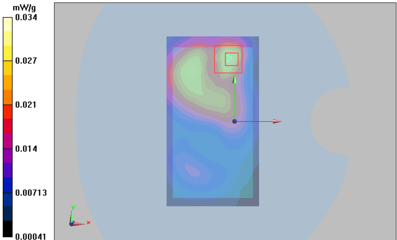
Figure 142 Body, Back Side, 802.11b Channel 11
