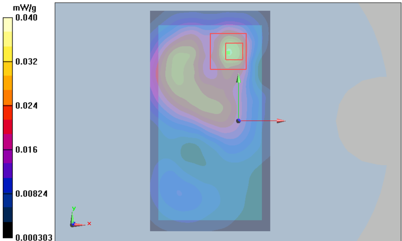
Figure 144 Body, Back Side, 802.11b Channel 11
