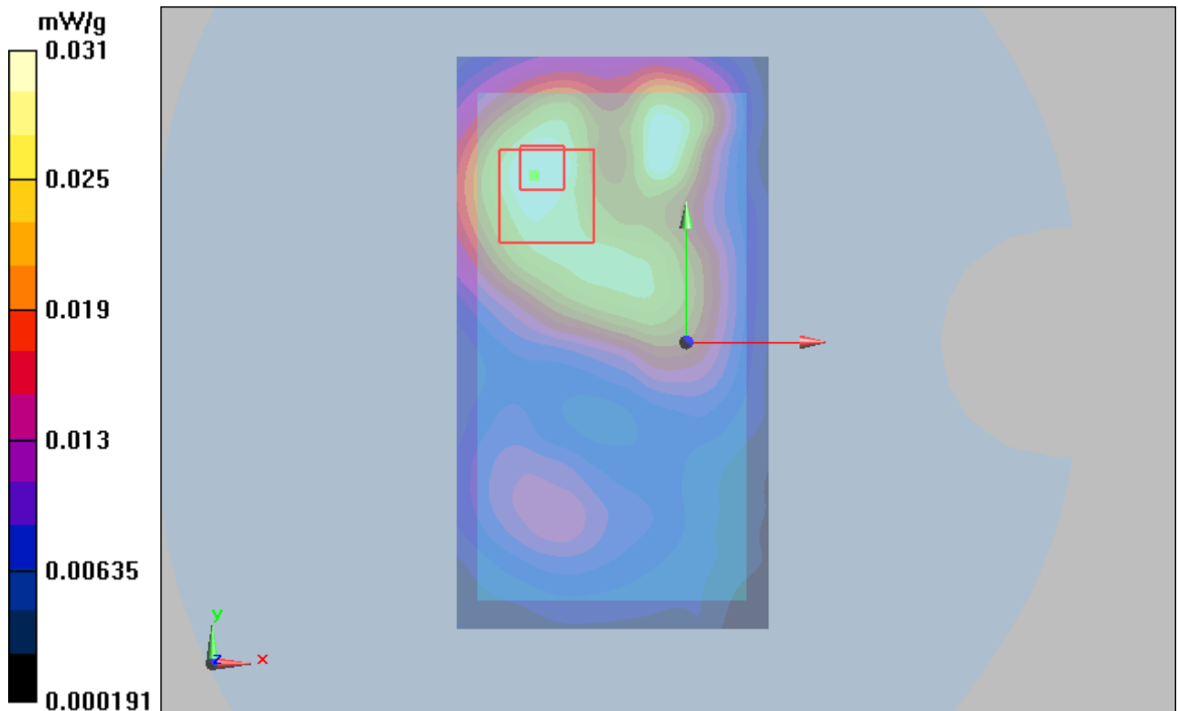
Figure 143 Body, Back Side, 802.11b Channel 11
