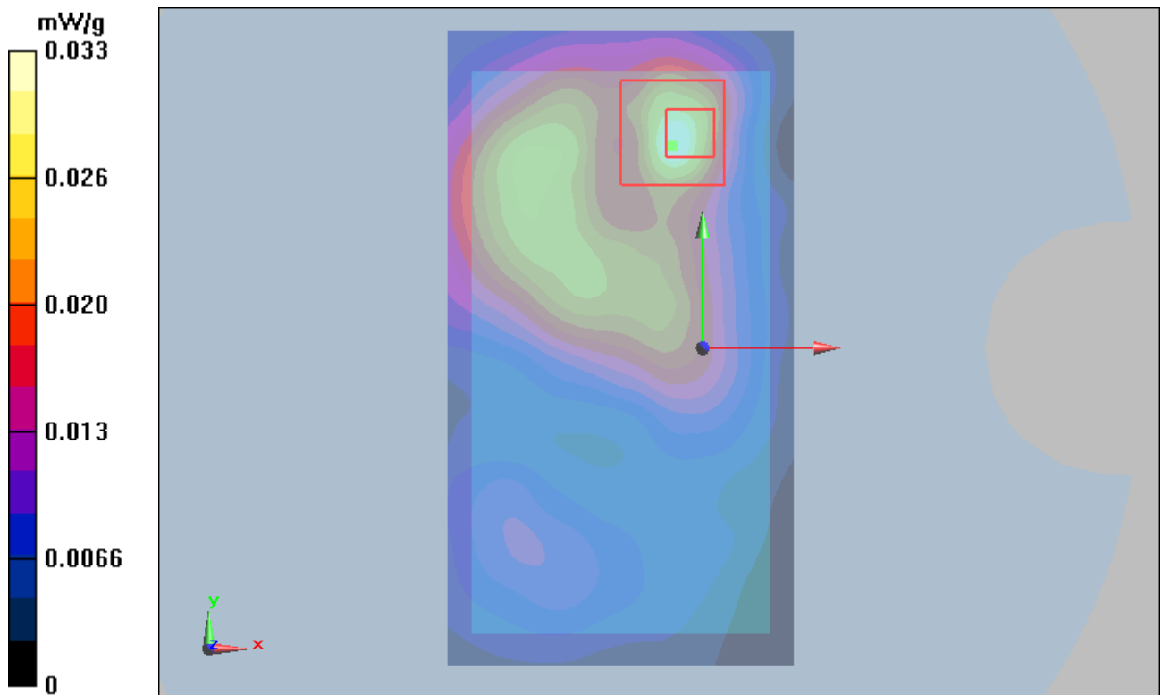
Figure 141 Body, Back Side, 802.11b Channel 11
