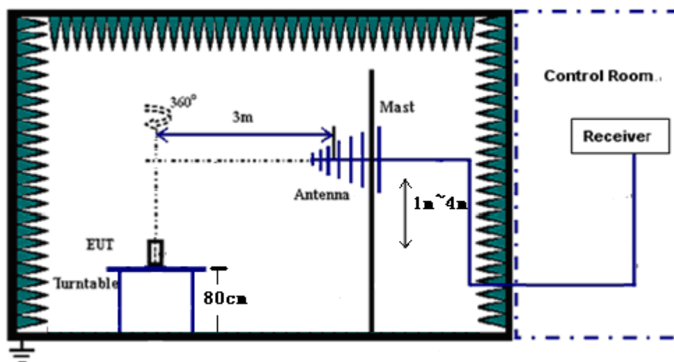
Figure 2. Test set-up
