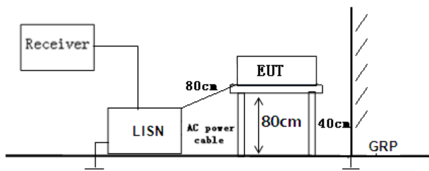
Figure 3. Test Set-up
