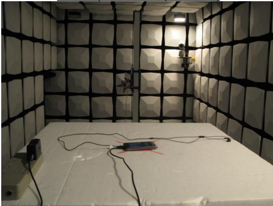
Radiated Spurious Emission (2GHz-18GHz)
