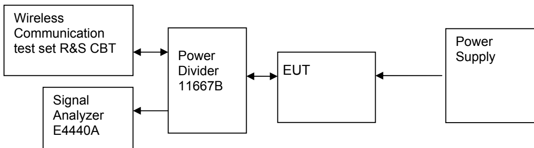
Figure 4. Test Set-up
