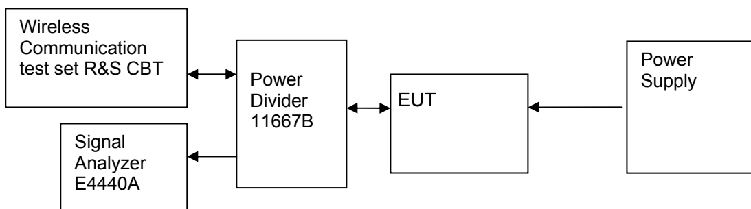
Figure 7. Test Set-up
