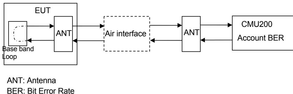
Figure 2. Test Configuration
