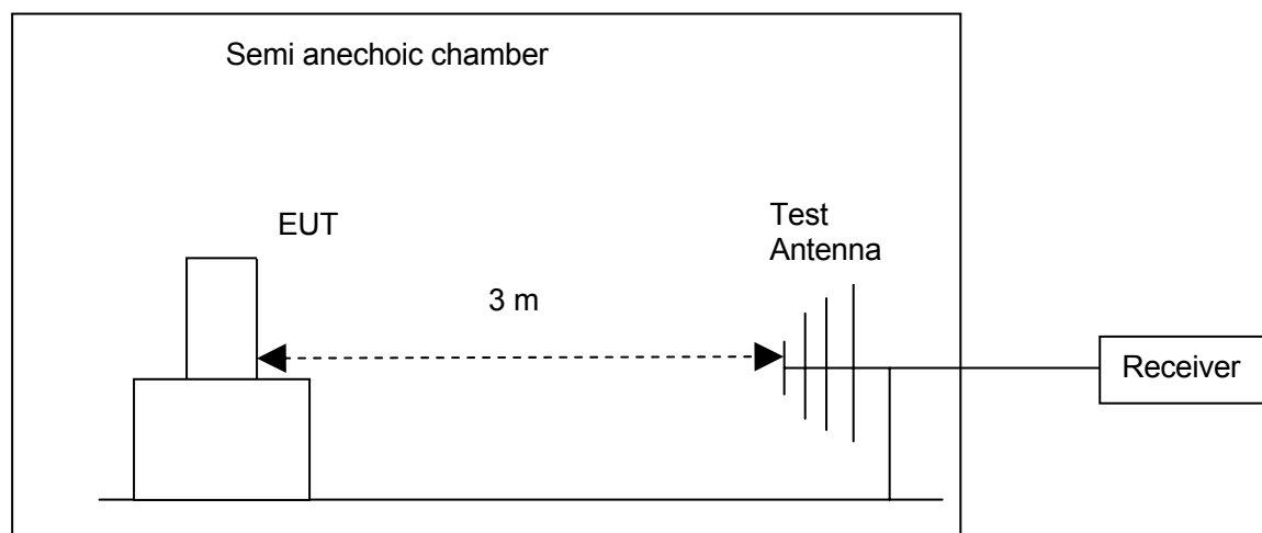
Figure 3. Test set-up
