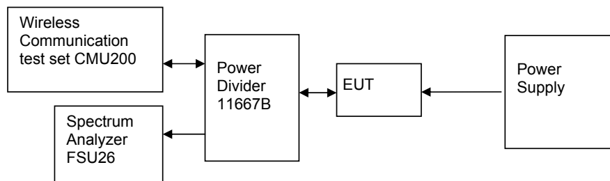
Figure 4. Test Set-up
