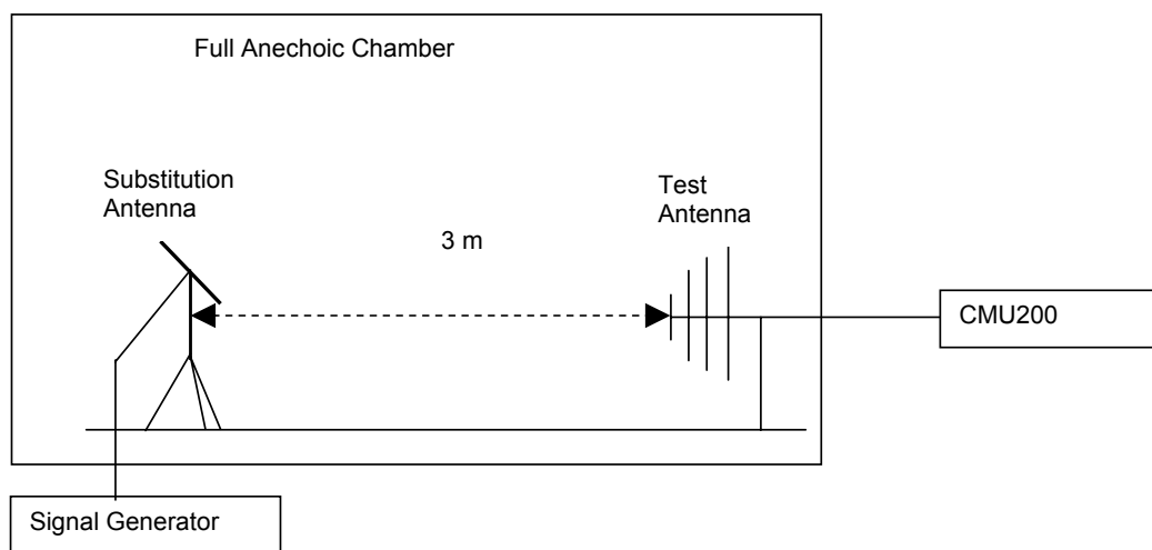
Figure 1. Test Set-up
