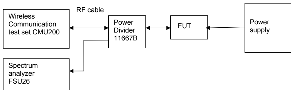
Figure 6. Test Set-up
