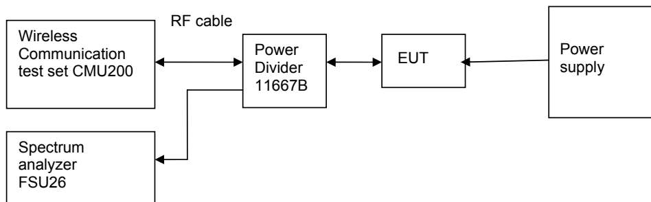
Figure 5. Test Set-up
