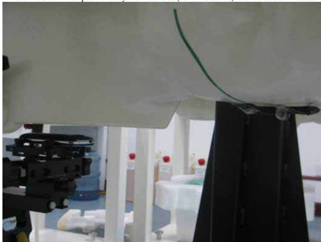
Photo 12: U7510 Test position body worn rear side (15 mm distance) with bluetooth headset
