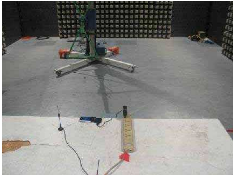
Radiated Disturbance
