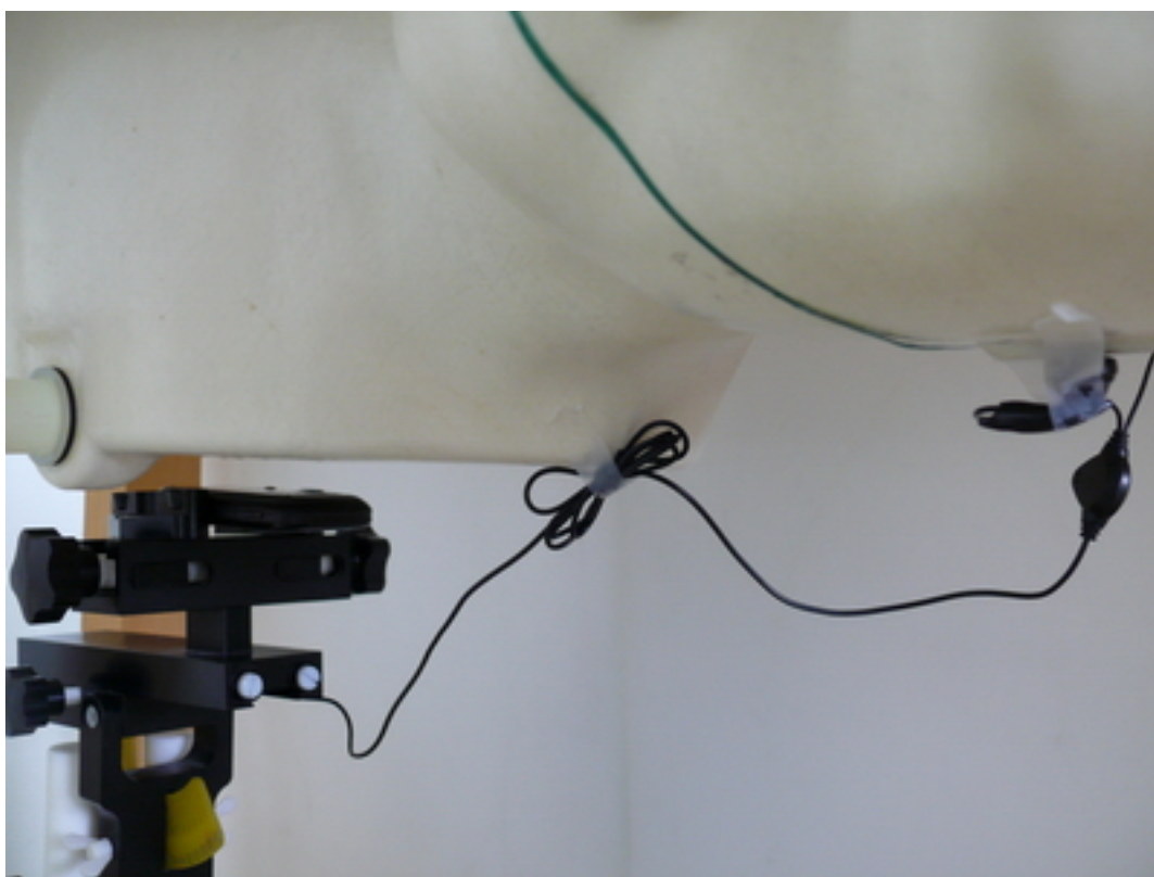
Picture 11: Body with the Earphone, towards ground, the distance from handset to the bottom of the Phantom is 15mm)
