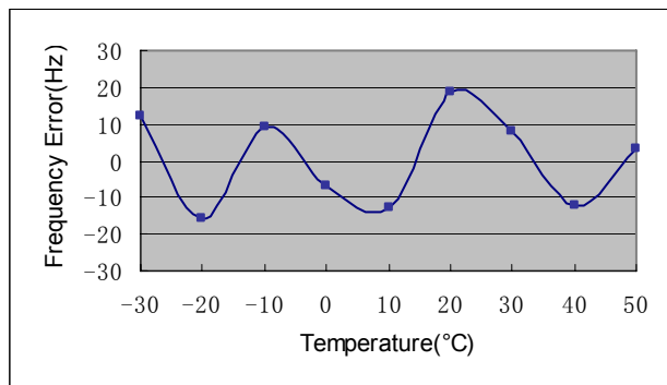
Figure 8. GPRS/GSM Mode Test Graph
