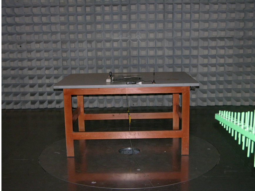
Radiated Disturbance
