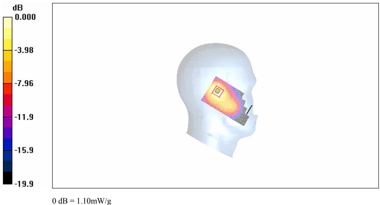
Fig. 5 Left Hand Touch Cheek PCS 1900MHz CH512
