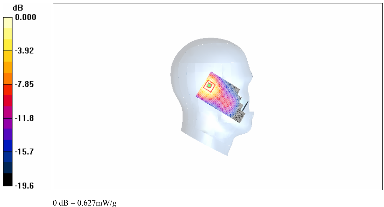
Fig. 7 Left Hand Tilt 15° PCS 1900MHz CH810
