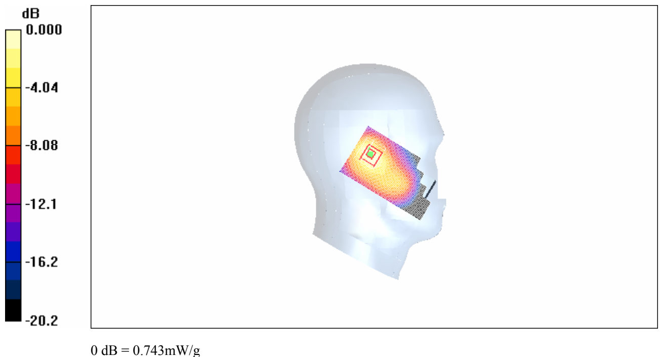
Fig. 3 Left Hand Touch Cheek PCS 1900MHz CH661
