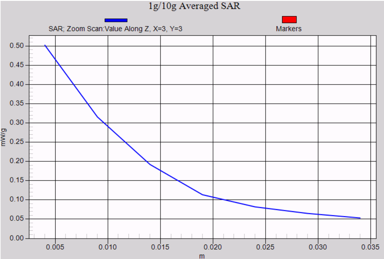
U1280 towards ground-GSM1900 GPRS 2TS Channel 810
