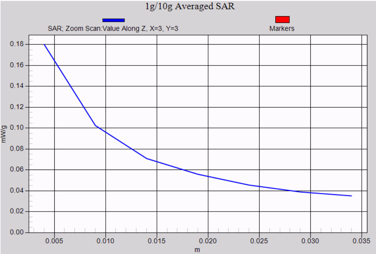
U1280 towards ground with Headset-GSM1900 GPRS 2TS Channel 810
