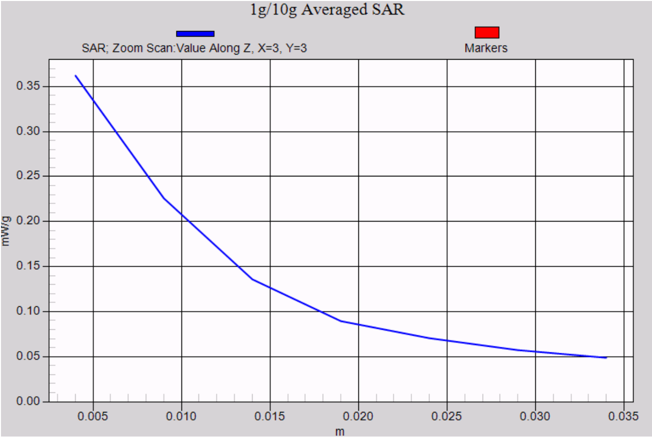
U1280 towards ground-GSM1900 GPRS 2TS Channel 661
