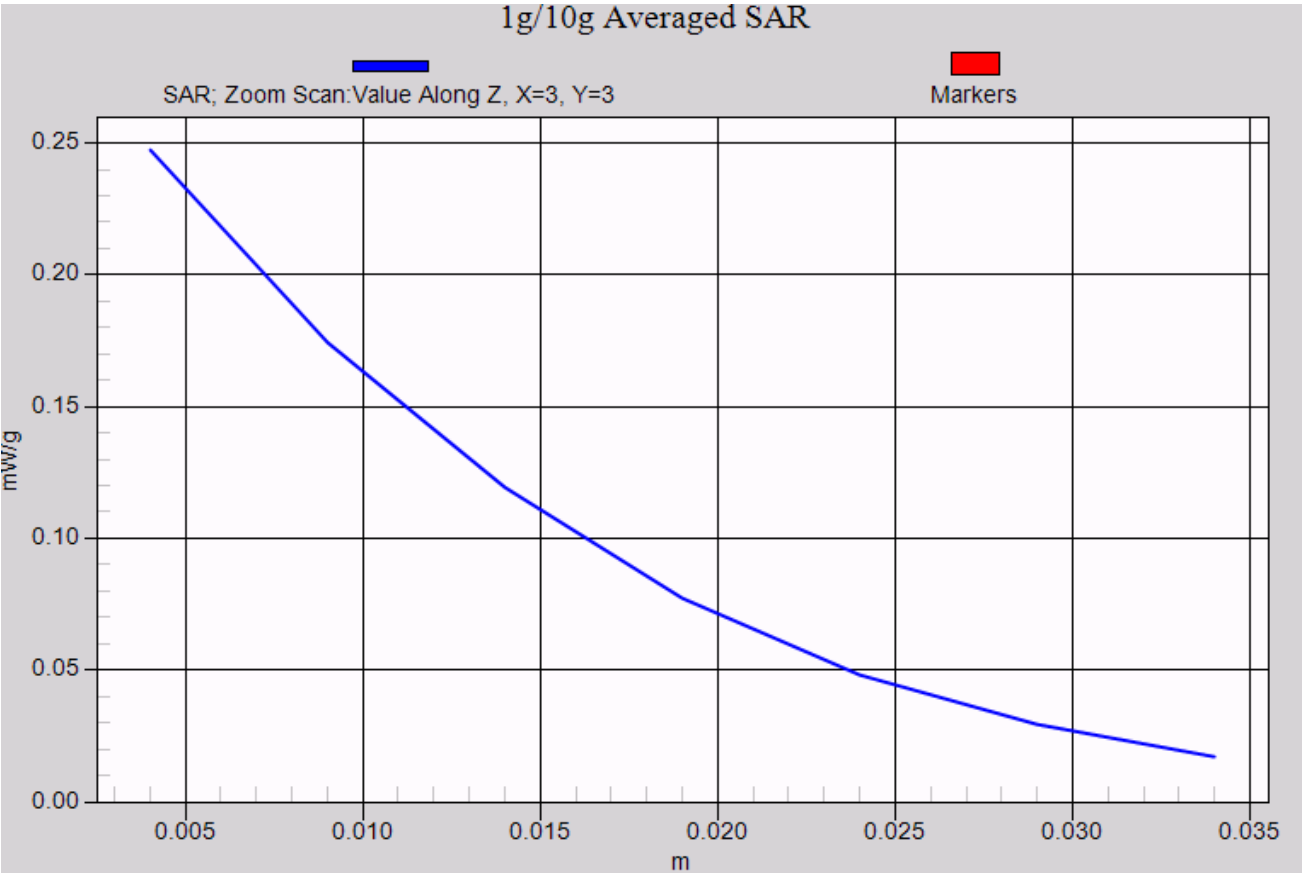
U1280 RightHandSide tilted 15°-GSM1900 Channel 661
