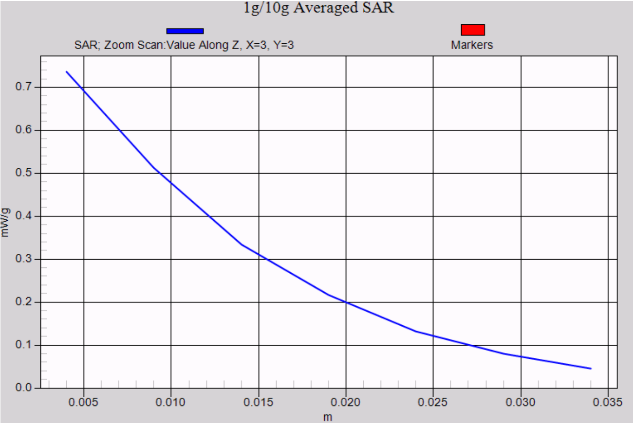
U1280 RightHandSide touched-GSM1900 Channel 810
