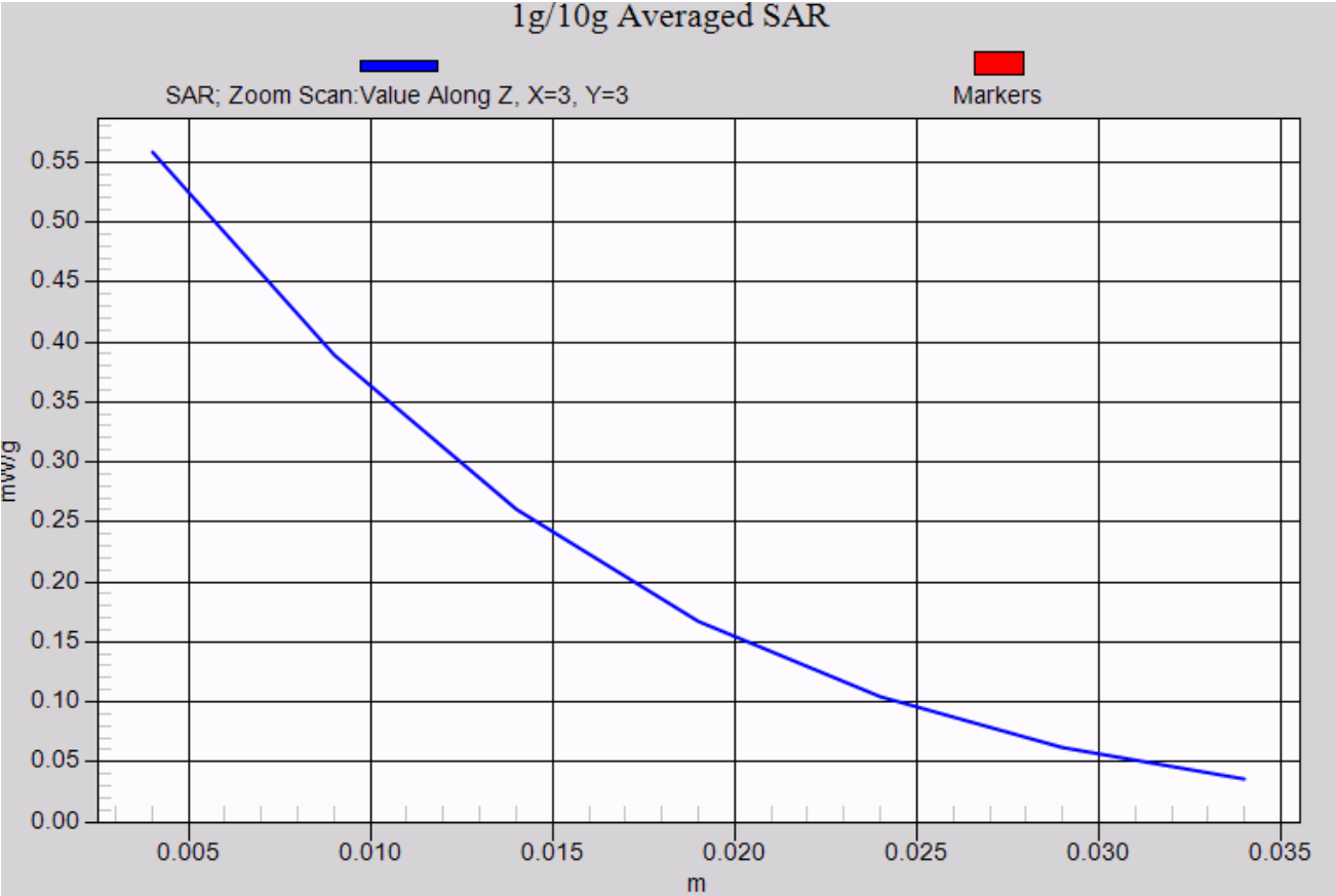
U1280 RightHandSide touched-GSM1900 Channel 661
