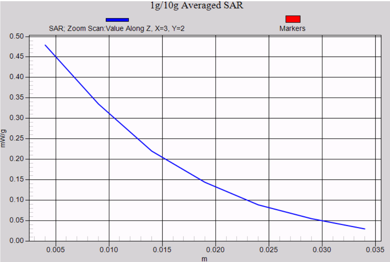
U1280 RightHandSide touched-GSM1900 Channel 512
