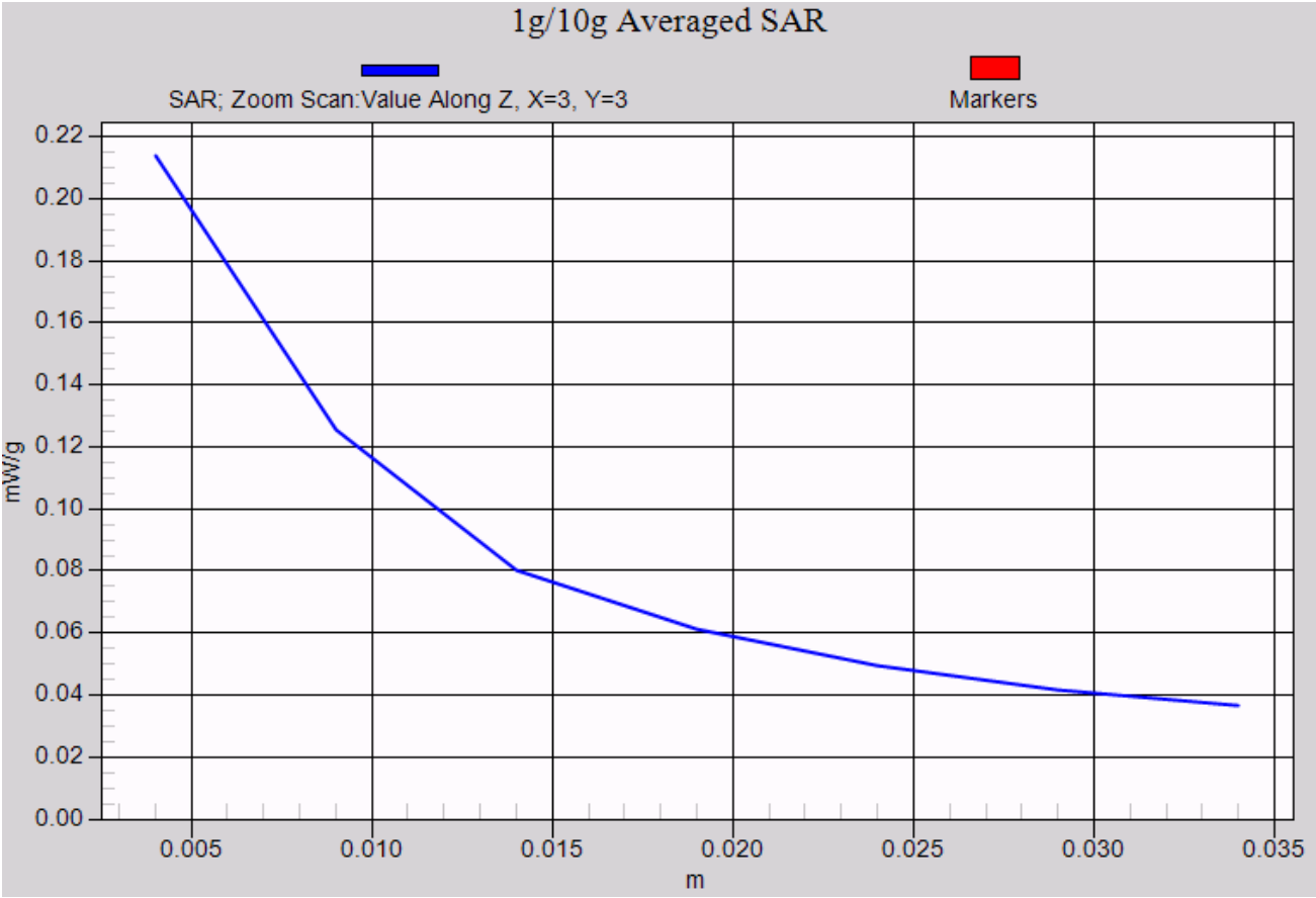
U1820 towards ground with Bluetooth Headset -GSM1900 GPRS 2TS Channel 810
