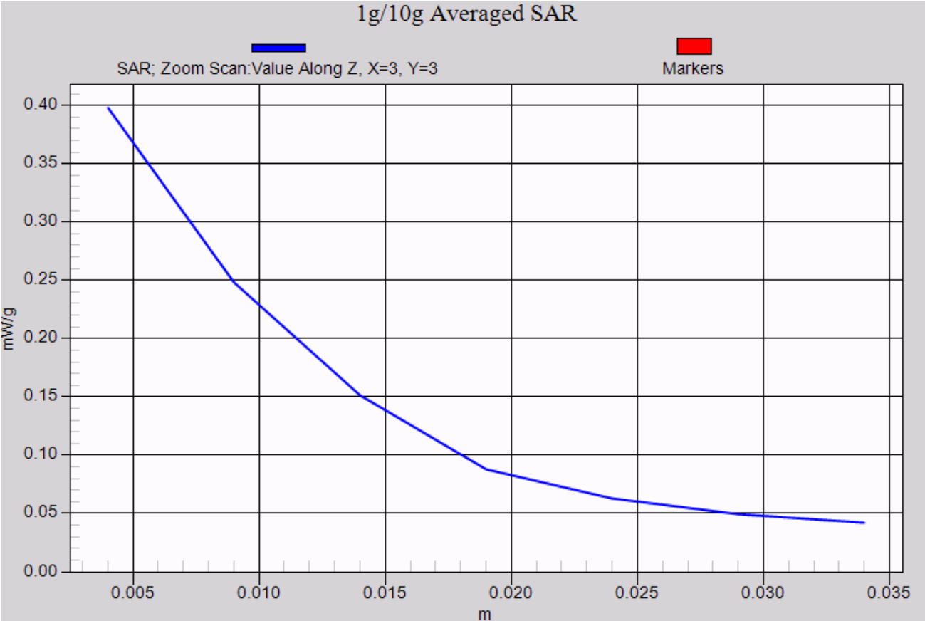
U1250 towards ground-GSM1900 GPRS 2TS Channel 810
