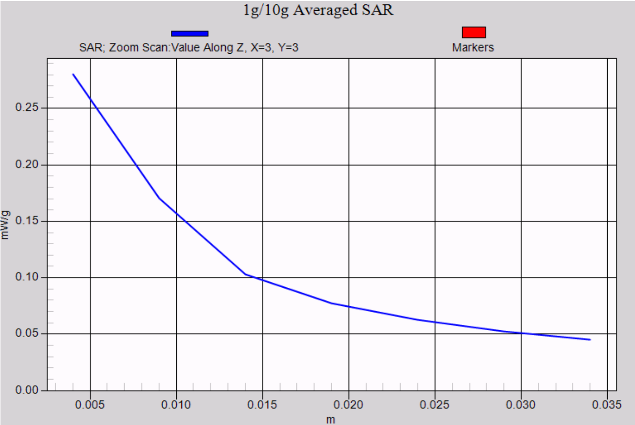
U1280 towards ground-GSM1900 GPRS 2TS Channel 512
