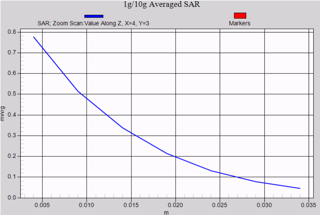
U1250 RightHandSide touched-GSM1900 Channel 810
