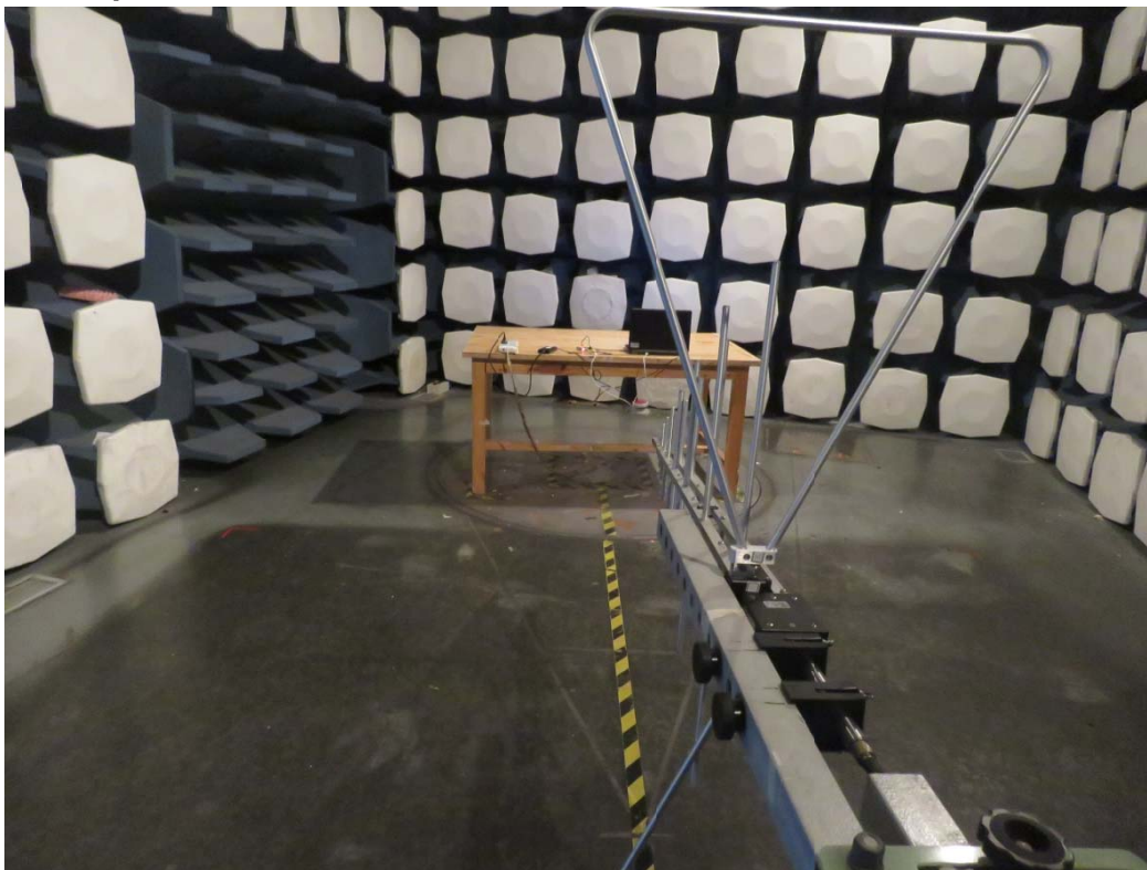
30M Hz-1GHz
