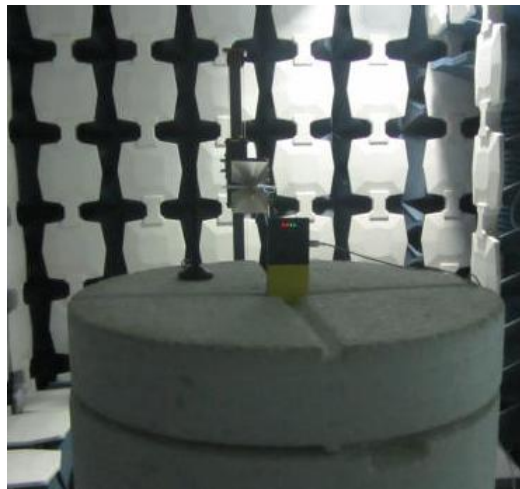
Radiated Spurious Emission (3GHz to18GHz)
