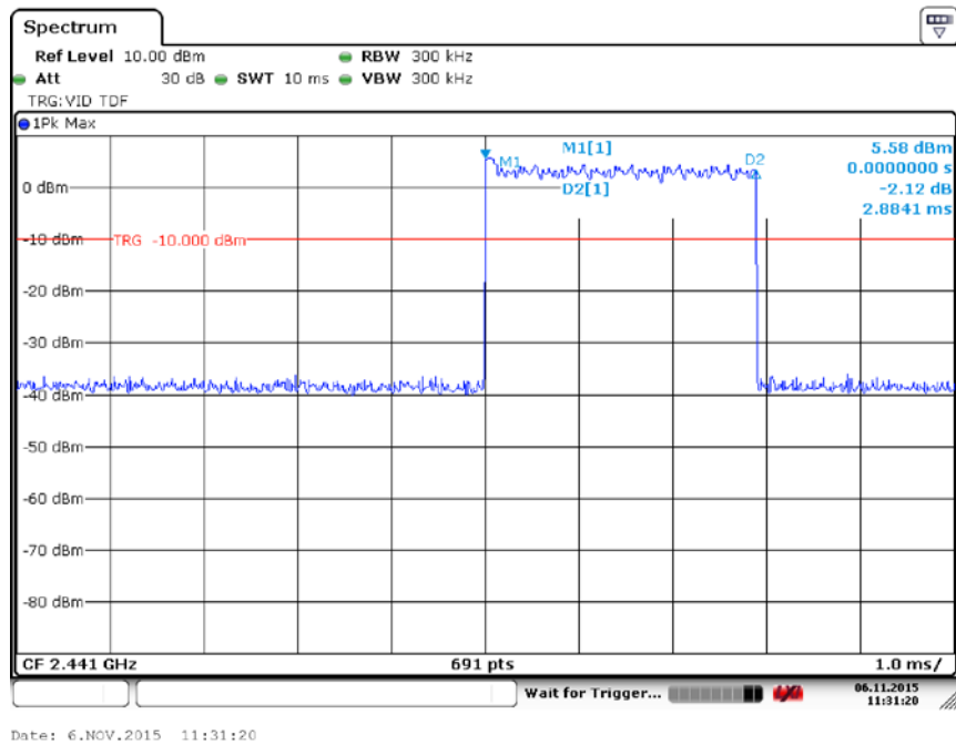
Fig. 85 Time of Occupancy(Dwell Time) (8DPSK, Ch39)
