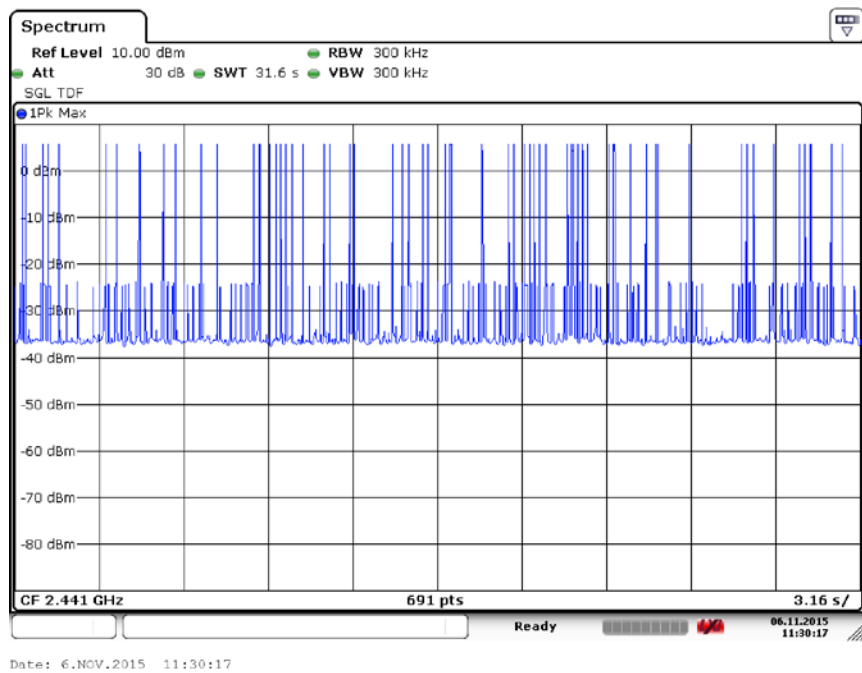
Fig. 86 Number of Transmissions (8DPSK, Ch39)
