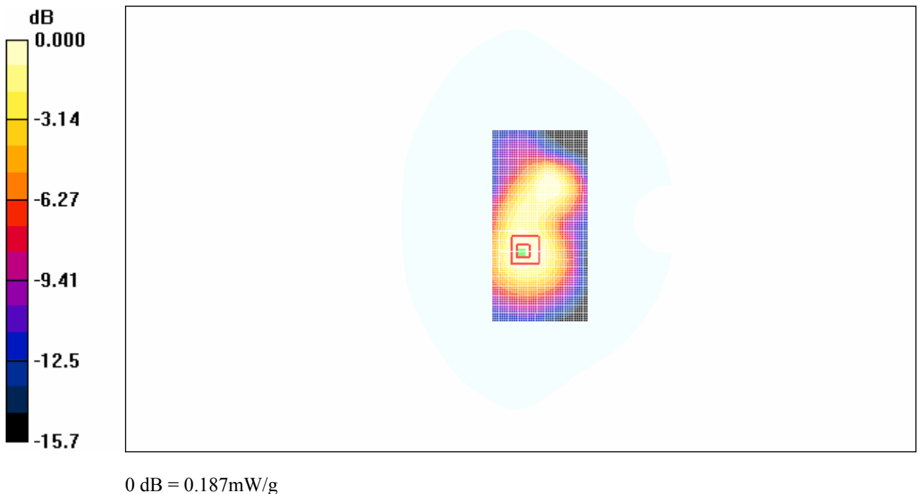
Fig. 151 PCS 1900MHz, Body, Towards Ground with Bluetooth, CH512
