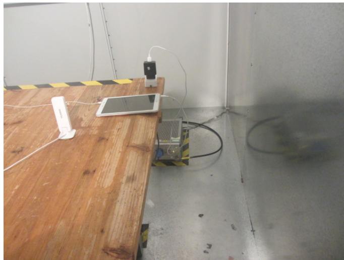
Conducted Emissions for AC Ports
