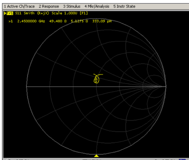
Impedance Test-Body
