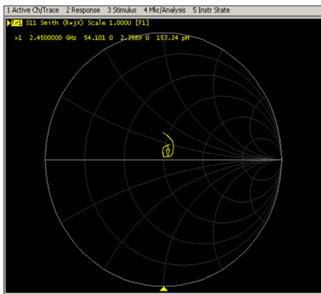
Impedance Test-Body
