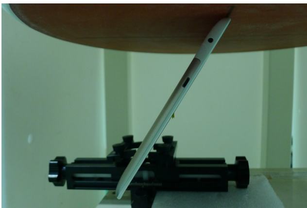
Curved surface of Edge1 at 30 Degree, Test Separation 0 cm
