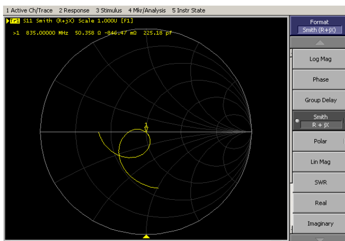
Impedance Test-Body
