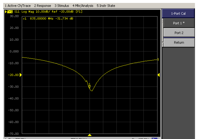
Return Loss Test-Body
