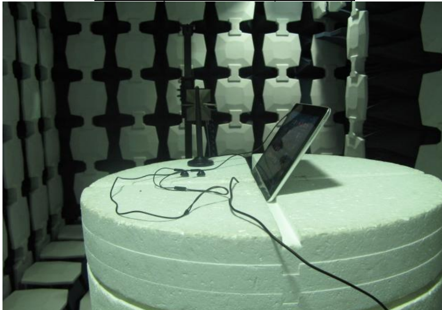
Radiated Spurious Emission (3GHz to18GHz)
