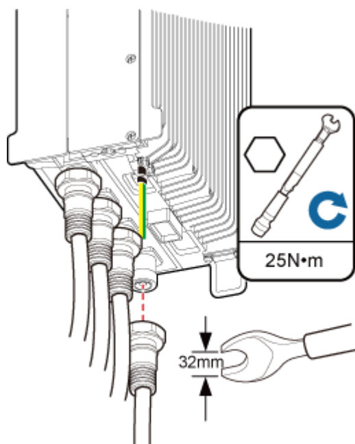
Figure 9-15 Installing an RRU RF jumper
