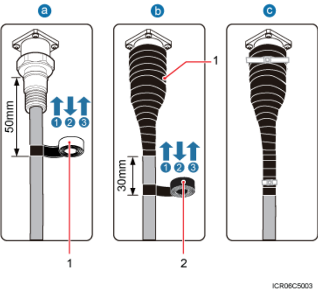
Figure 9-16 Waterproofing a connector of the RF jumper
