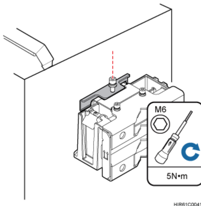
Figure 8-28 Securing the captive screw into the connection hole
