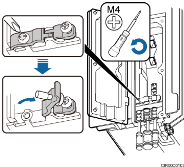
Figure 9-24 Opening clips
