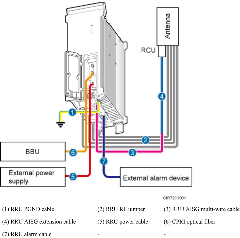
Figure 9-8 Cable connections of a single-mode RRU
