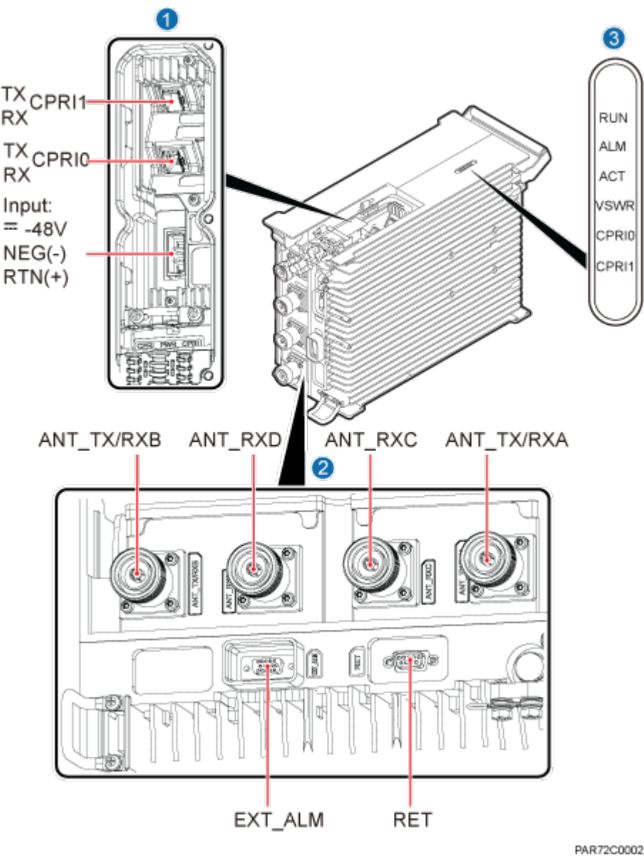
Figure 3-4 Ports on the RRU panels
