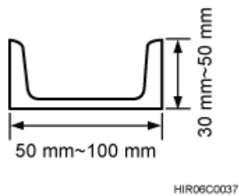
Figure 3-13 U-steel specifications
