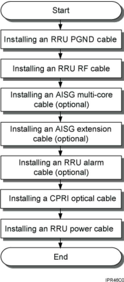
Figure 9-12 Procedure for installing RRU cables
