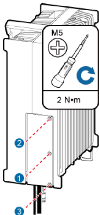
Figure 9-30 Closing the cover plate of an RRU cabling cavity
