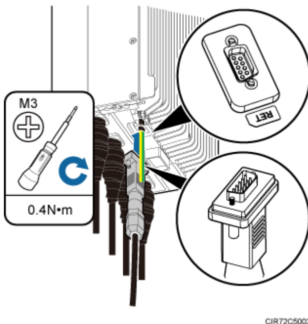
Figure 9-18 Installing an RRU AISG multi-wire cable
