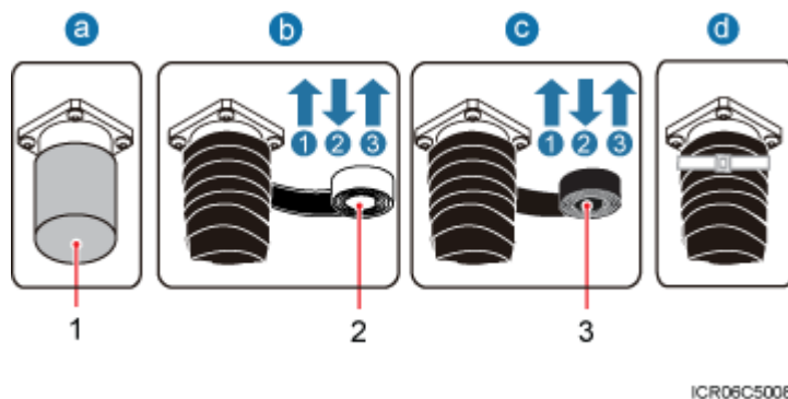
Figure 9-17 Waterproofing a dustproof cap
