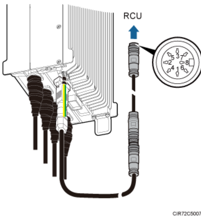
Figure 9-20 Installing an RRU AISG extension cable
