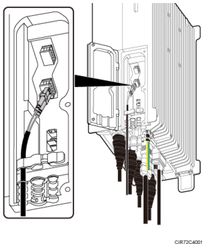
Figure 9-26 Installing a CPRI optical cable
