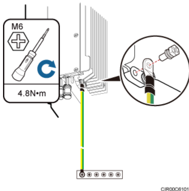
Figure 9-13 Installing an RRU PGND cable
