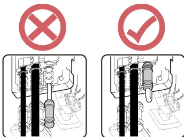
Figure 9-29 Correct placement of waterproof blocks
