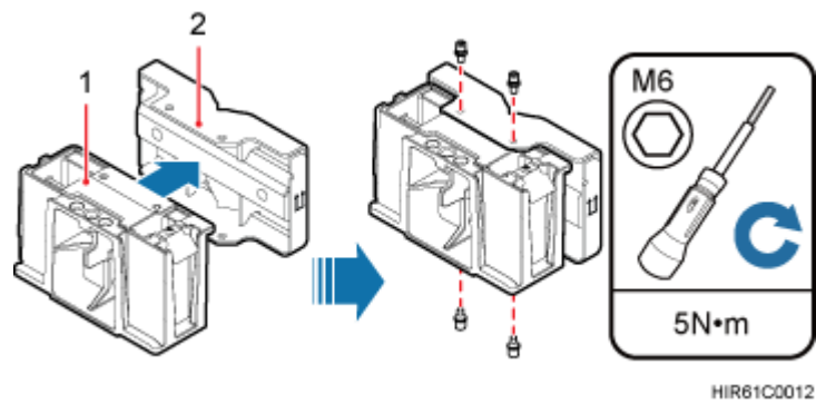
Figure 8-46 Installing the main bracket
