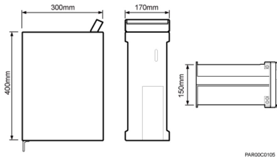
Figure 3-2 RRU dimensions
