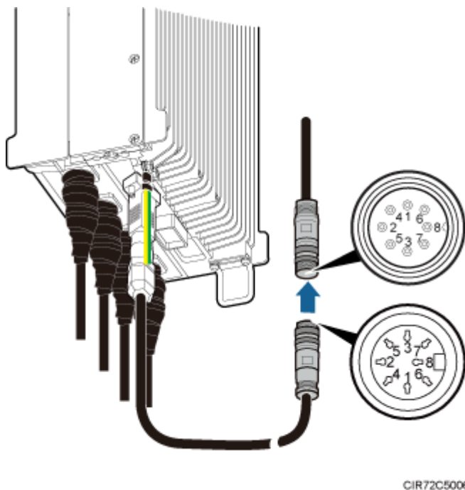
Figure 9-19 Installing an RRU AISG multi-wire cable
