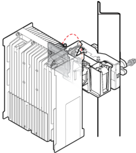
Figure 8-34 Installing the RRU onto the main bracket
