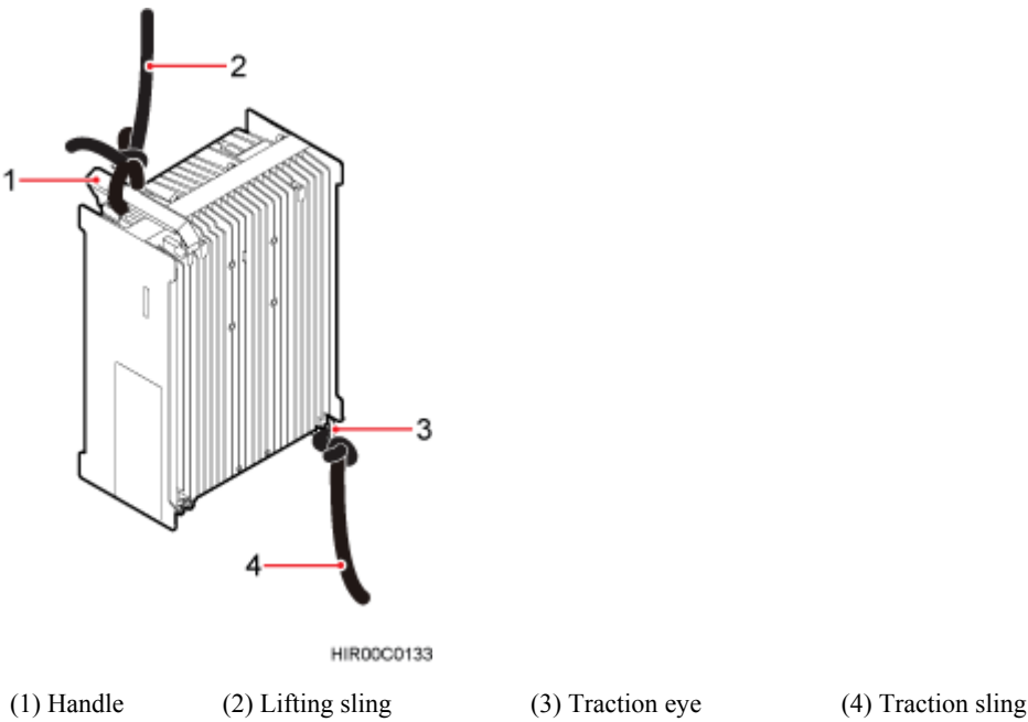
Figure 7-2 Binding the RRU
