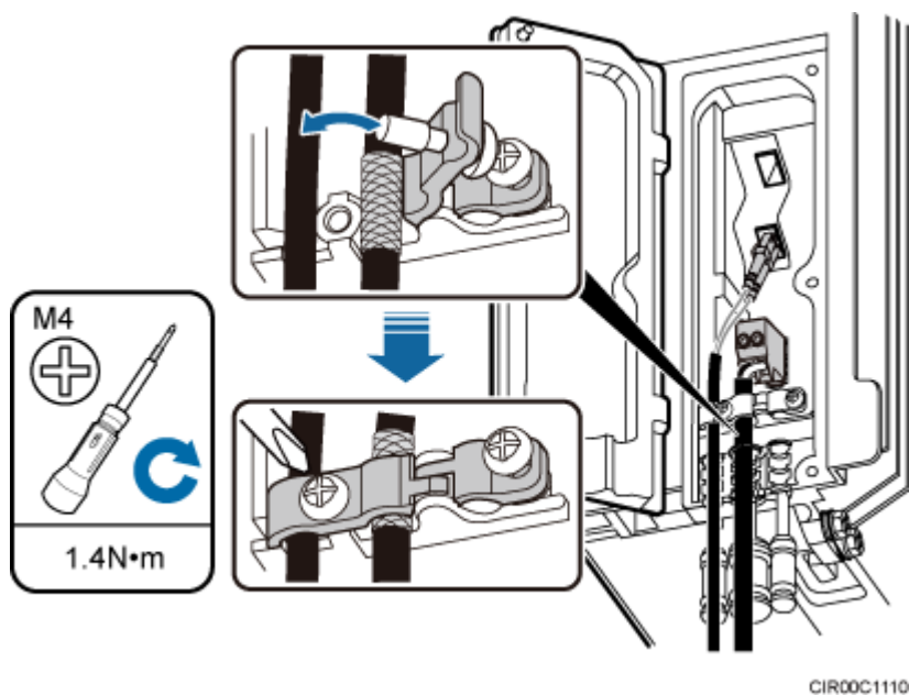
Figure 9-28 Closing clips
