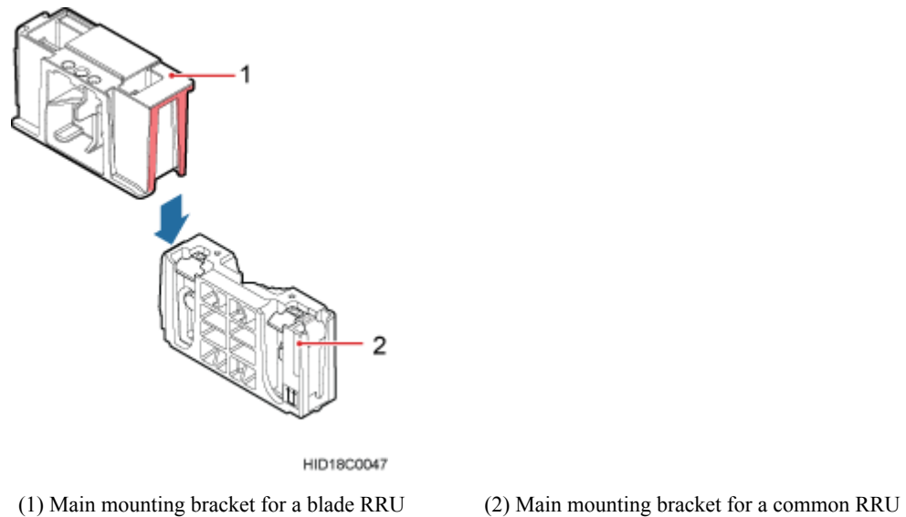
Figure 8-11 Connect to the main mounting bracket for installing a common RRU
