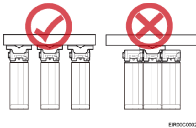
Figure 3-19 Correct installation of mounting brackets for RRUs installed on an IFS06
