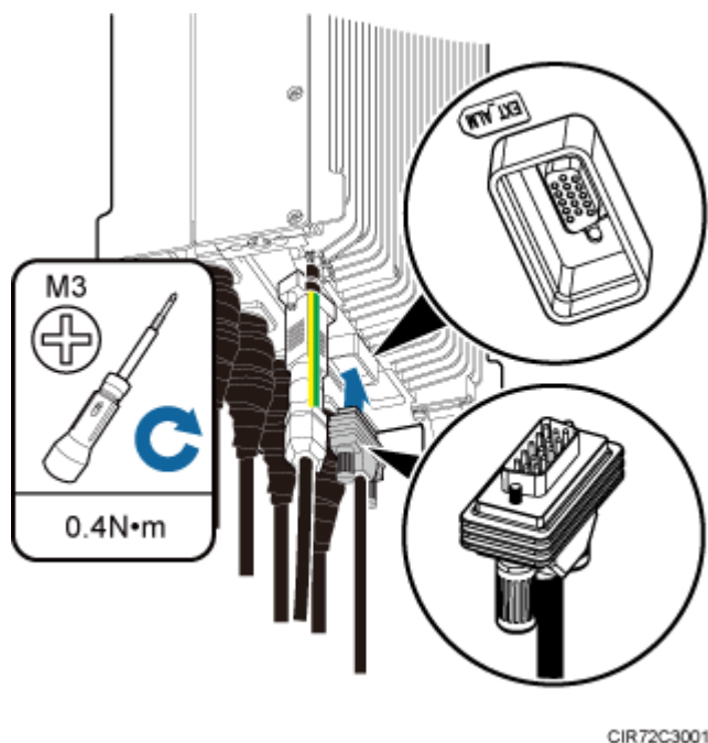
Figure 9-21 Installing an RRU alarm cable
