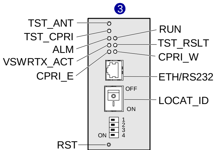
Maintenance cavity
