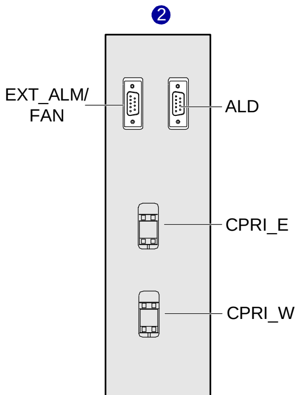
Cabling cavity
