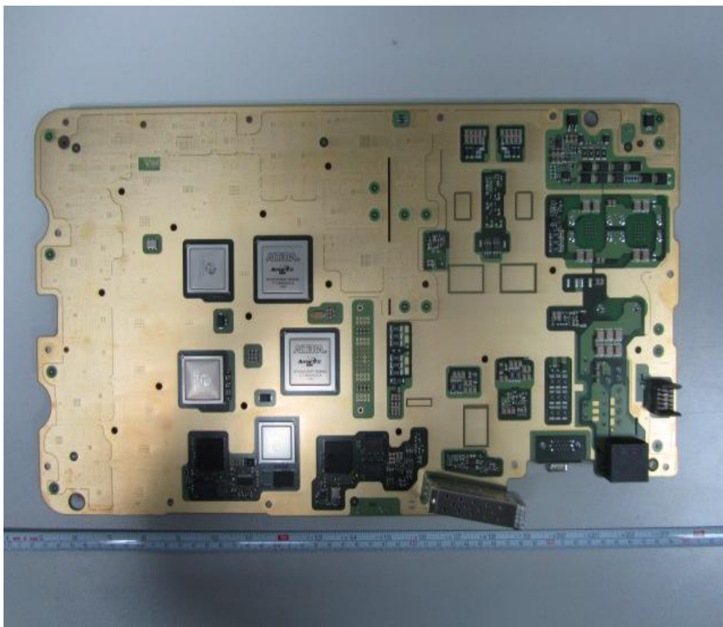
Photo-02 Internal View –BOTTOM
