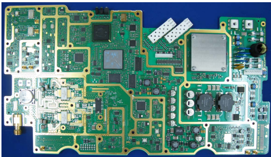
Figure 2, Top view of RRU3606 PCB
