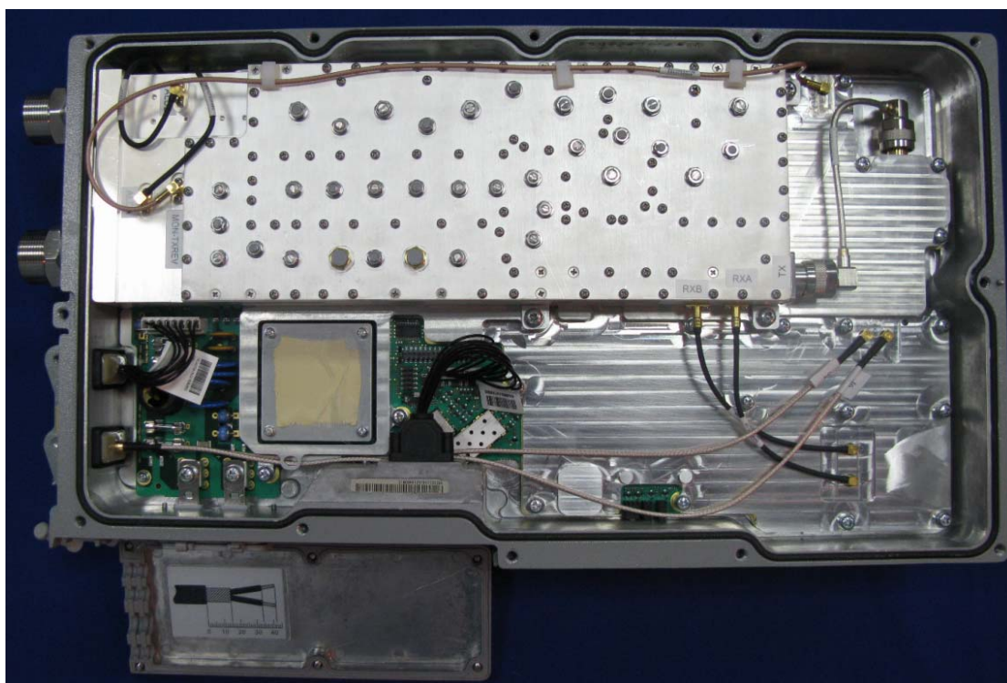
Figure 1, Internal view of RRU3606
