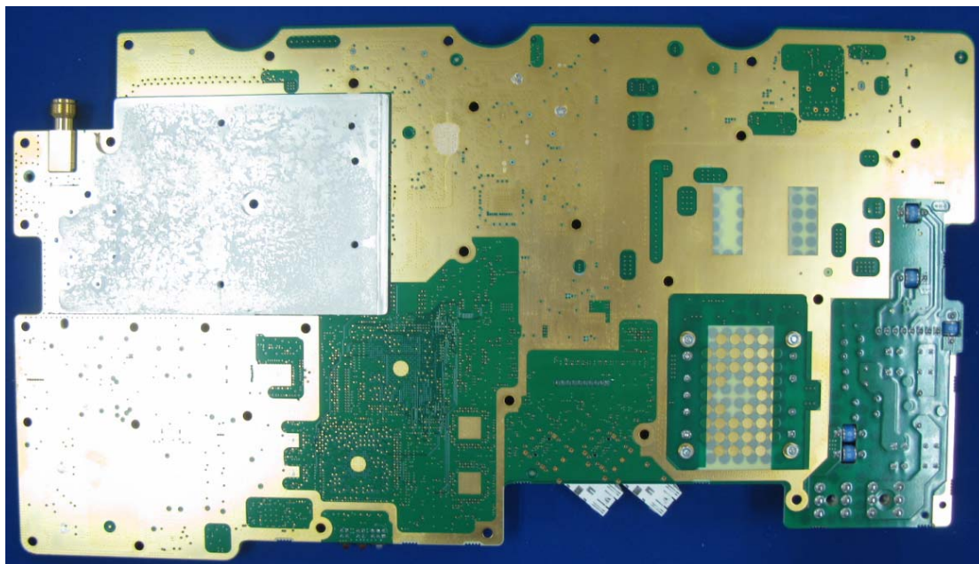
Figure 3, Bottom view of RRU3606 PCB
