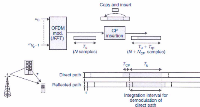
Figure 1-1 Cyclic-prefix insertion
