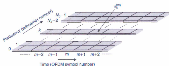
Figure 1-2 OFDM time-frequency grids
