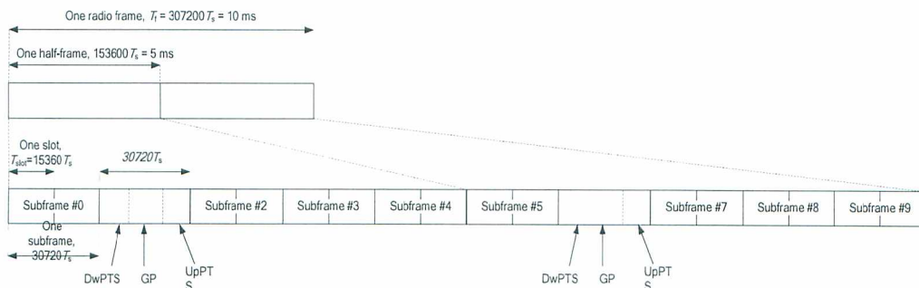
Figure 1-1 Frame structure type 2 (for 5 ms switch-point periodicity).
