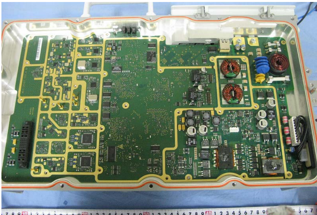
Photo-05 Internal Rear View –TRX
