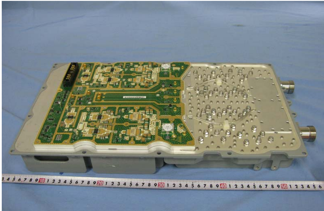
Photo-06 Internal Rear View –PA
