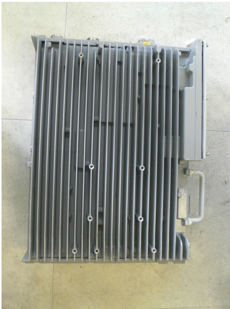
Figure 1-3 Another Side view of the RRU3008
