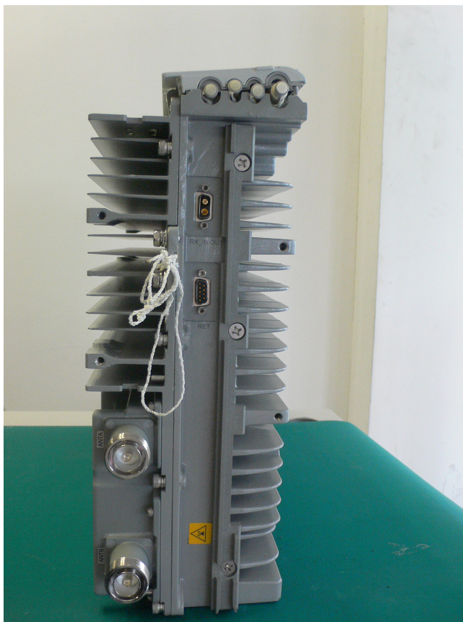
Figure 1-4 Rear view of the RRU3008
