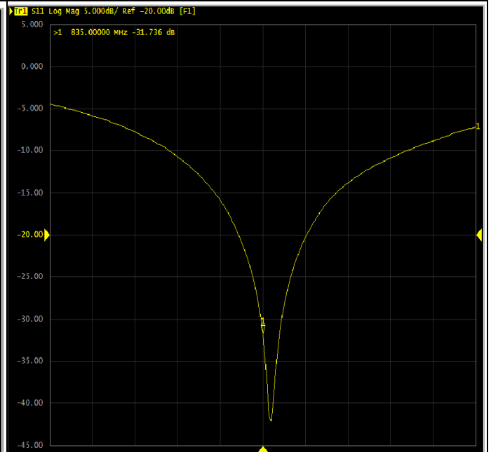
Return Loss Test-Head
