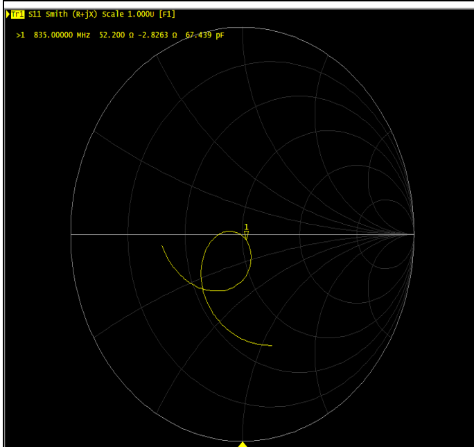
Impedance Test-Head
