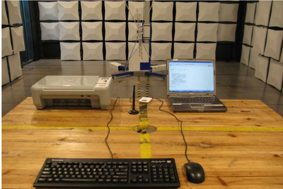
Radiated Disturbance (30MHz-1GHz)
