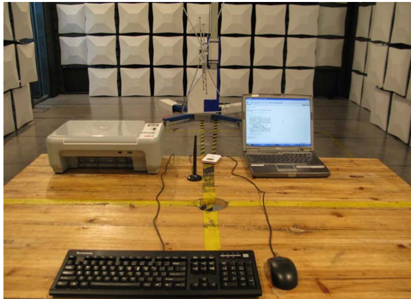
Radiated Spurious Emission (below 3GHz)
