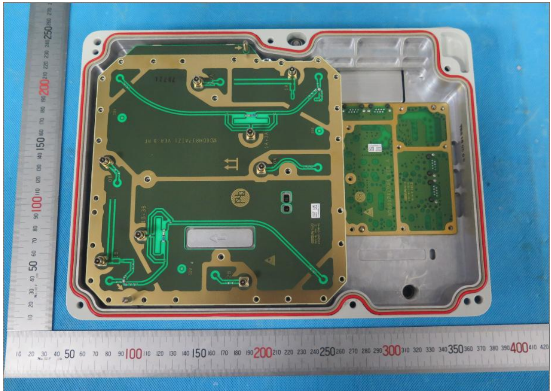
Photo-02 Internal View—takes apart the shielding
