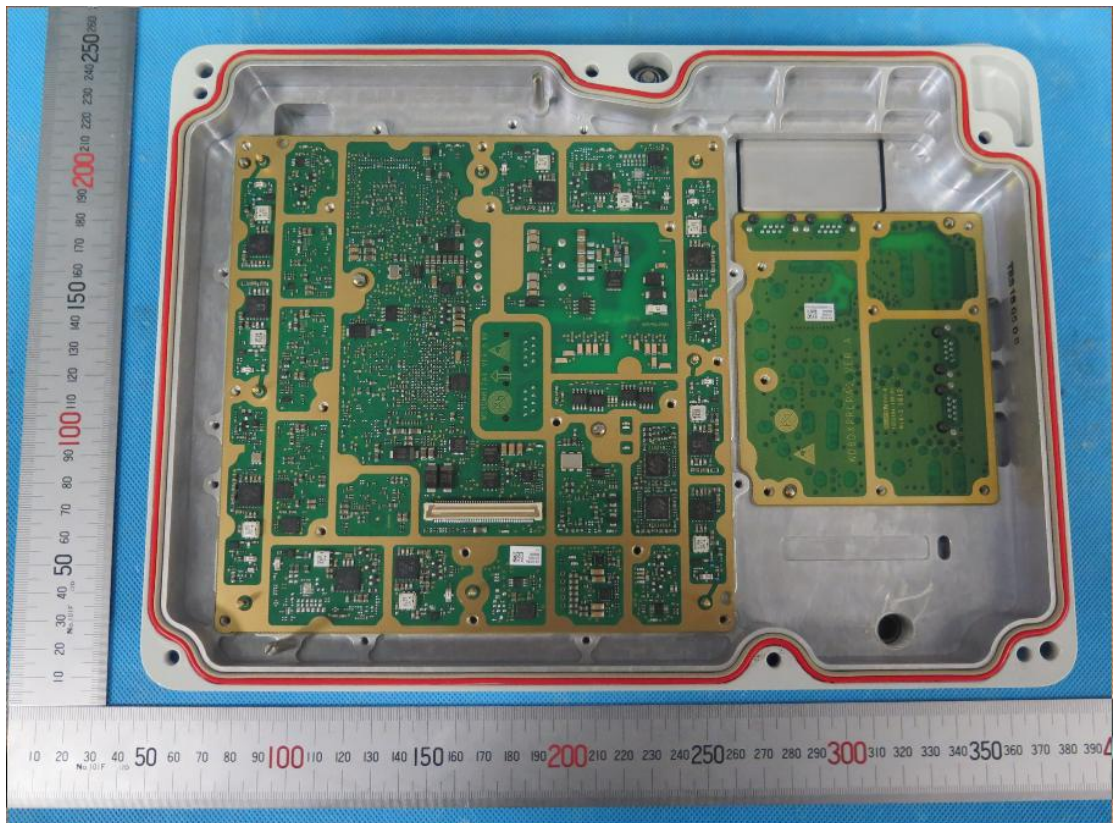
Photo-03 Internal View—takes apart the WD6DMR17AIZ1 board
