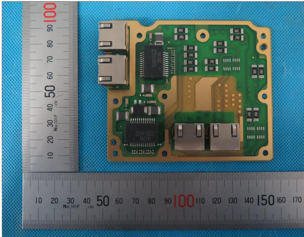
Photo-06 Heads of WD6DXPRLPA1
