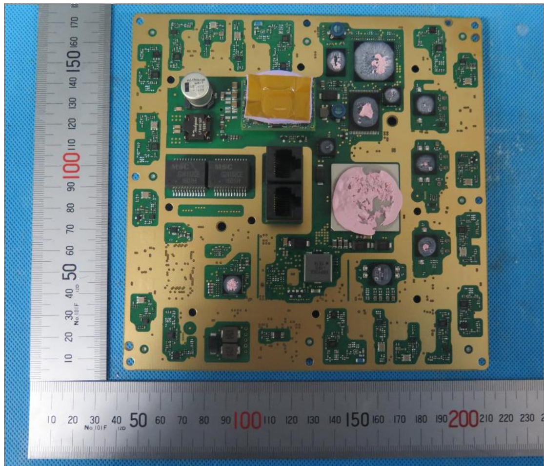
Photo-09 Rear of WD6DMR17AI
