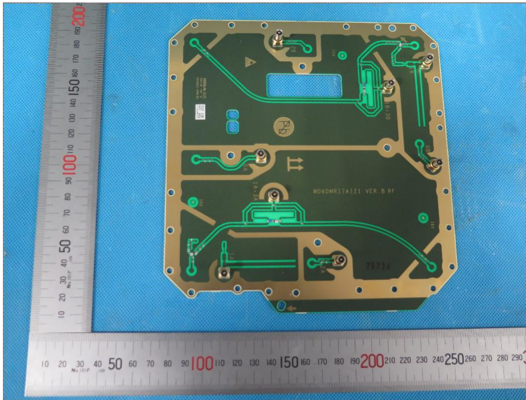
Photo-04 Heads of WD6DMRI7AIZ1
