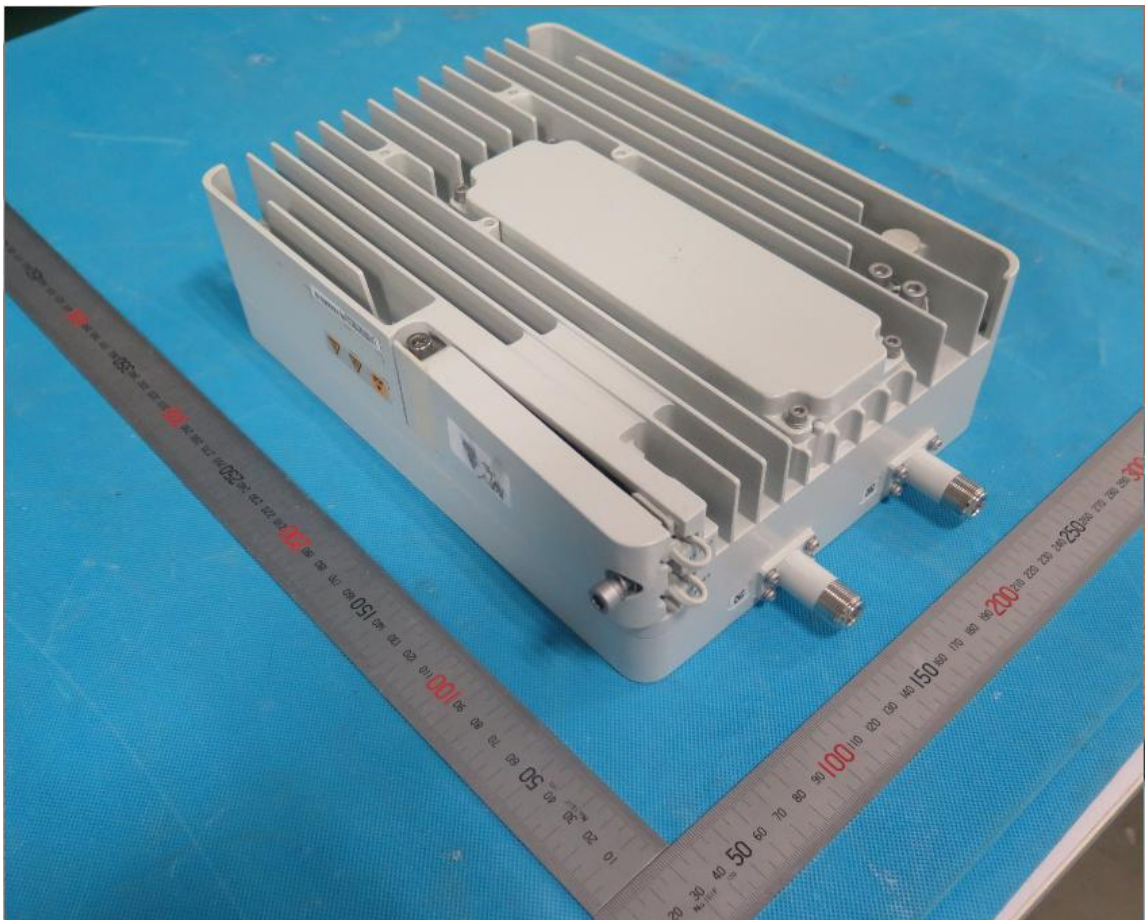
Photo-04 External View - Back
