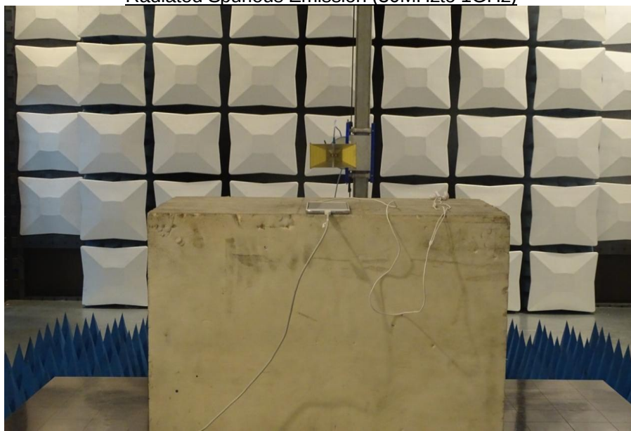
Radiated Spurious Emission (1GHz to18GHz)
